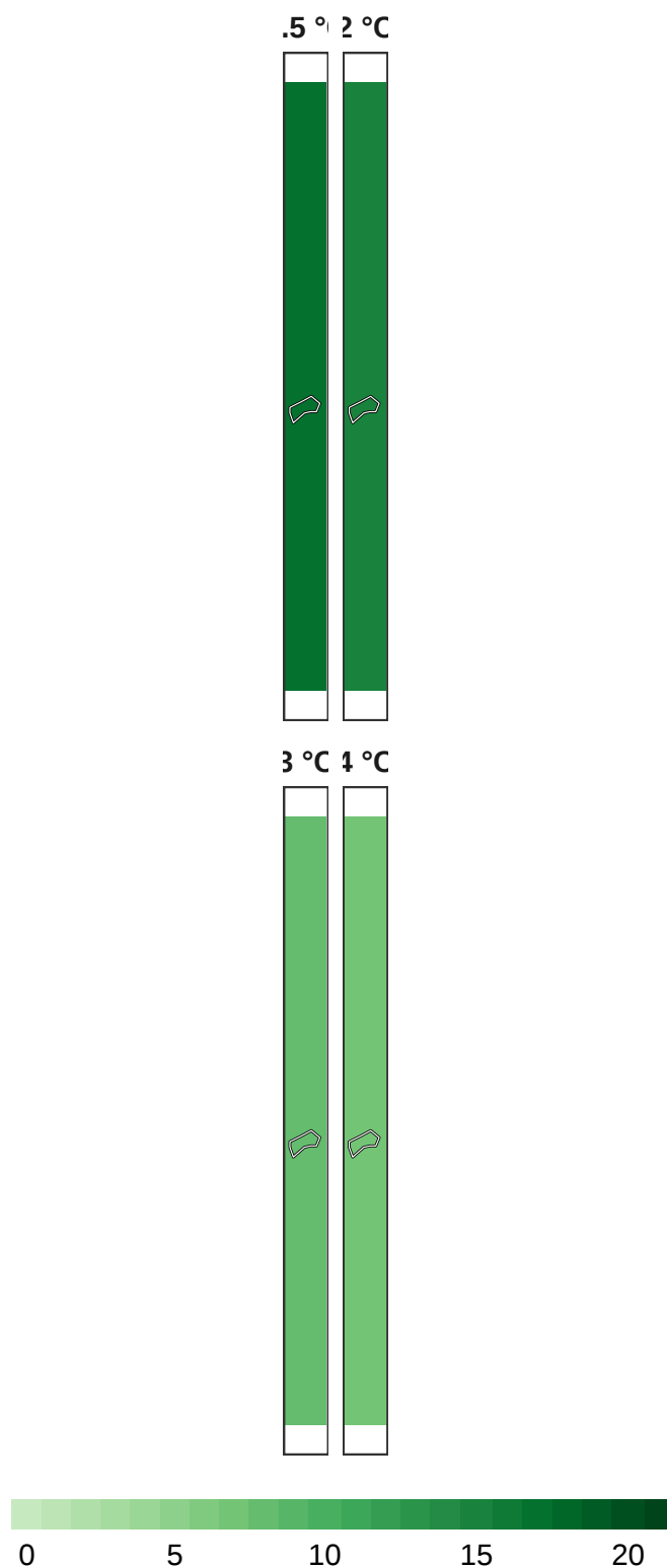
Figure 11: Number of models in agreement for reptile refugia at 1 km resolution.
