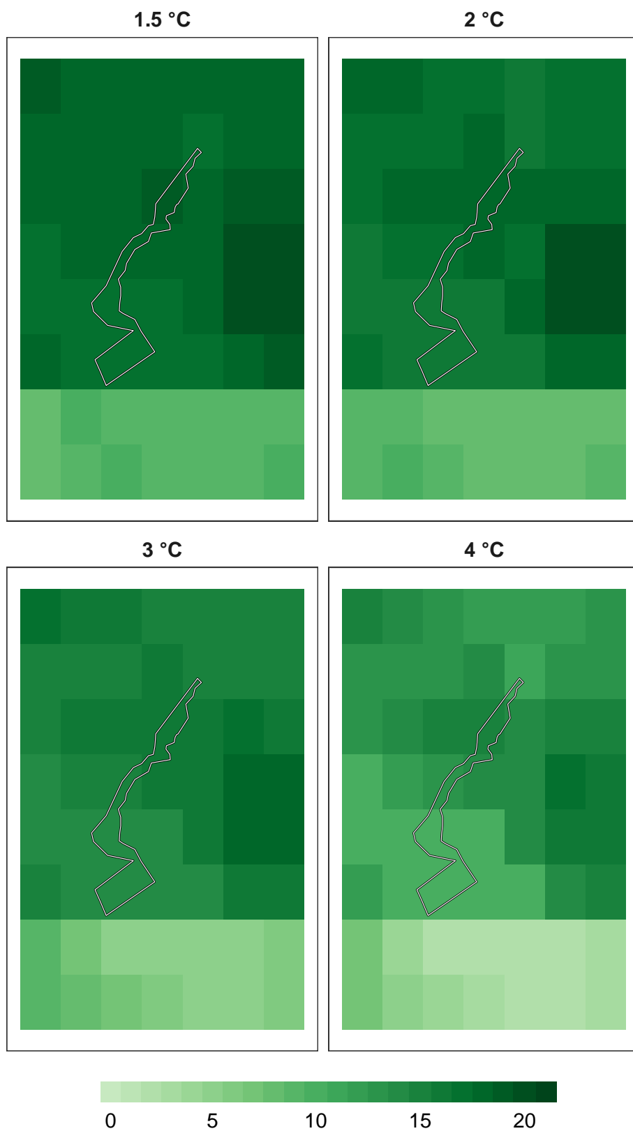
Figure 16: Number of models in agreement for pollinator refugia at 1 km resolution.
