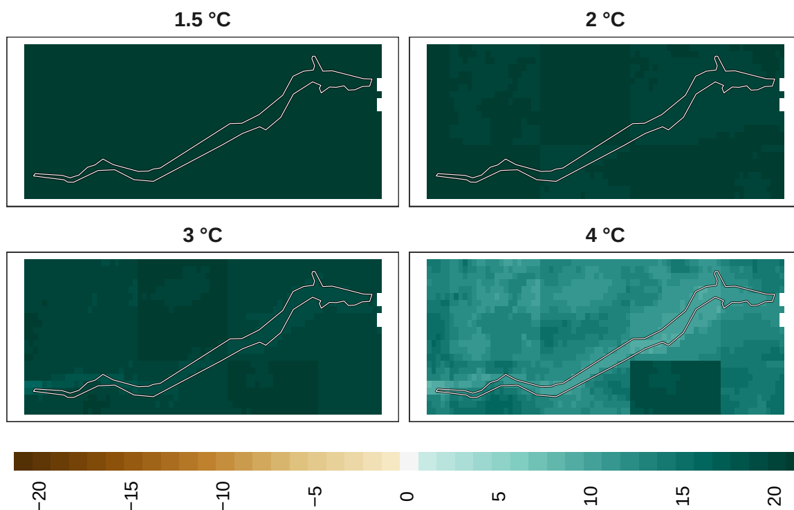
Figure 20: Adaptation effort for insects at 1 km resolution.
