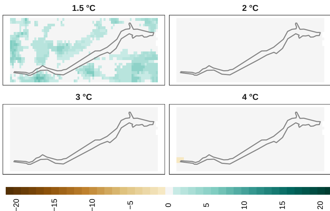
Figure 15: Adaptation effort for overall biodiversity at 1 km resolution.
