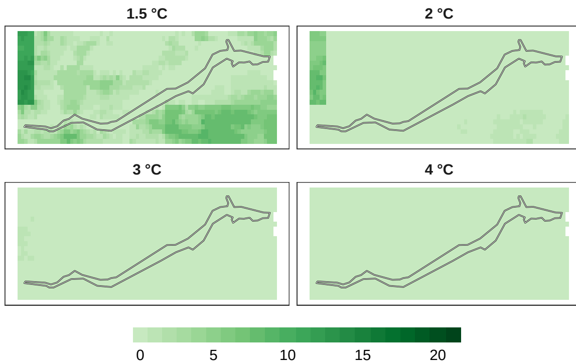
Figure 12: Number of models in agreement for reptile refugia at 1 km resolution.
