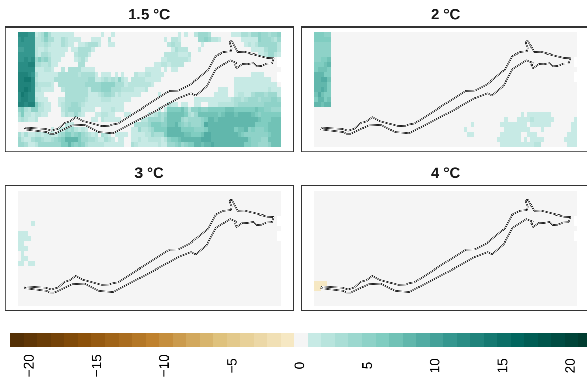
Figure 19: Adaptation effort for reptiles at 1 km resolution.
