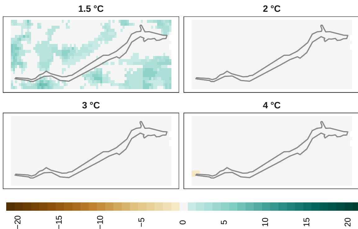
Figure 16: Adaptation effort for plants at 1 km resolution.
