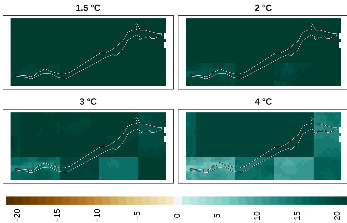
Figure 18: Adaptation effort for mammals at 1 km resolution.
