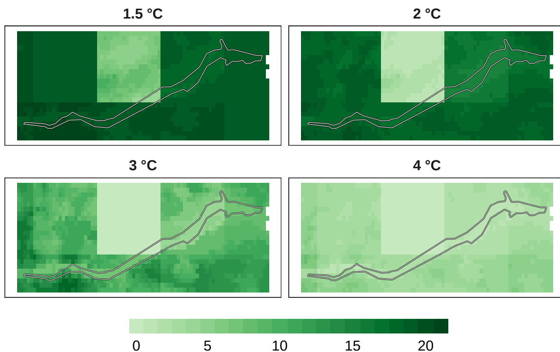
Figure 14: Number of models in agreement for pollinator refugia at 1 km resolution.
