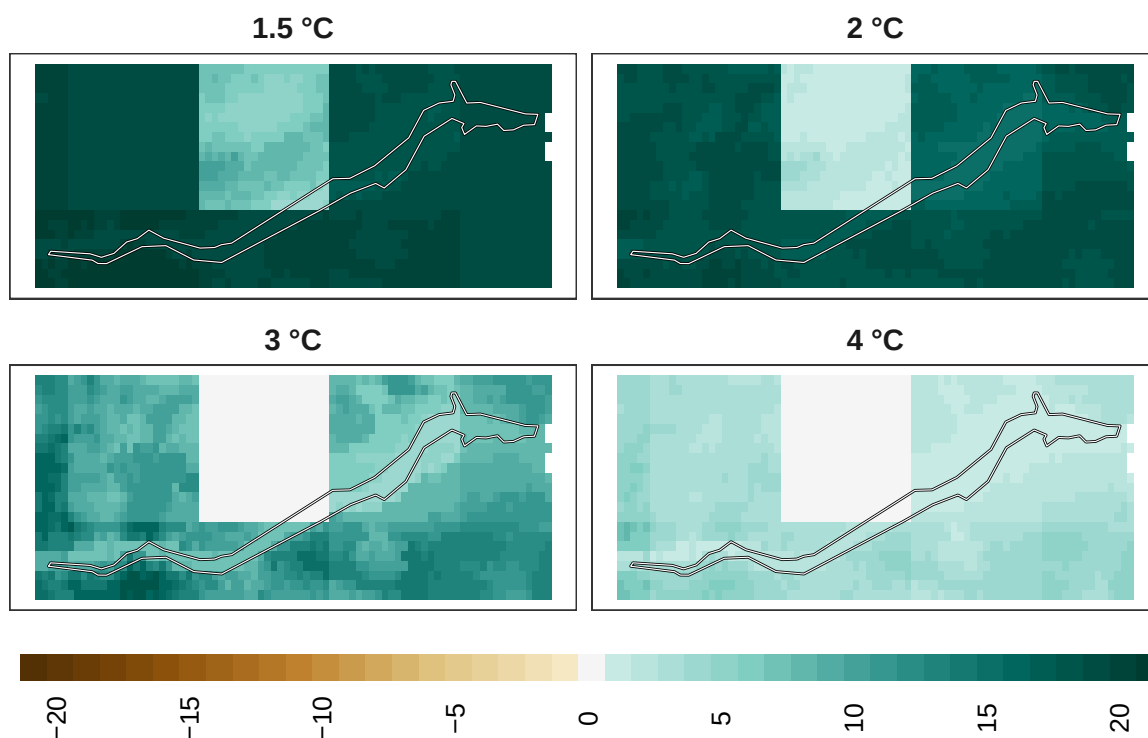
Figure 21: Adaptation effort for pollinators at 1 km resolution.
