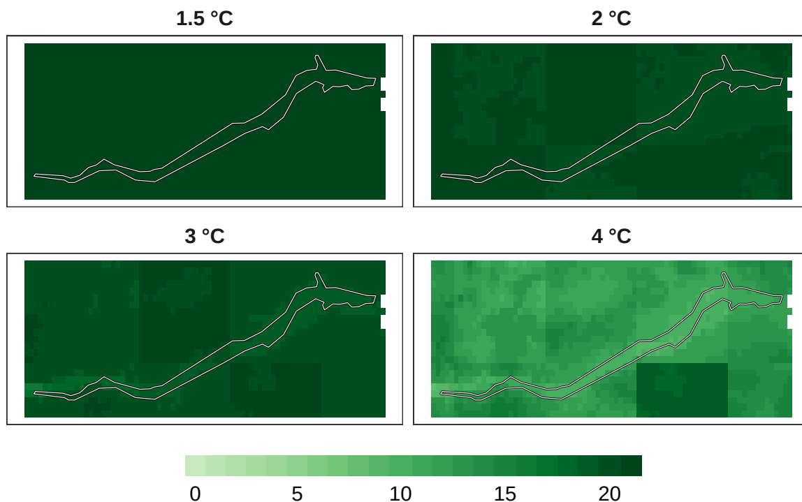
Figure 13: Number of models in agreement for insect refugia at 1 km resolution.
