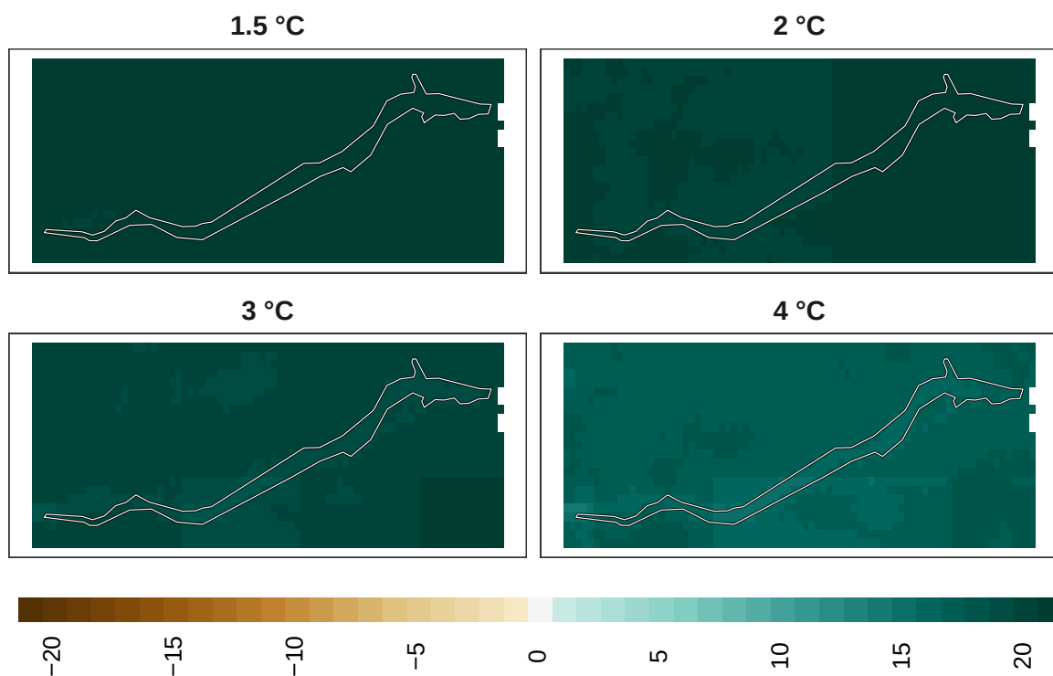
Figure 17: Adaptation effort for birds at 1 km resolution.
