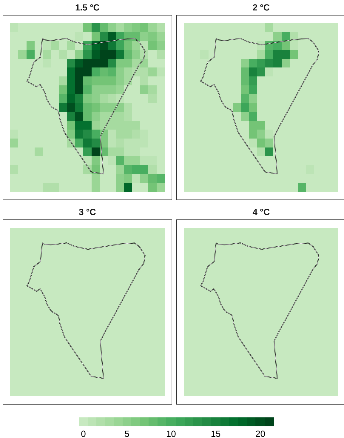
Figure 15: Number of models in agreement for insect refugia at 1 km resolution.
