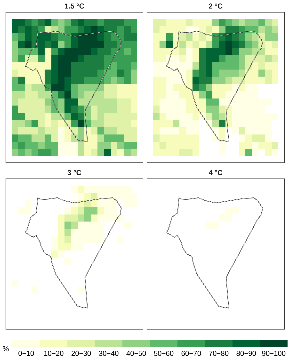
Figure 3: Percent amphibians remaining at 1 km resolution.
