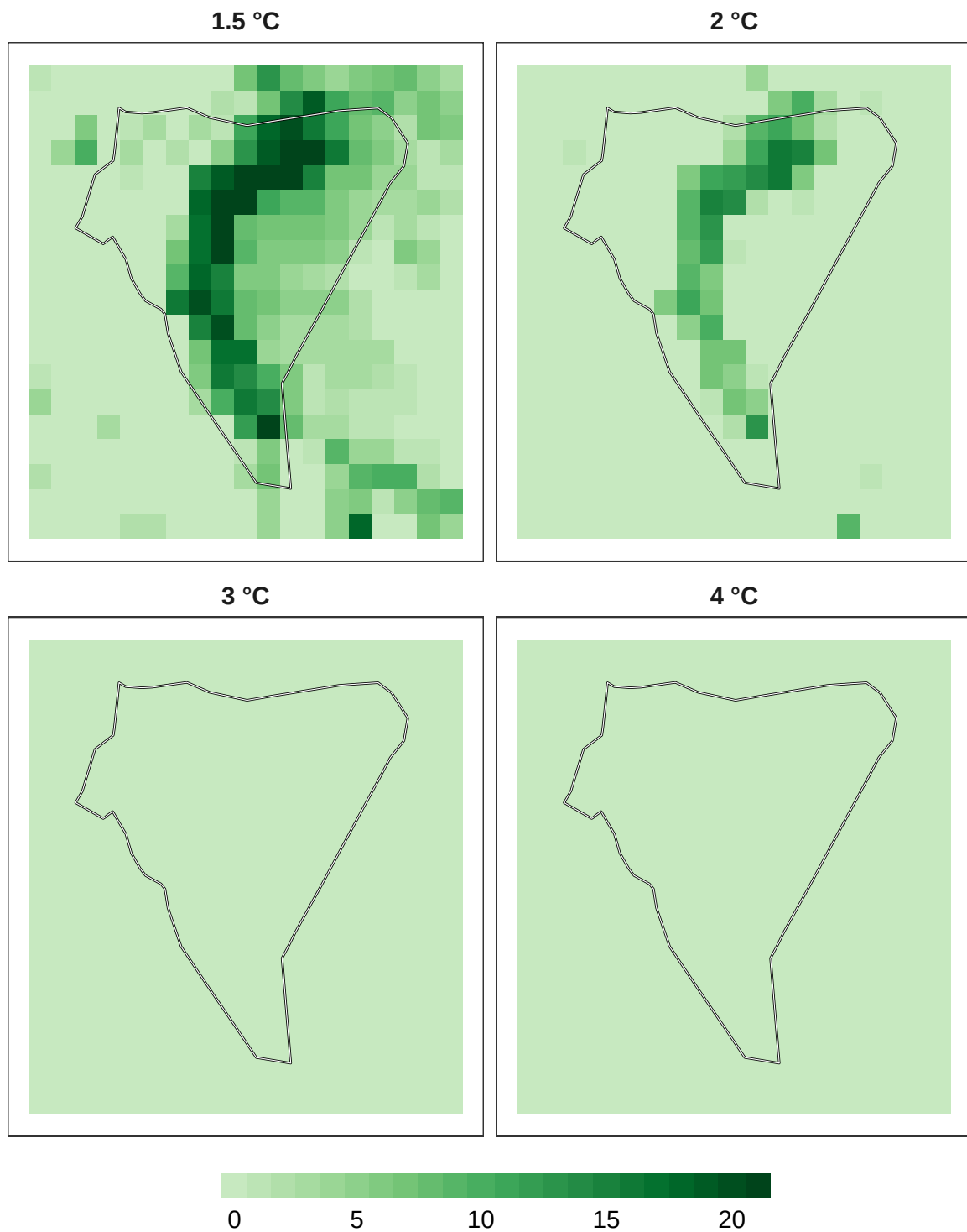
Figure 14: Number of models in agreement for reptile refugia at 1 km resolution.
