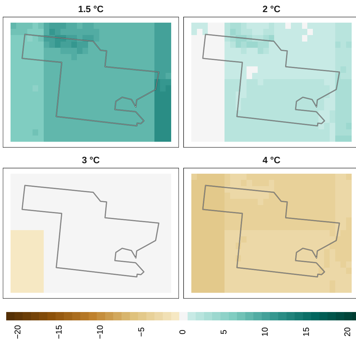
Figure 22: Adaptation effort for insects at 1 km resolution.
