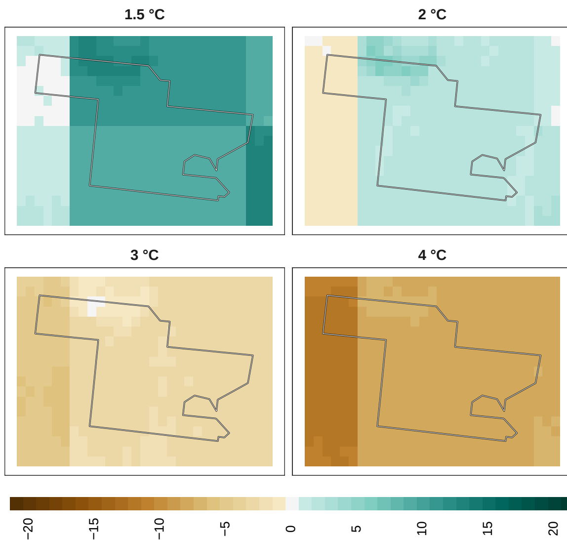
Figure 17: Adaptation effort for plants at 1 km resolution.
