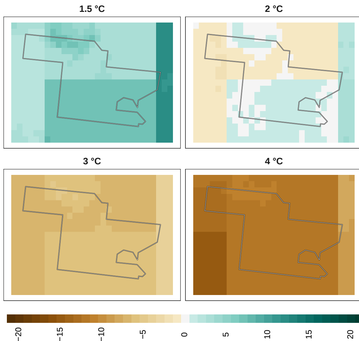
Figure 21: Adaptation effort for reptiles at 1 km resolution.
