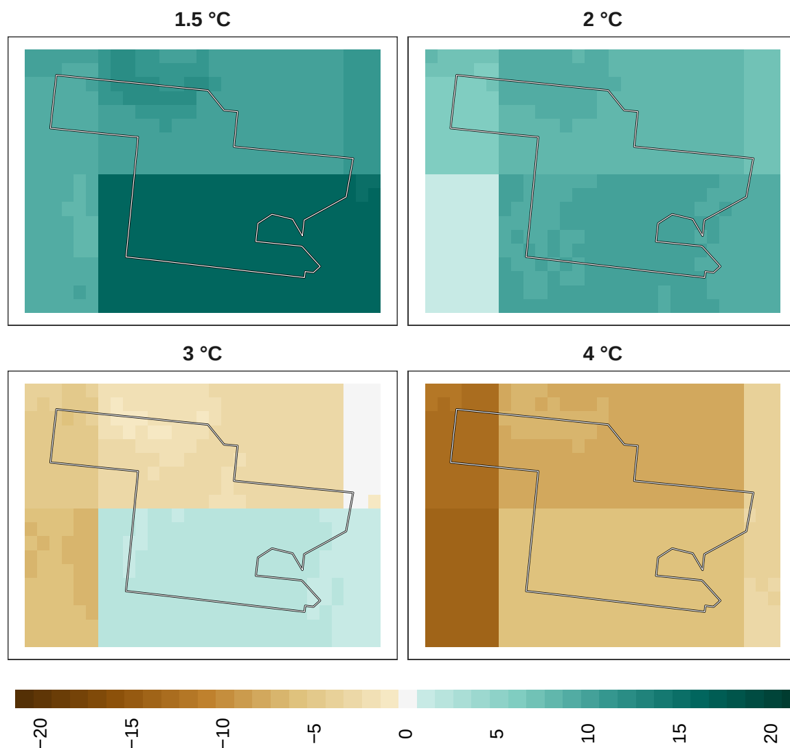
Figure 18: Adaptation effort for amphibians at 1 km resolution.
