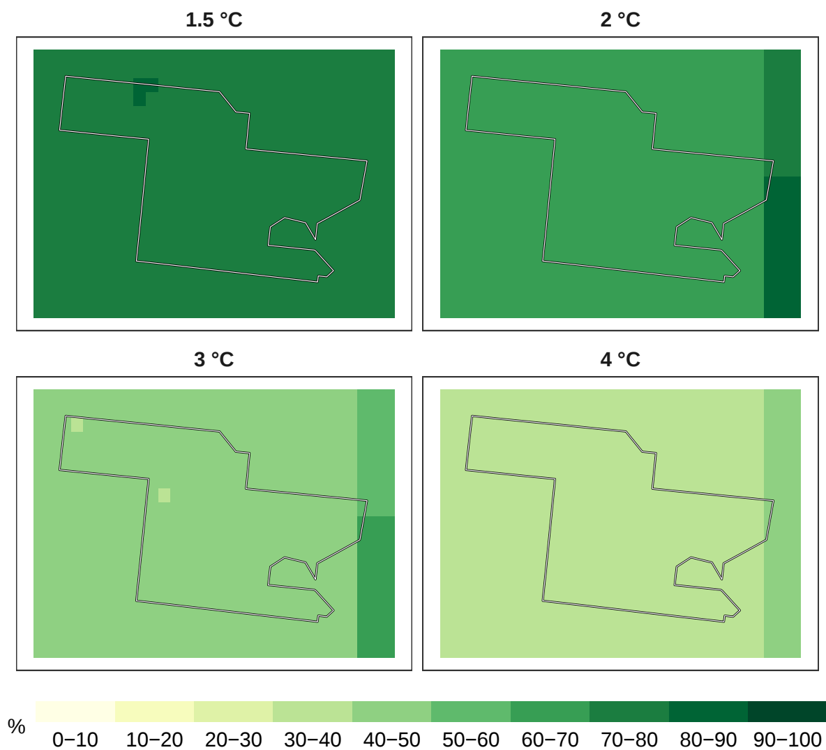
Figure 8: Percent timber species remaining at 1 km resolution.
