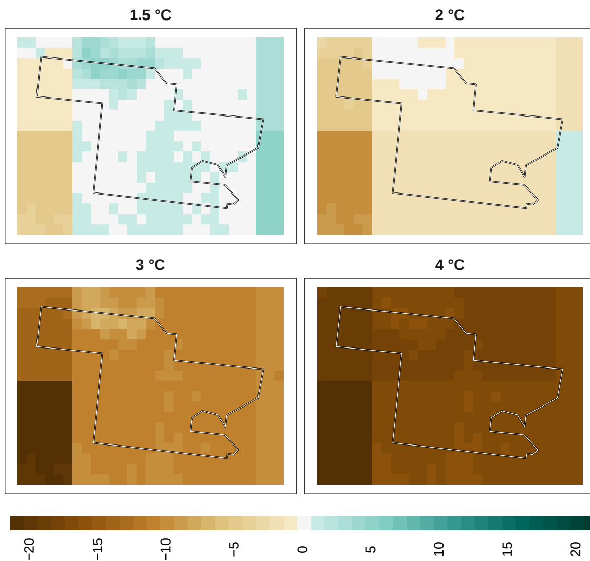
Figure 20: Adaptation effort for mammals at 1 km resolution.
