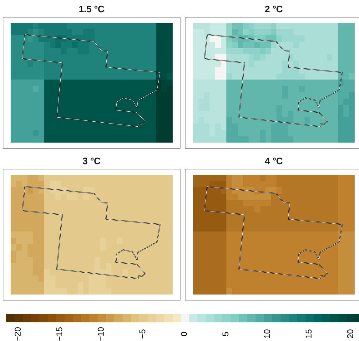
Figure 19: Adaptation effort for birds at 1 km resolution.
