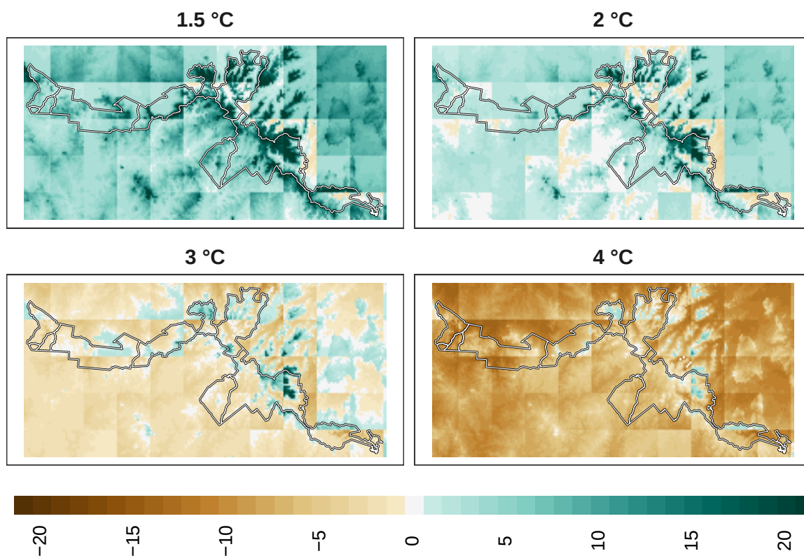
Figure 21: Adaptation effort for birds at 1 km resolution.
