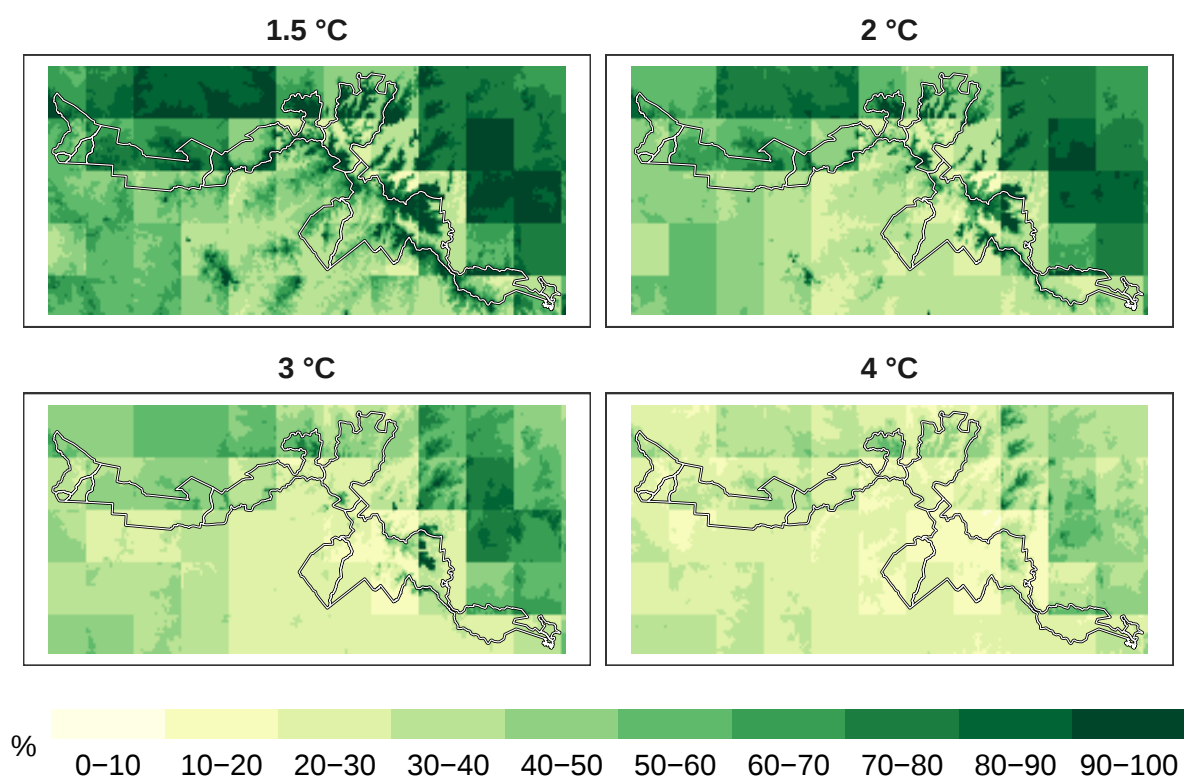
Figure 5: Percent mammals remaining at 1 km resolution.
