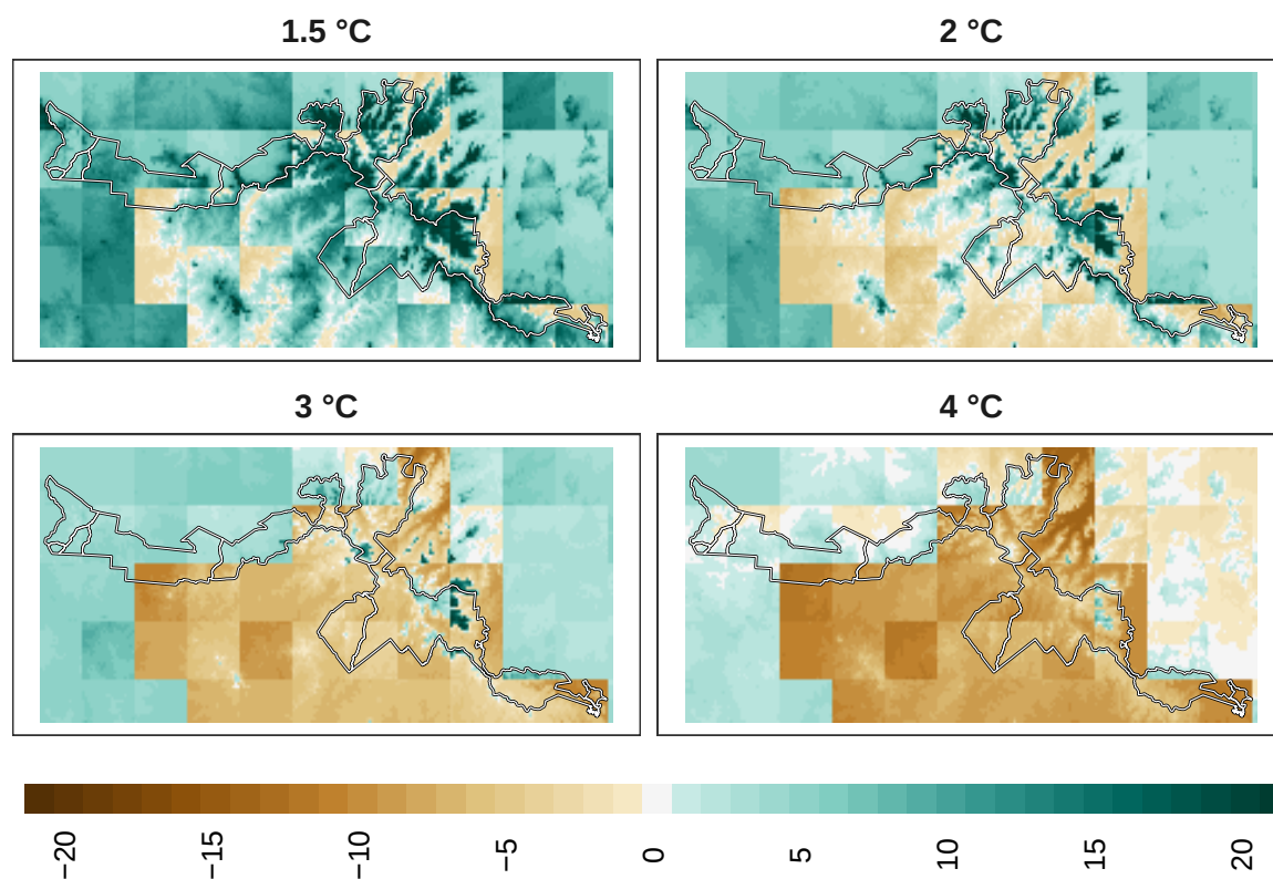
Figure 25: Adaptation effort for pollinators at 1 km resolution.
