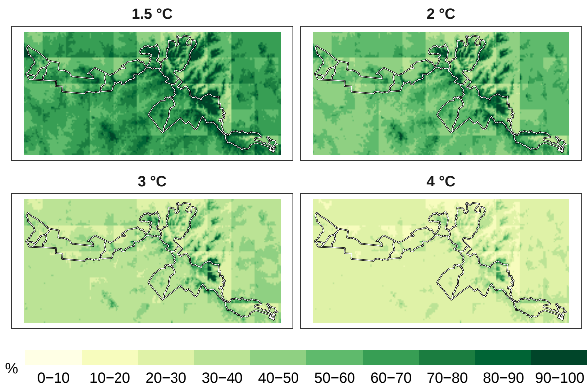
Figure 7: Percent insects remaining at 1 km resolution.
