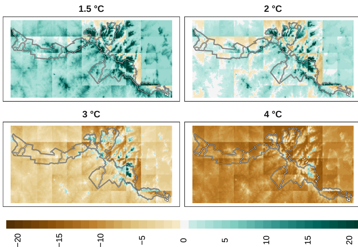
Figure 24: Adaptation effort for insects at 1 km resolution.
