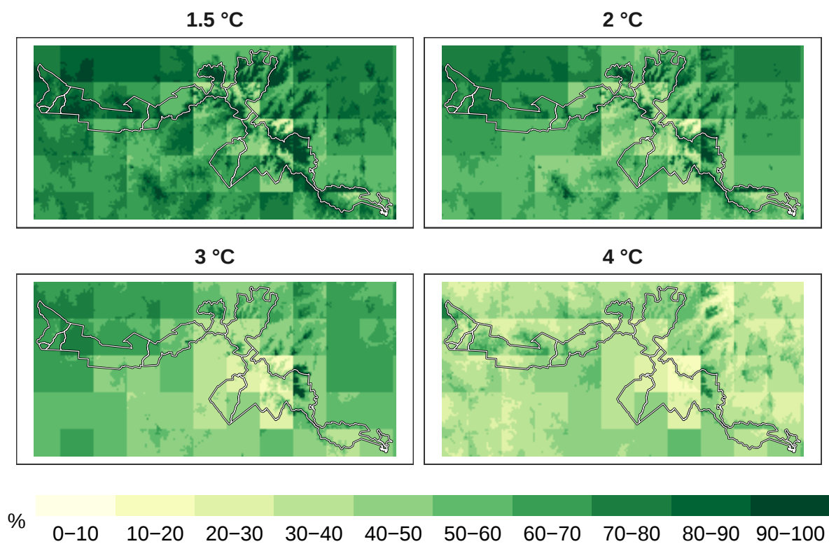
Figure 3: Percent amphibians remaining at 1 km resolution.
