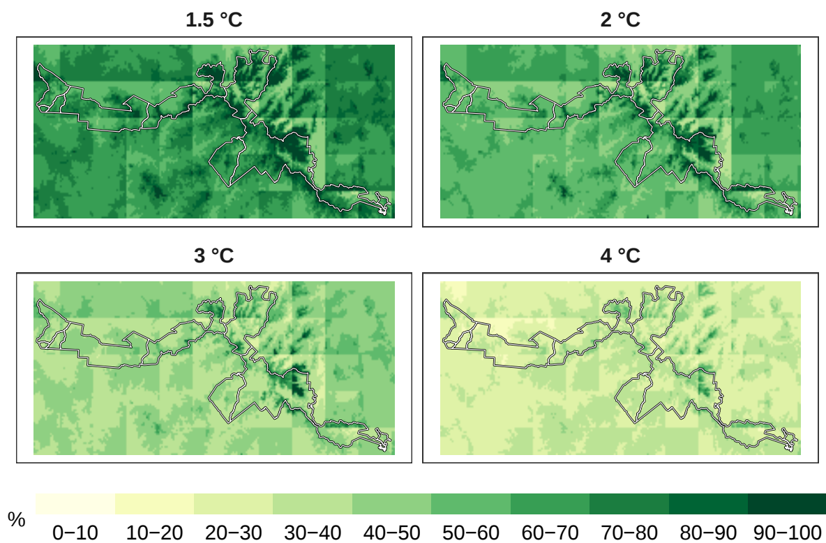
Figure 4: Percent birds remaining at 1 km resolution.
