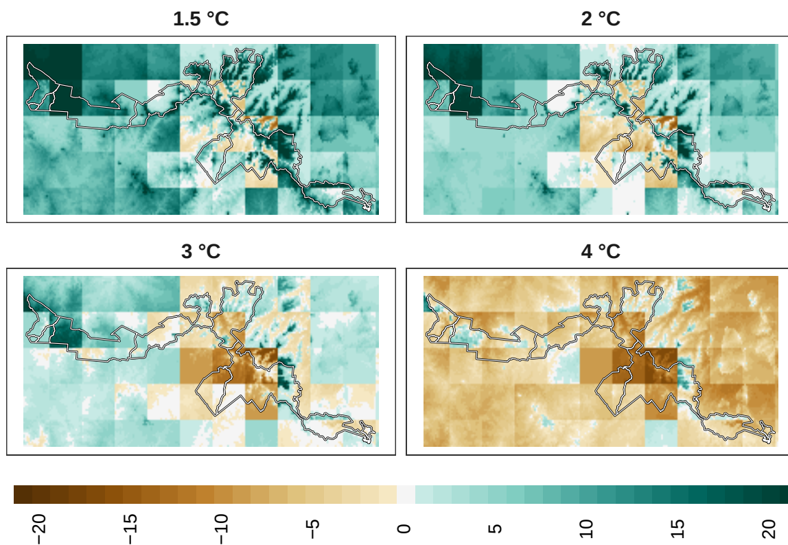
Figure 20: Adaptation effort for amphibians at 1 km resolution.
