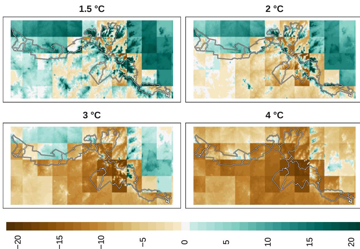
Figure 22: Adaptation effort for mammals at 1 km resolution.
