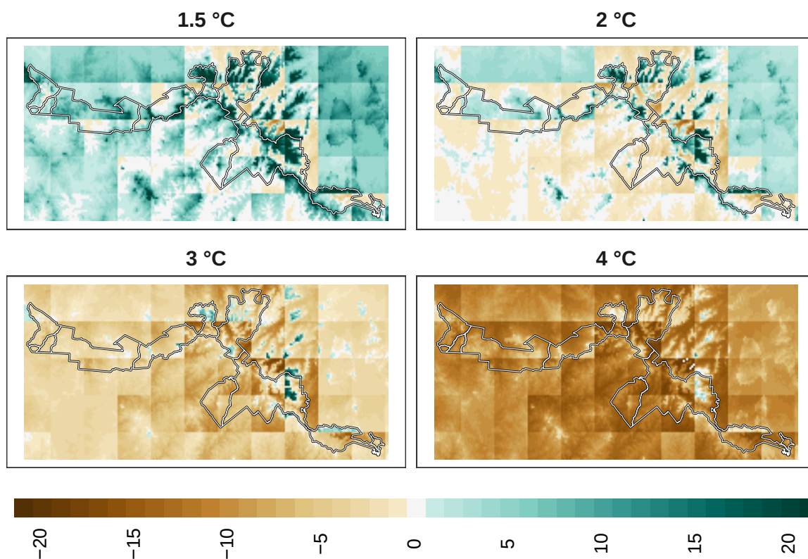
Figure 19: Adaptation effort for plants at 1 km resolution.
