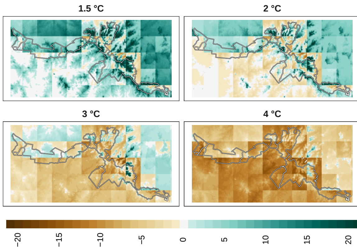
Figure 23: Adaptation effort for reptiles at 1 km resolution.
