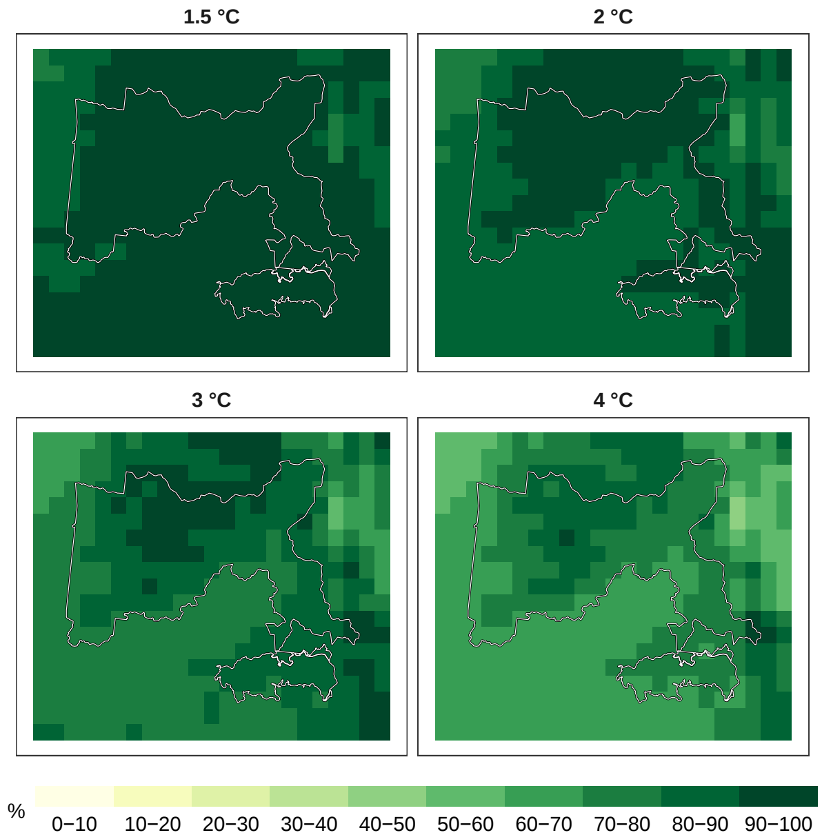
Figure 2: Percent plants remaining at 1 km resolution.
