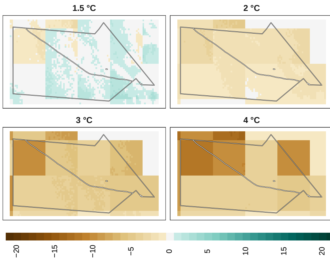
Figure 20: Adaptation effort for reptiles at 1 km resolution.
