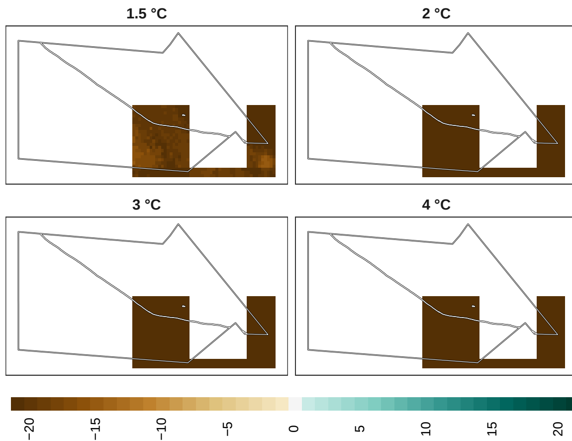
Figure 17: Adaptation effort for amphibians at 1 km resolution.
