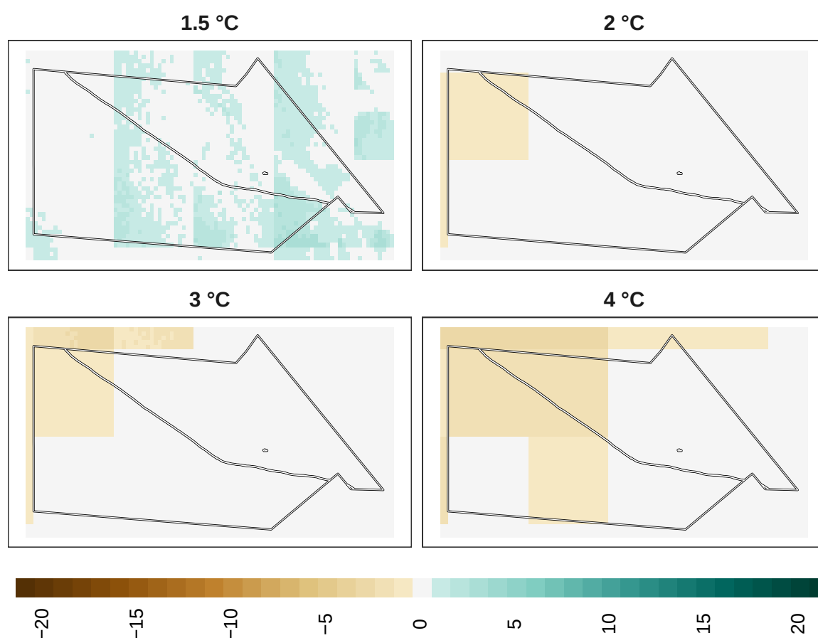
Figure 15: Adaptation effort for overall biodiversity at 1 km resolution.
