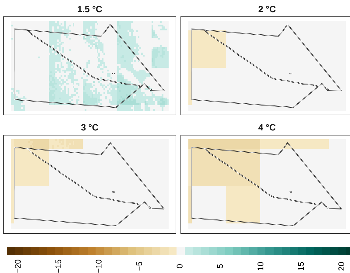
Figure 16: Adaptation effort for plants at 1 km resolution.
