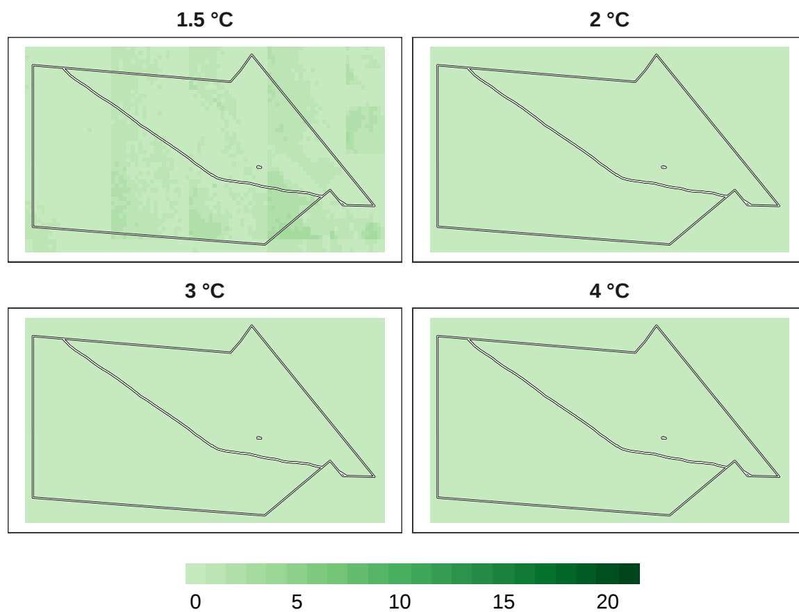
Figure 13: Number of models in agreement for reptile refugia at 1 km resolution.
