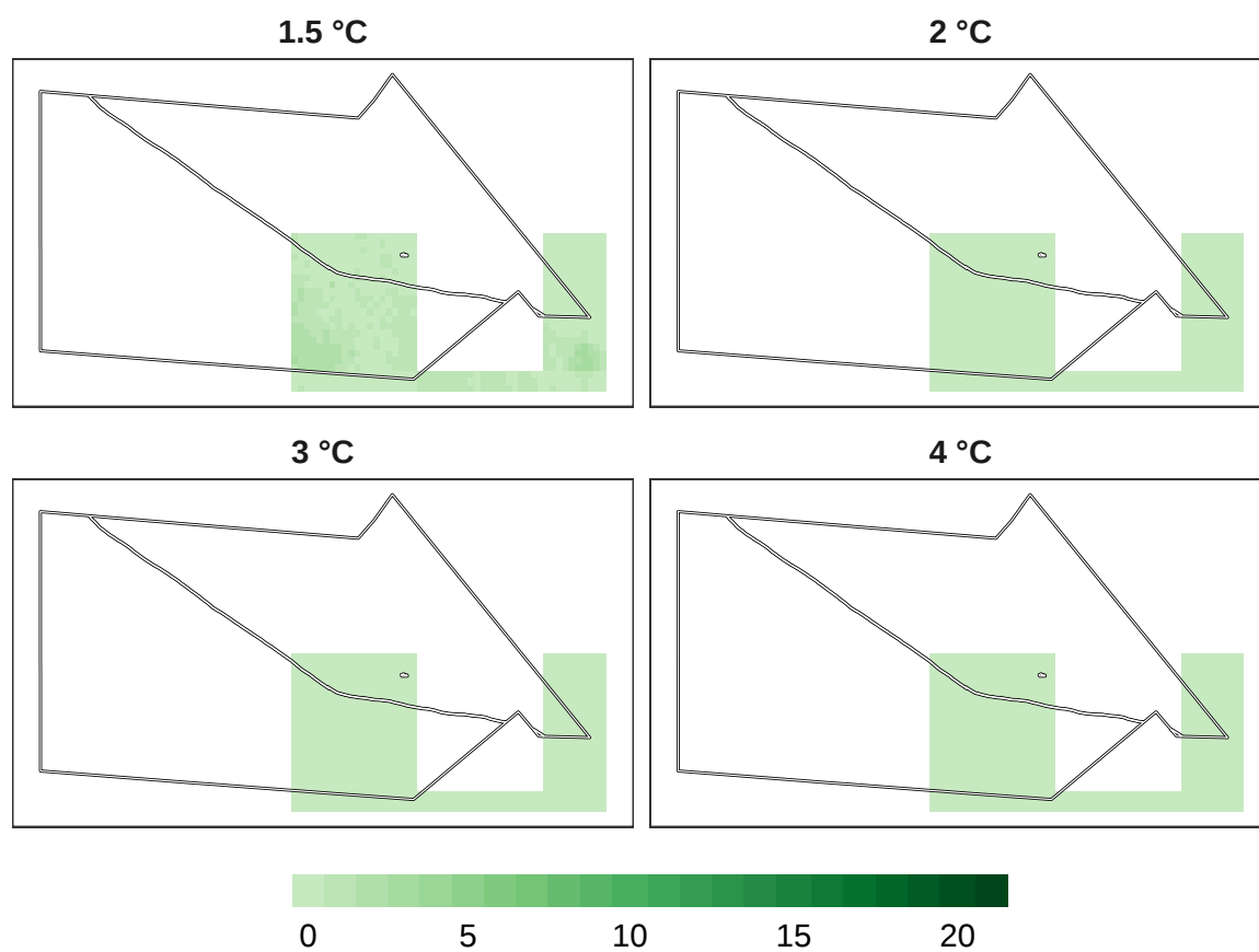
Figure 10: Number of models in agreement for amphibian refugia at 1 km resolution.
