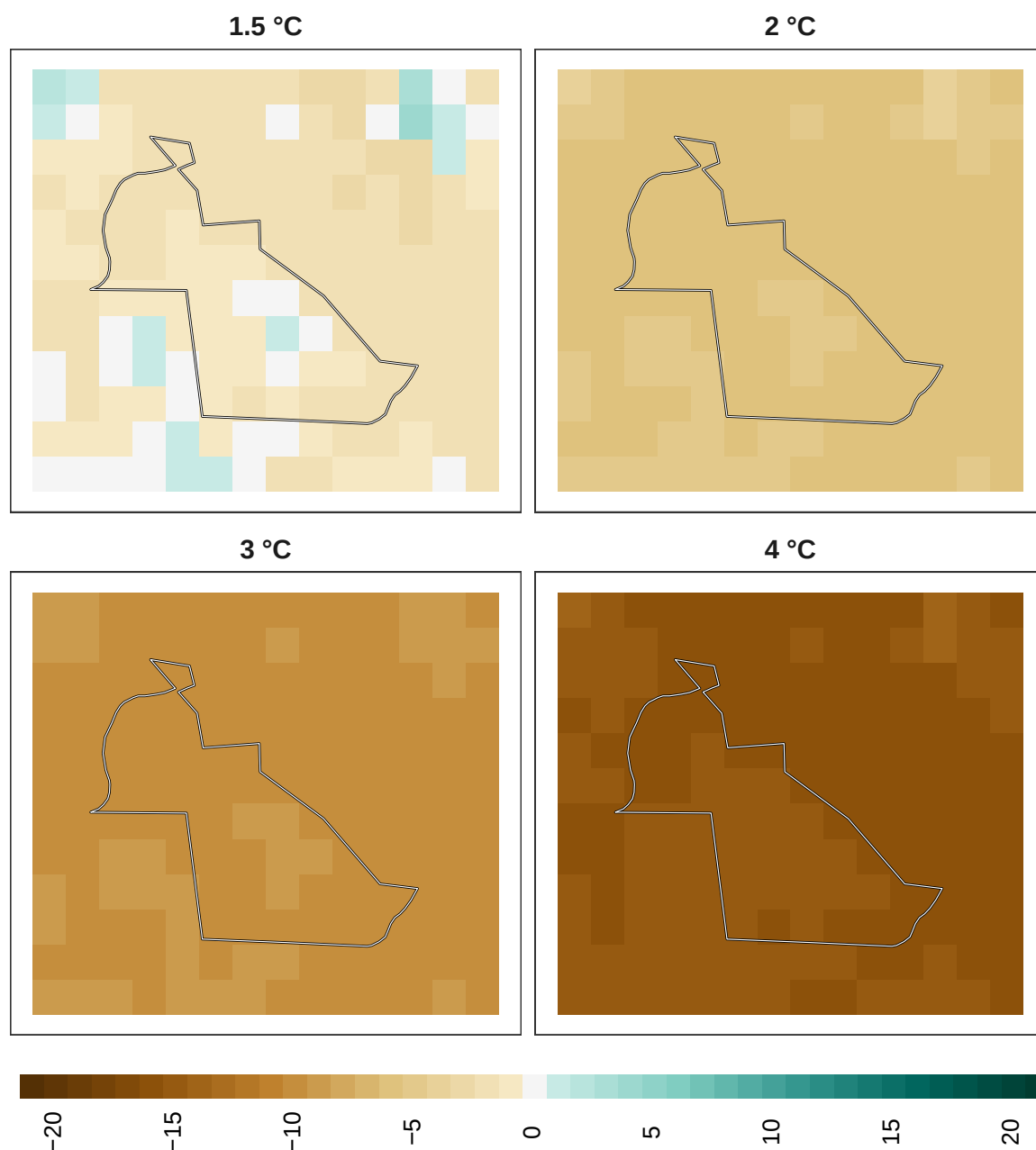
Figure 20: Adaptation effort for mammals at 1 km resolution.
