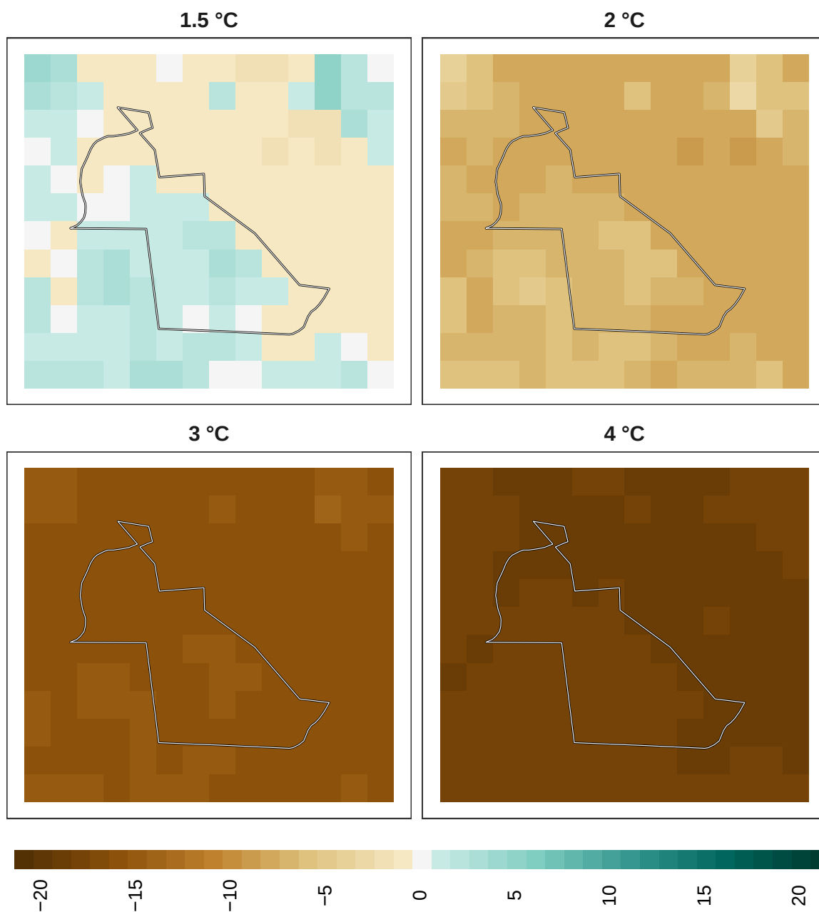
Figure 21: Adaptation effort for reptiles at 1 km resolution.
