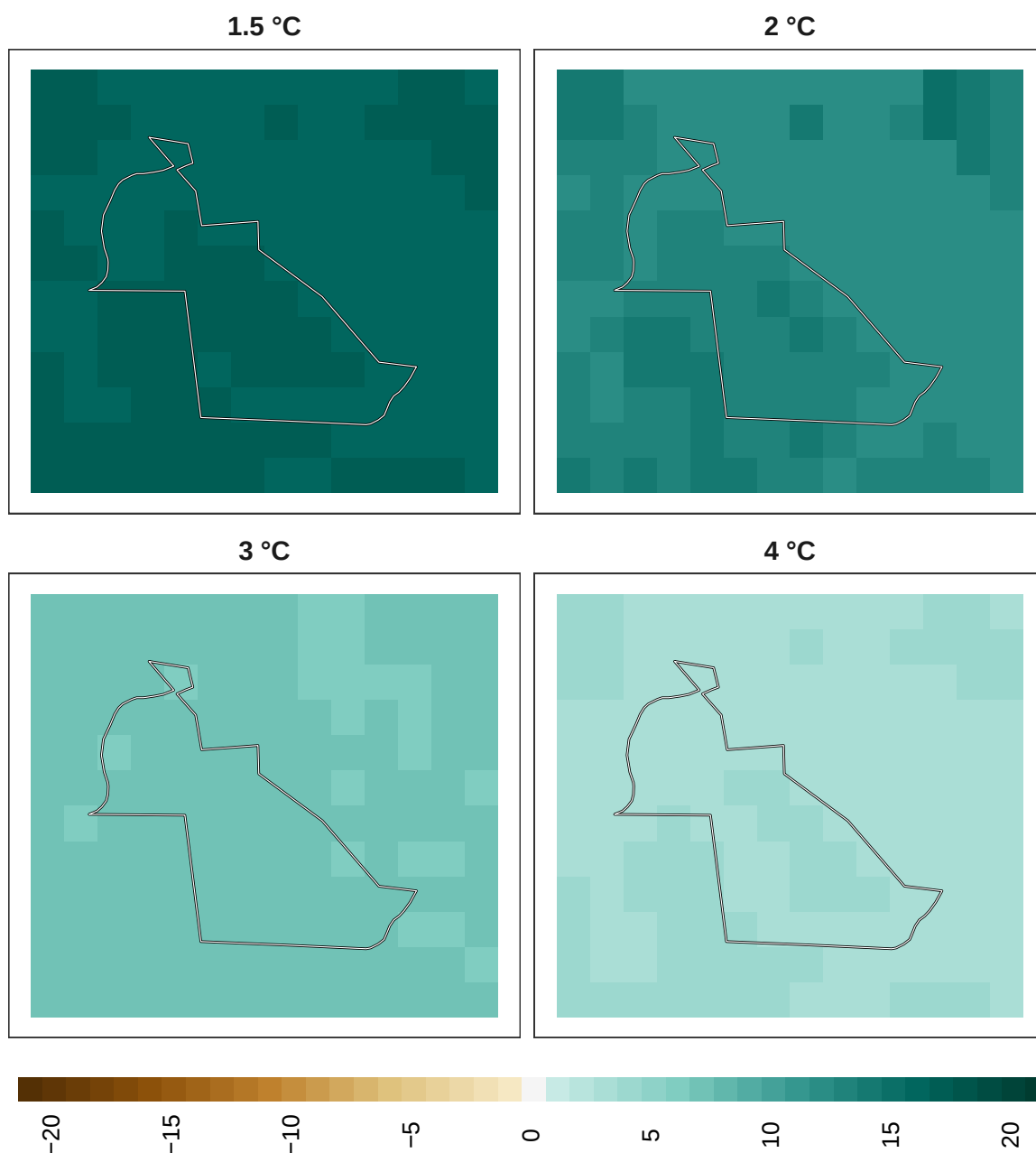
Figure 22: Adaptation effort for insects at 1 km resolution.
