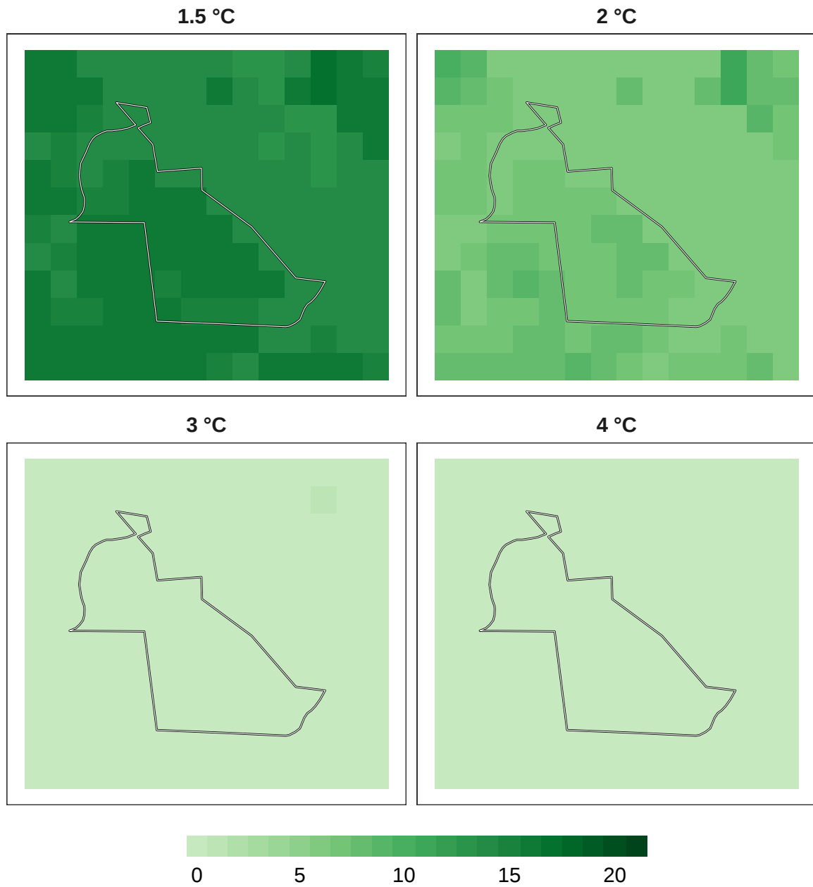
Figure 11: Number of models in agreement for amphibian refugia at 1 km resolution.
