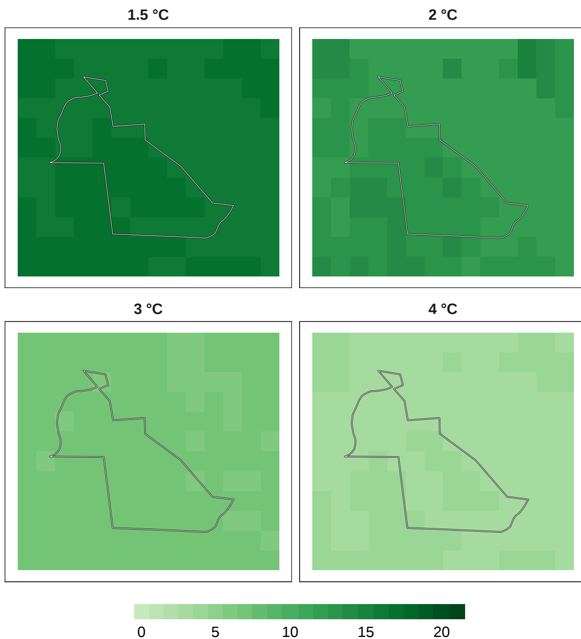
Figure 15: Number of models in agreement for insect refugia at 1 km resolution.
