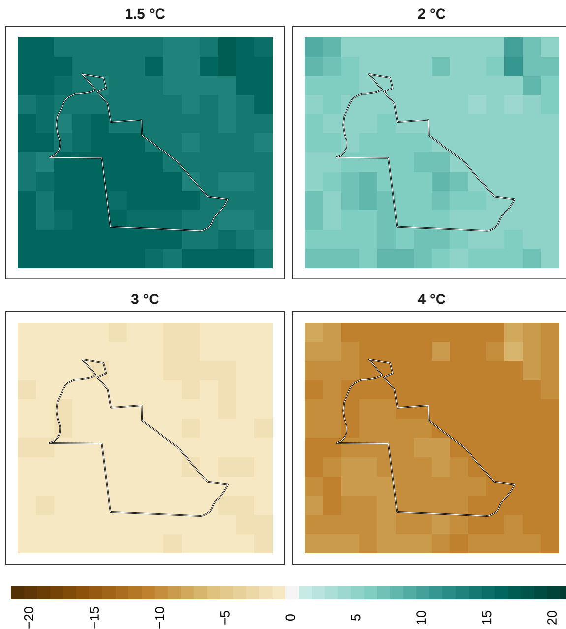
Figure 18: Adaptation effort for amphibians at 1 km resolution.
