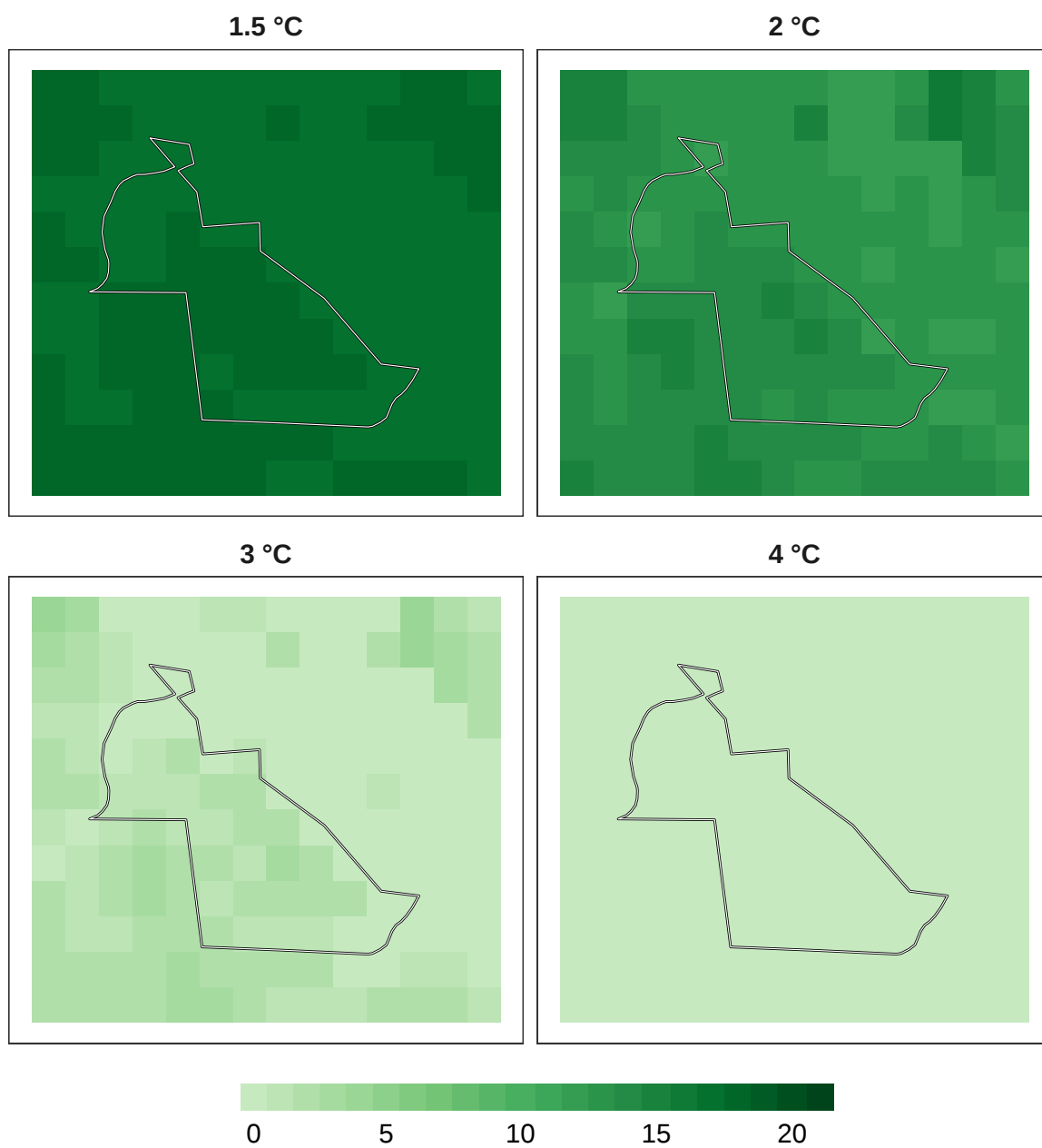
Figure 12: Number of models in agreement for bird refugia.
