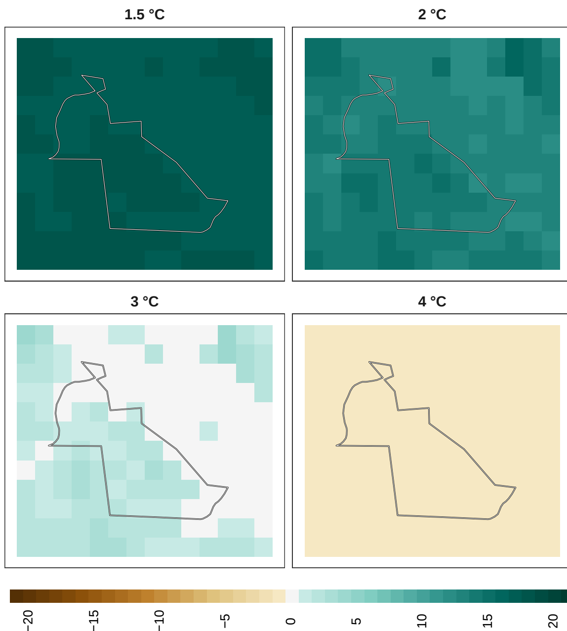
Figure 19: Adaptation effort for birds at 1 km resolution.
