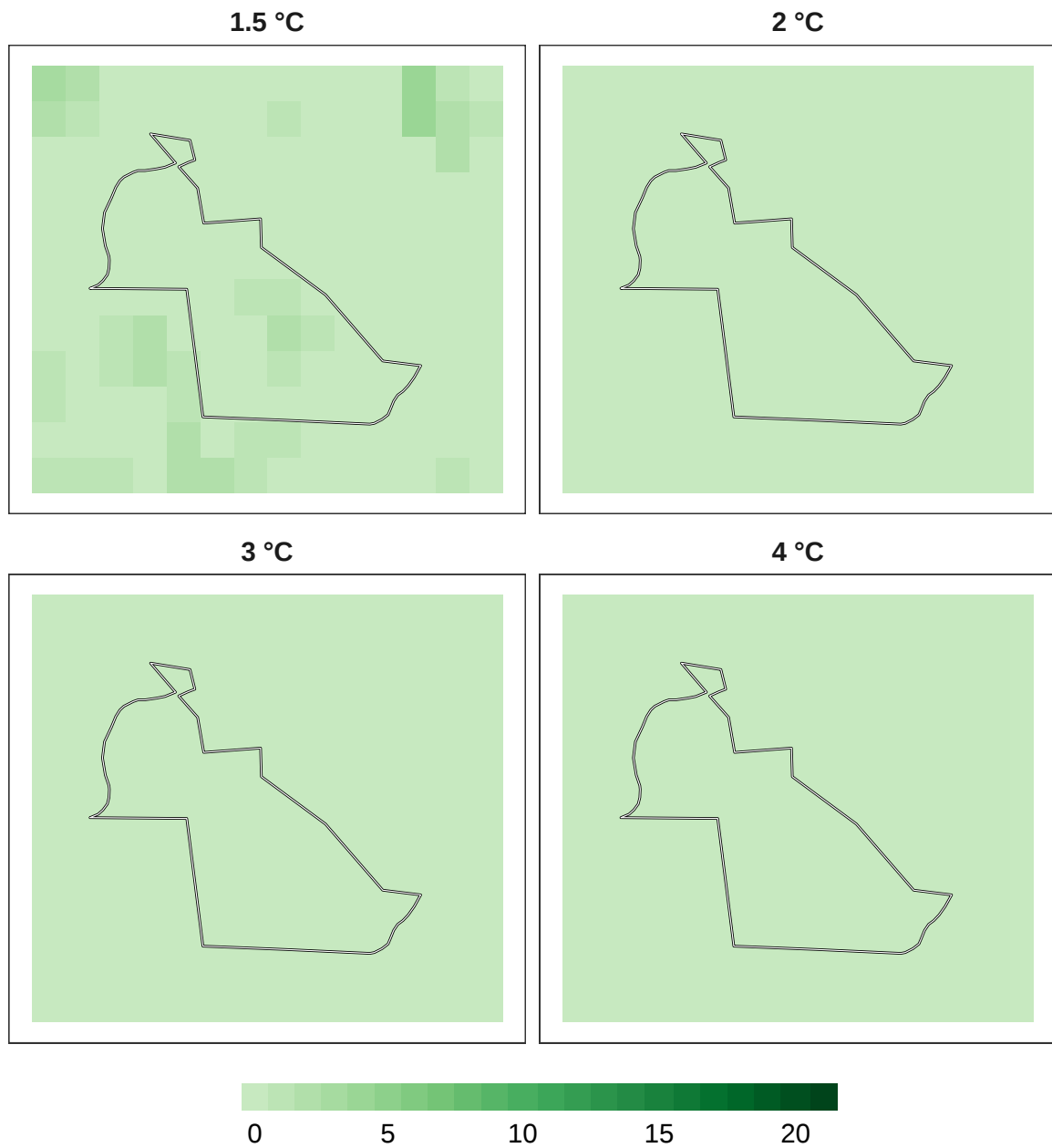
Figure 13: Number of models in agreement for mammal refugia at 1 km resolution.
