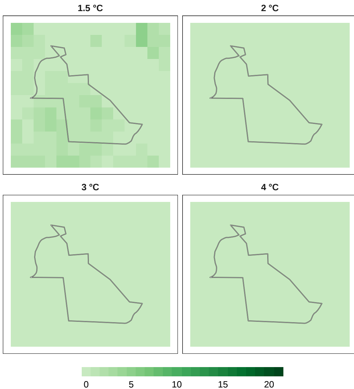
Figure 14: Number of models in agreement for reptile refugia at 1 km resolution.
