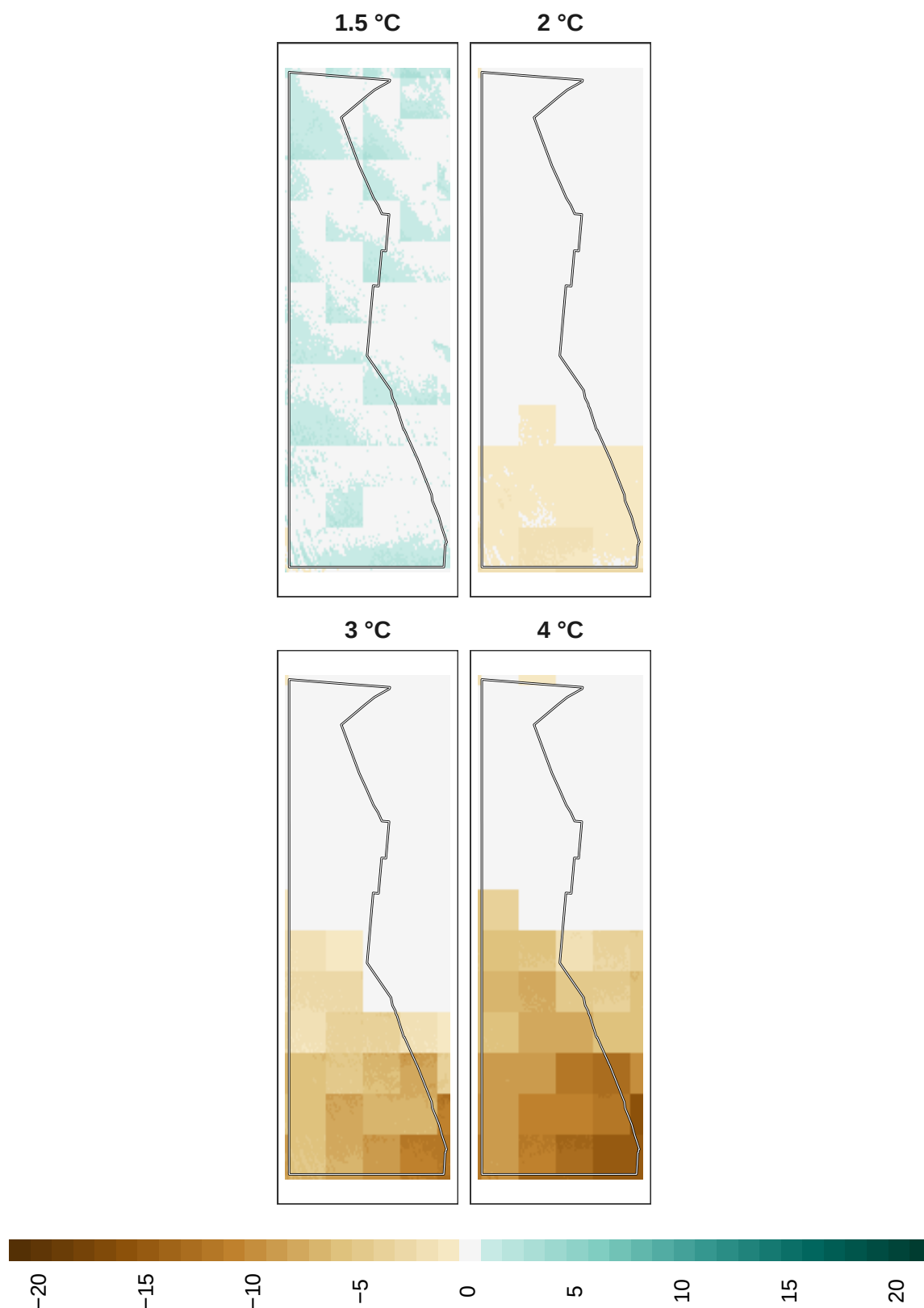
Figure 15: Adaptation effort for overall biodiversity at 1 km resolution.
