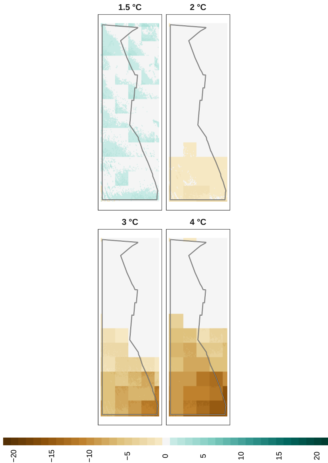
Figure 16: Adaptation effort for plants at 1 km resolution.
