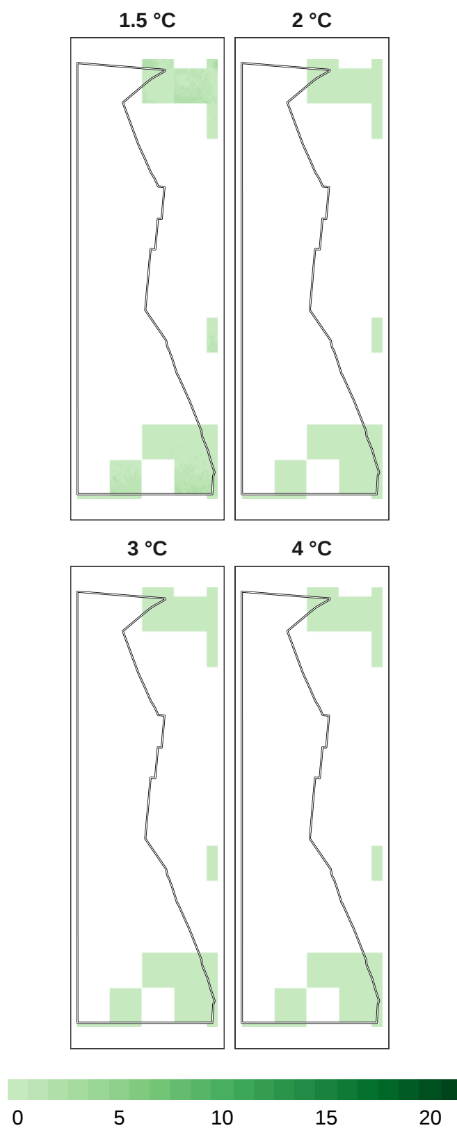
Figure 10: Number of models in agreement for amphibian refugia at 1 km resolution.
