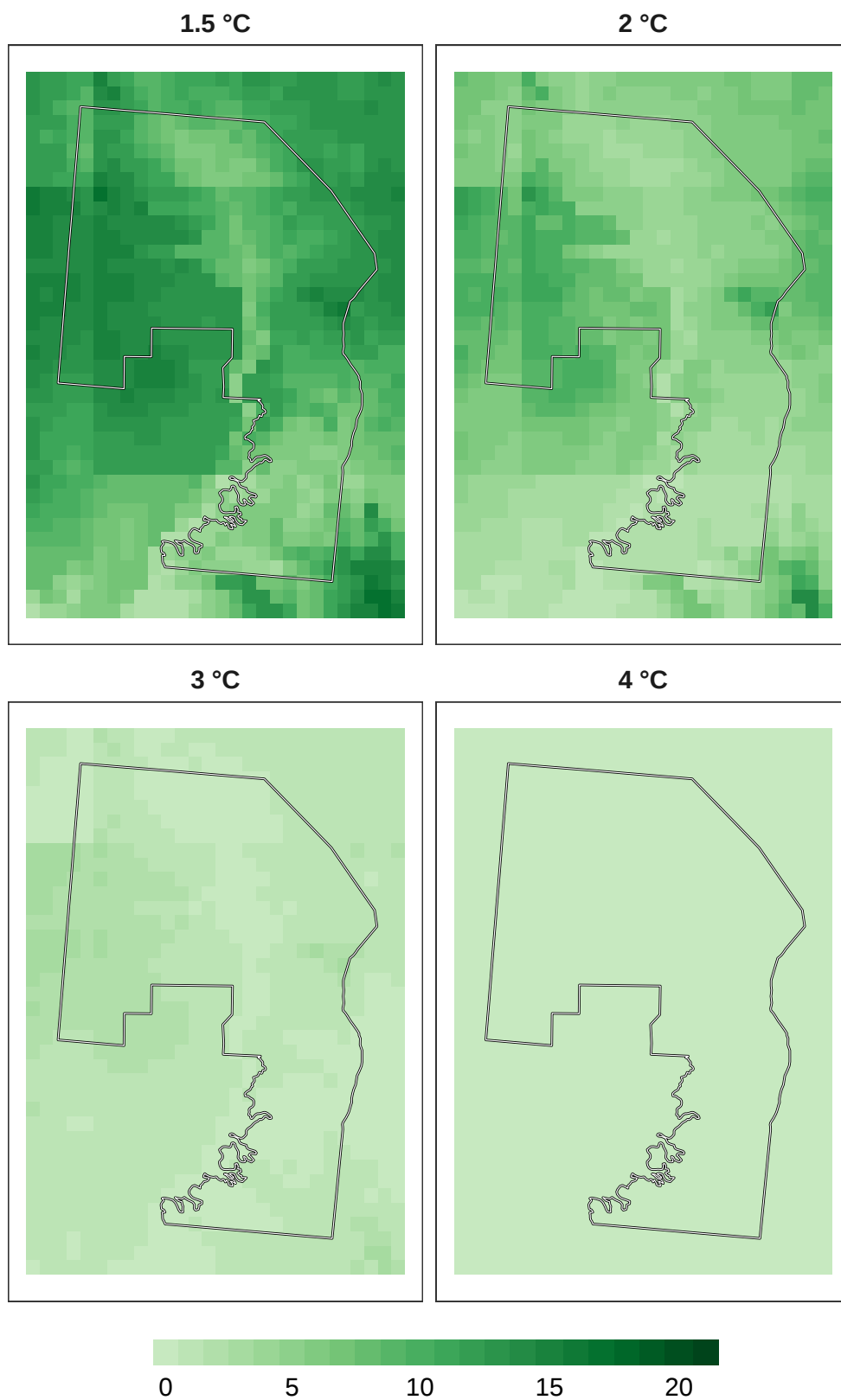
Figure 15: Number of models in agreement for reptile refugia at 1 km resolution.
