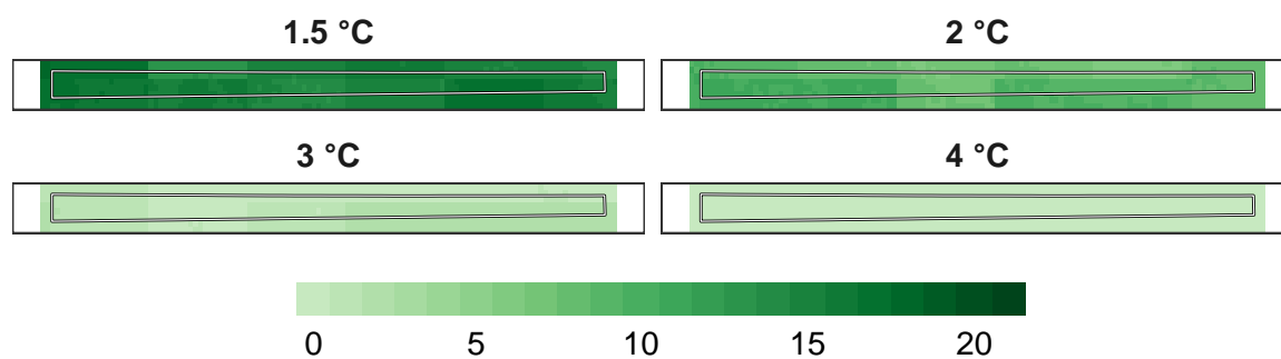
Figure 12: Number of models in agreement for bird refugia.
