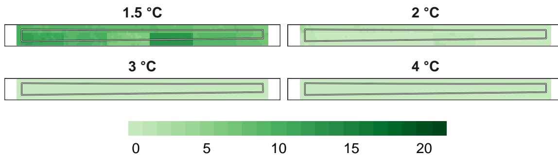
Figure 9: Number of models in agreement for overall biodiversity refugia at 1 km resolution.
