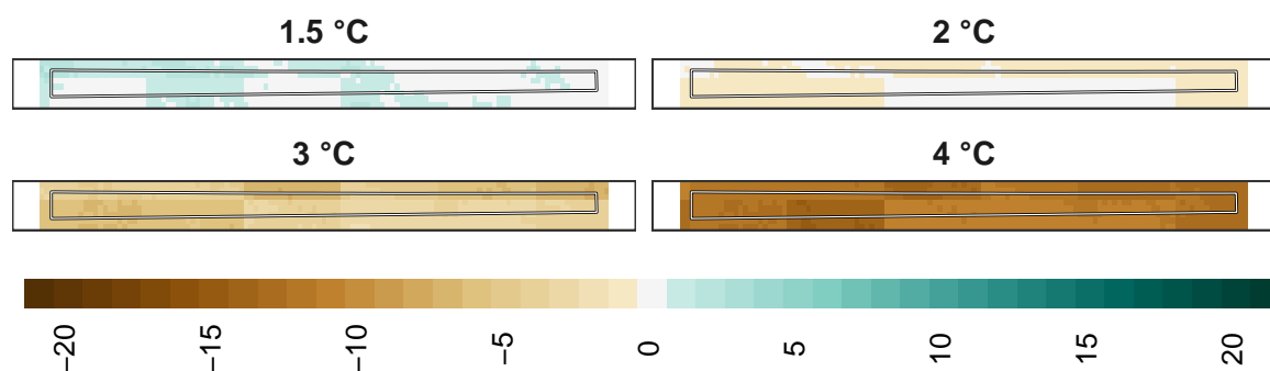
Figure 20: Adaptation effort for mammals at 1 km resolution.
