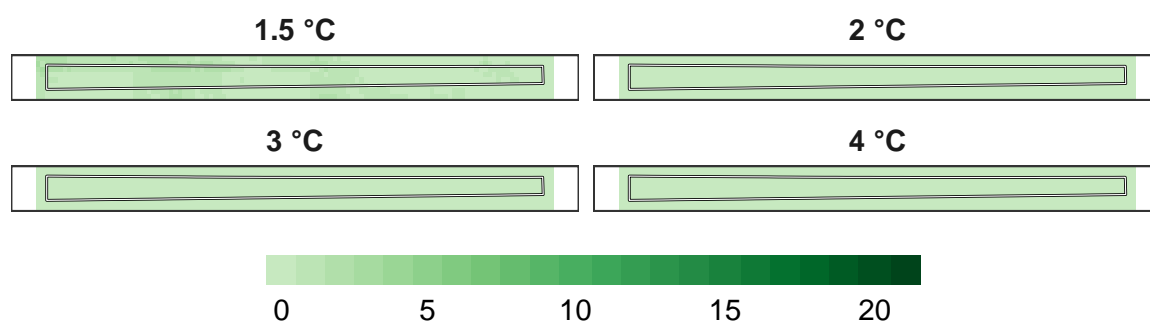
Figure 13: Number of models in agreement for mammal refugia at 1 km resolution.
