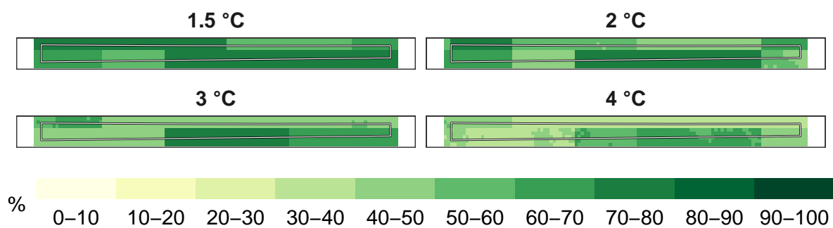
Figure 8: Percent timber species remaining at 1 km resolution.
