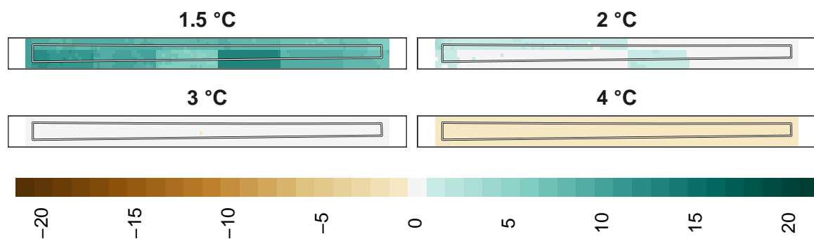
Figure 16: Adaptation effort for overall biodiversity at 1 km resolution.
