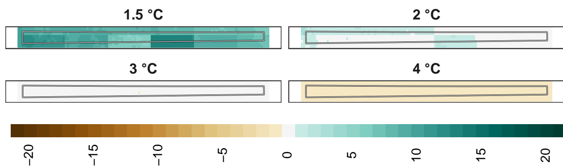
Figure 17: Adaptation effort for plants at 1 km resolution.
