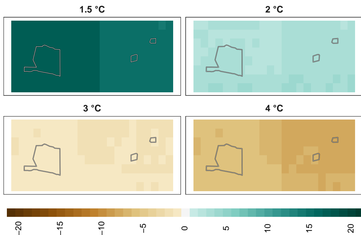
Figure 22: Adaptation effort for insects at 1 km resolution.
