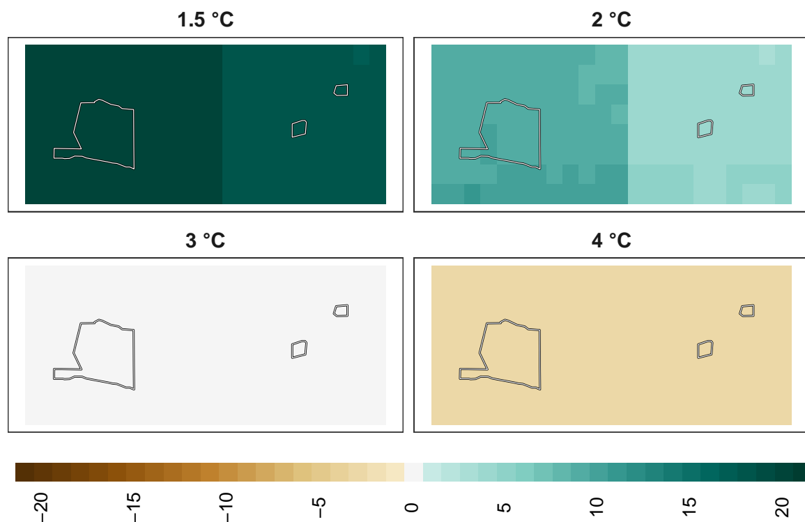
Figure 21: Adaptation effort for reptiles at 1 km resolution.
