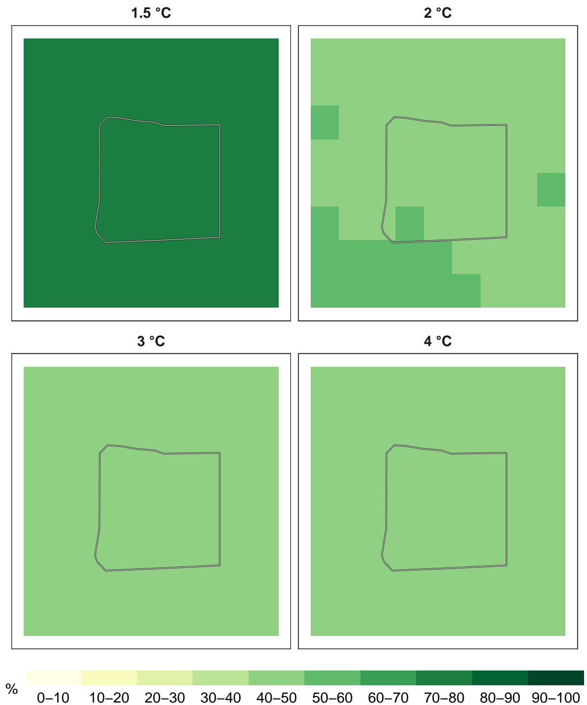
Figure 8: Percent timber species remaining at 1 km resolution.
