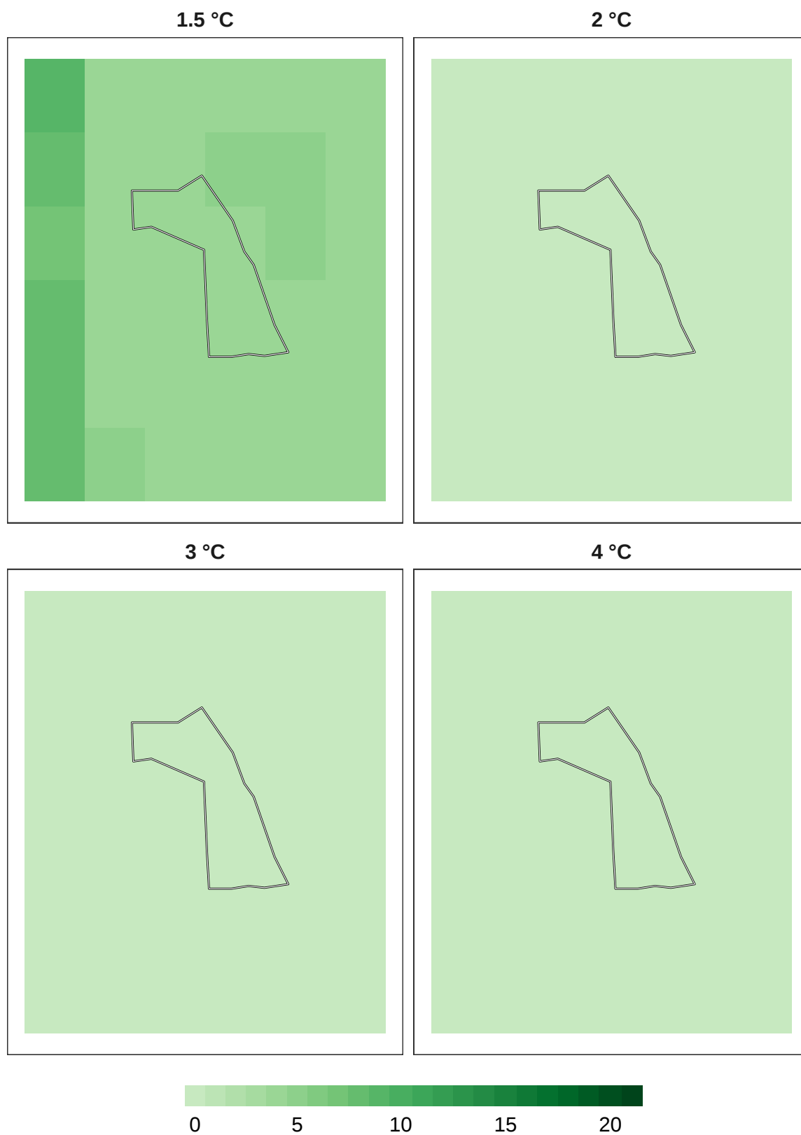
Figure 15: Number of models in agreement for insect refugia at 1 km resolution.
