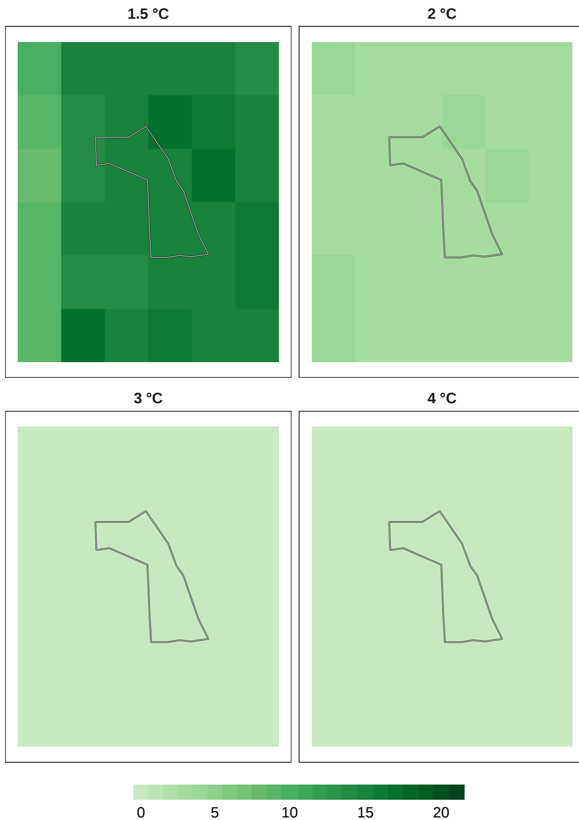
Figure 14: Number of models in agreement for reptile refugia at 1 km resolution.
