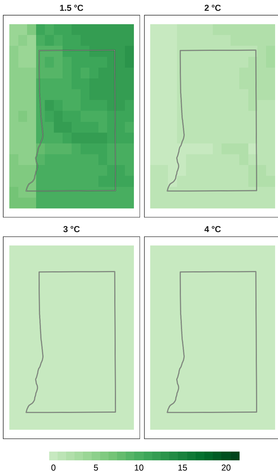
Figure 14: Number of models in agreement for reptile refugia at 1 km resolution.
