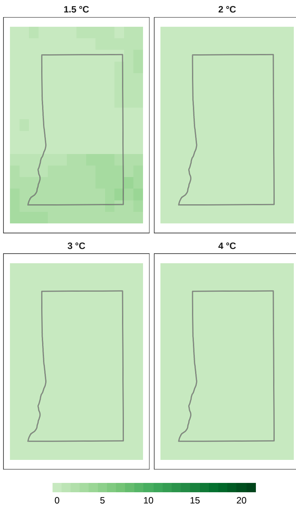
Figure 15: Number of models in agreement for insect refugia at 1 km resolution.
