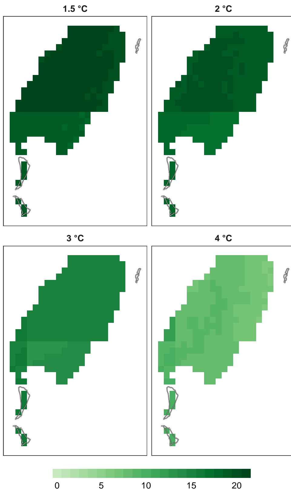
Figure 10: Number of models in agreement for reptile refugia at 1 km resolution.
