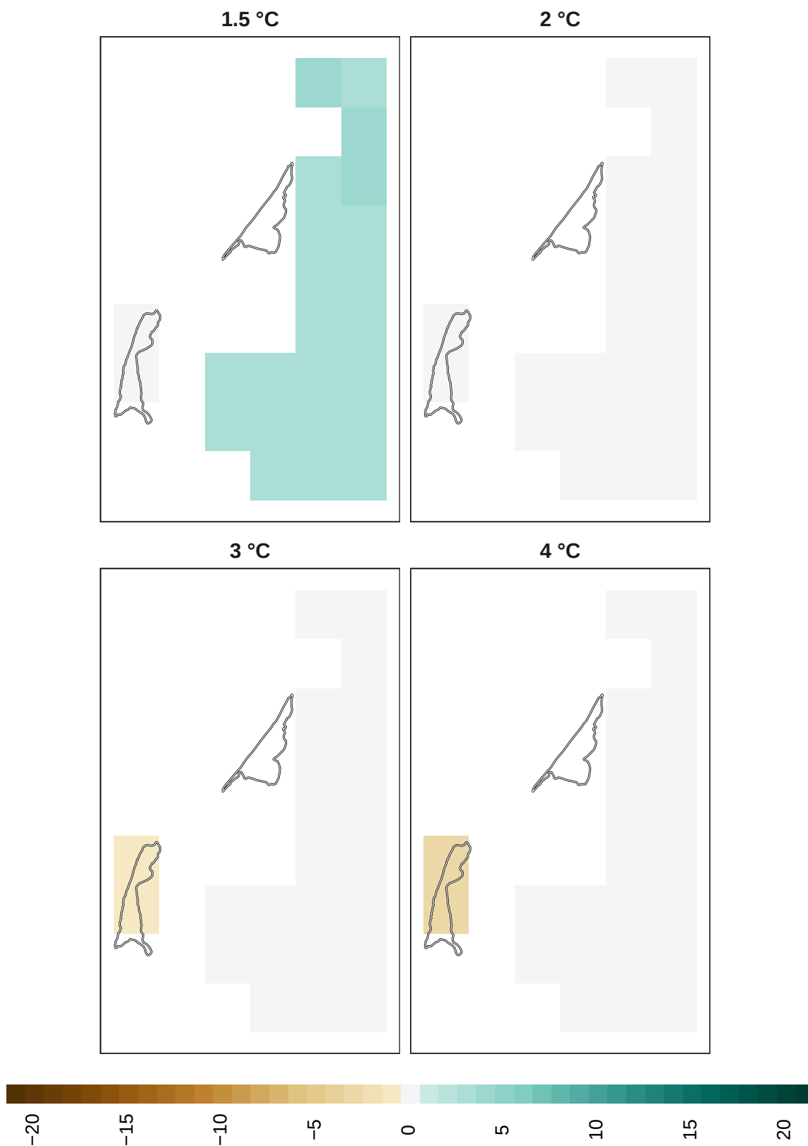
Figure 14: Adaptation effort for reptiles at 1 km resolution.
