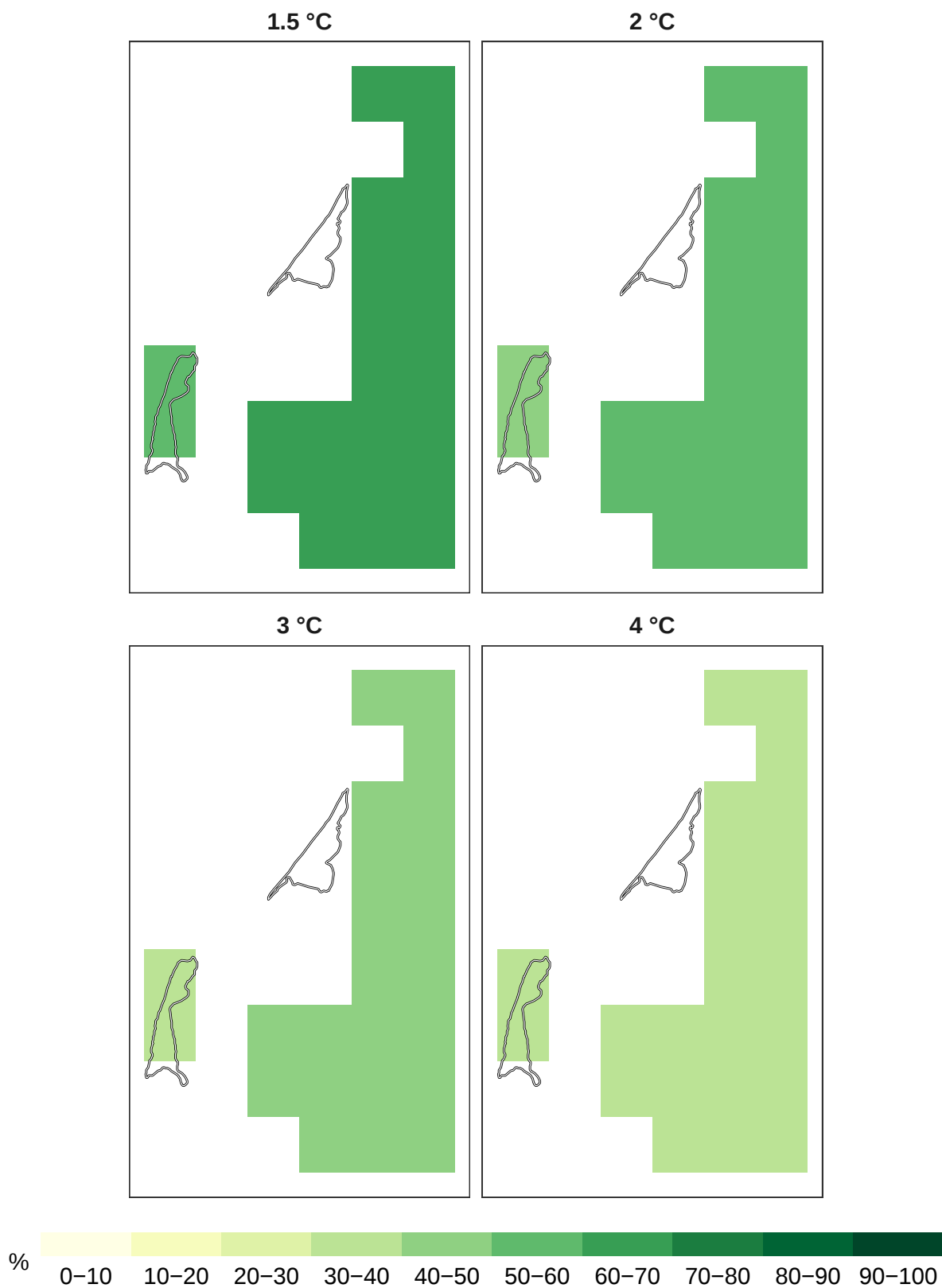
Figure 4: Percent reptiles remaining at 1 km resolution.
