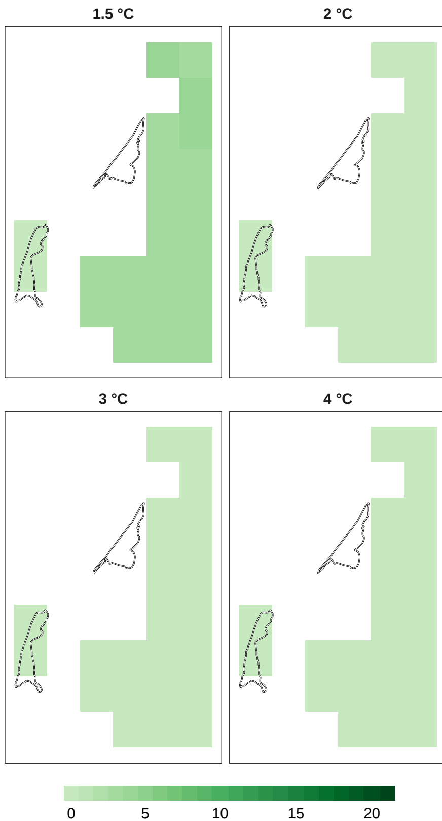
Figure 9: Number of models in agreement for reptile refugia at 1 km resolution.
