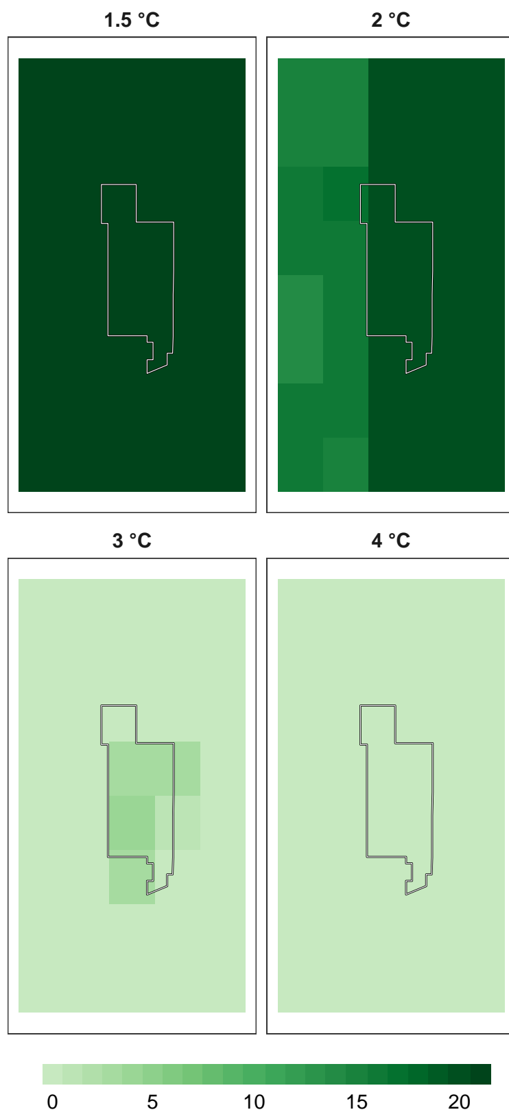
Figure 14: Number of models in agreement for reptile refugia at 1 km resolution.
