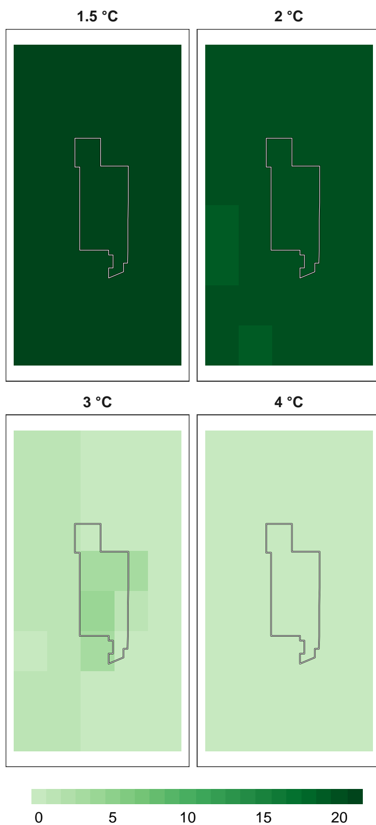
Figure 15: Number of models in agreement for insect refugia at 1 km resolution.
