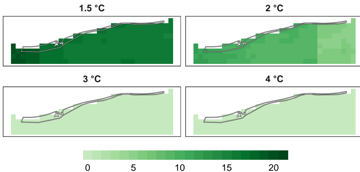
Figure 8: Number of models in agreement for overall biodiversity refugia at 1 km resolution.
