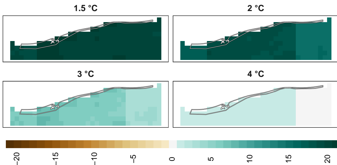
Figure 18: Adaptation effort for insects at 1 km resolution.
