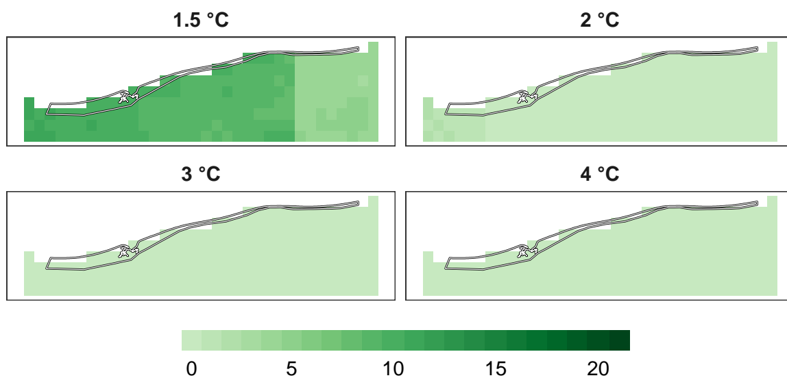
Figure 11: Number of models in agreement for reptile refugia at 1 km resolution.
