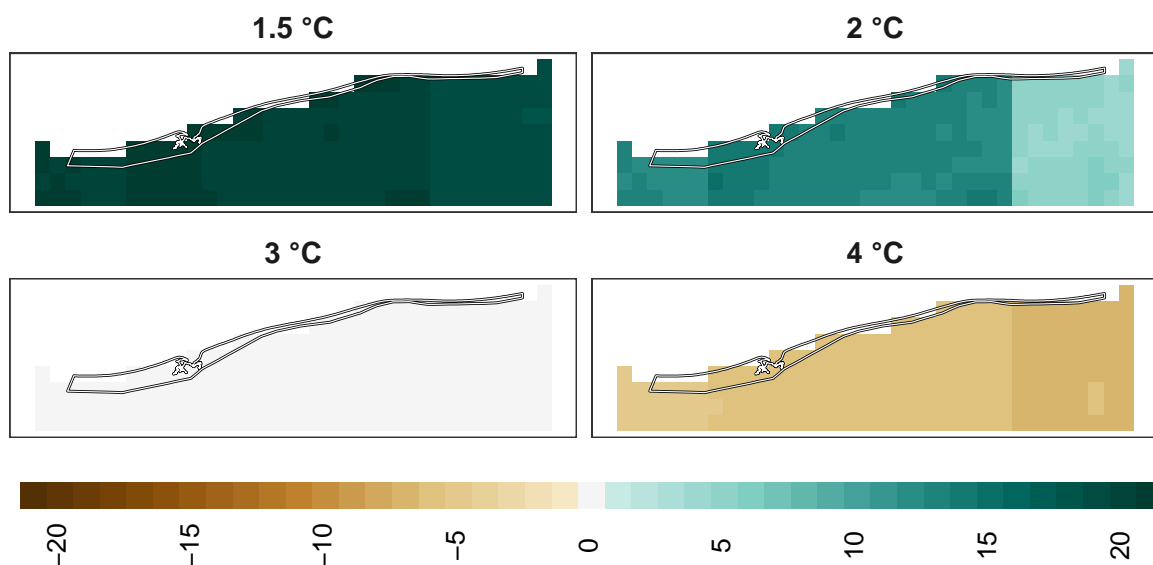
Figure 16: Adaptation effort for birds at 1 km resolution.
