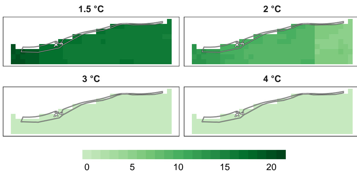
Figure 9: Number of models in agreement for plant refugia at 1 km resolution.
