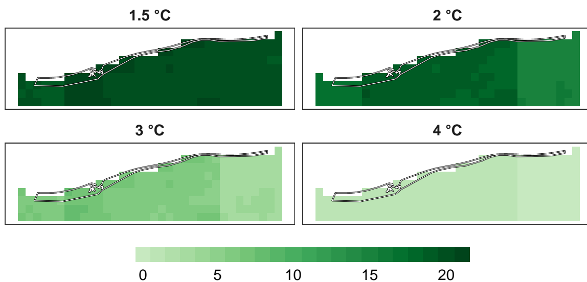
Figure 12: Number of models in agreement for insect refugia at 1 km resolution.
