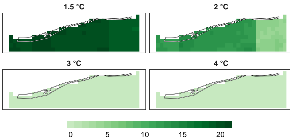
Figure 10: Number of models in agreement for bird refugia.
