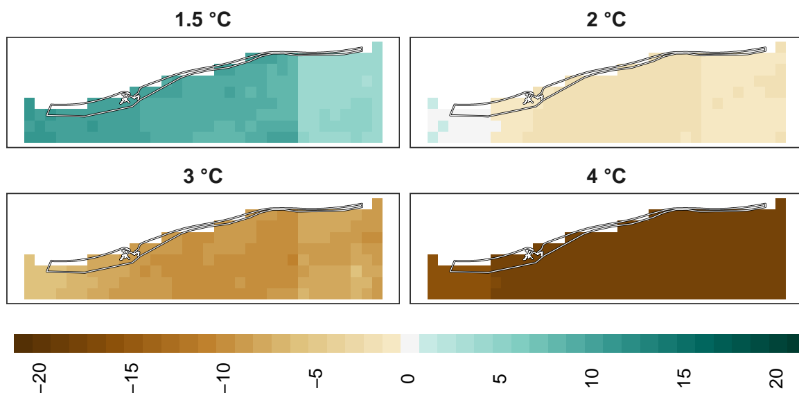
Figure 17: Adaptation effort for reptiles at 1 km resolution.
