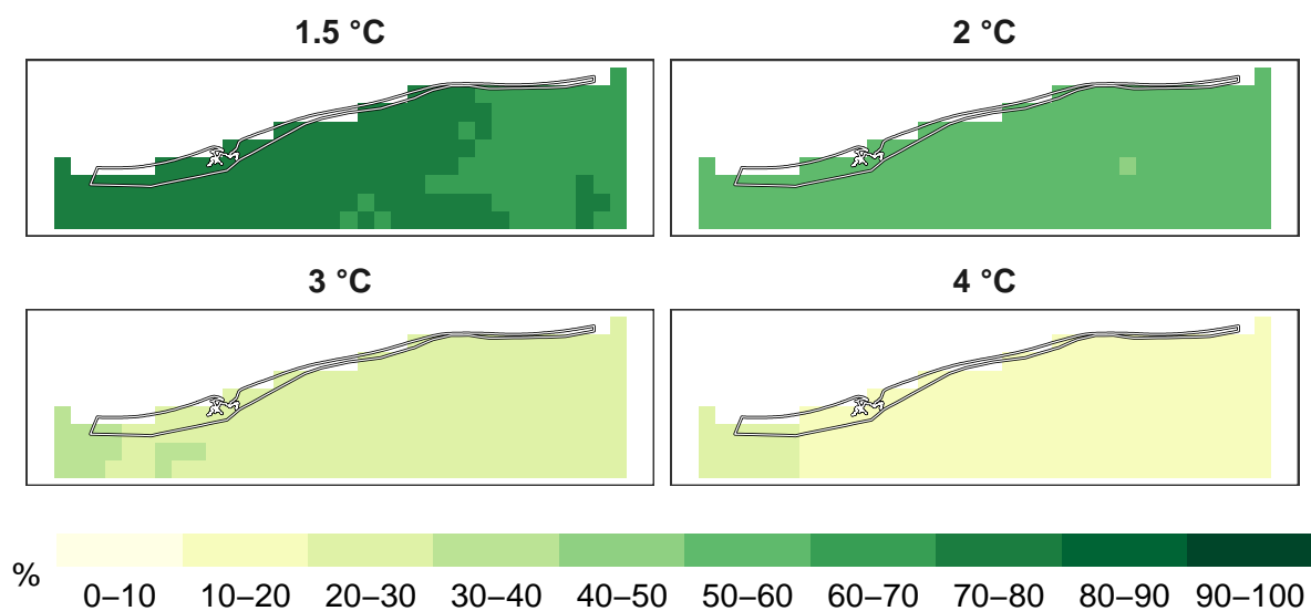
Figure 4: Percent reptiles remaining at 1 km resolution.
