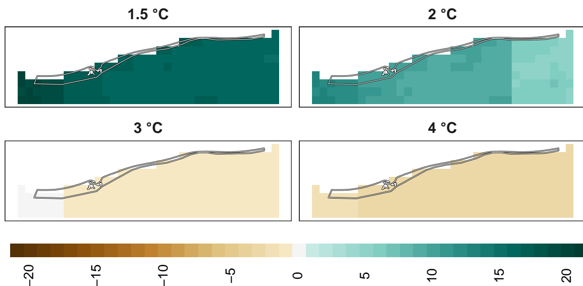
Figure 15: Adaptation effort for plants at 1 km resolution.
