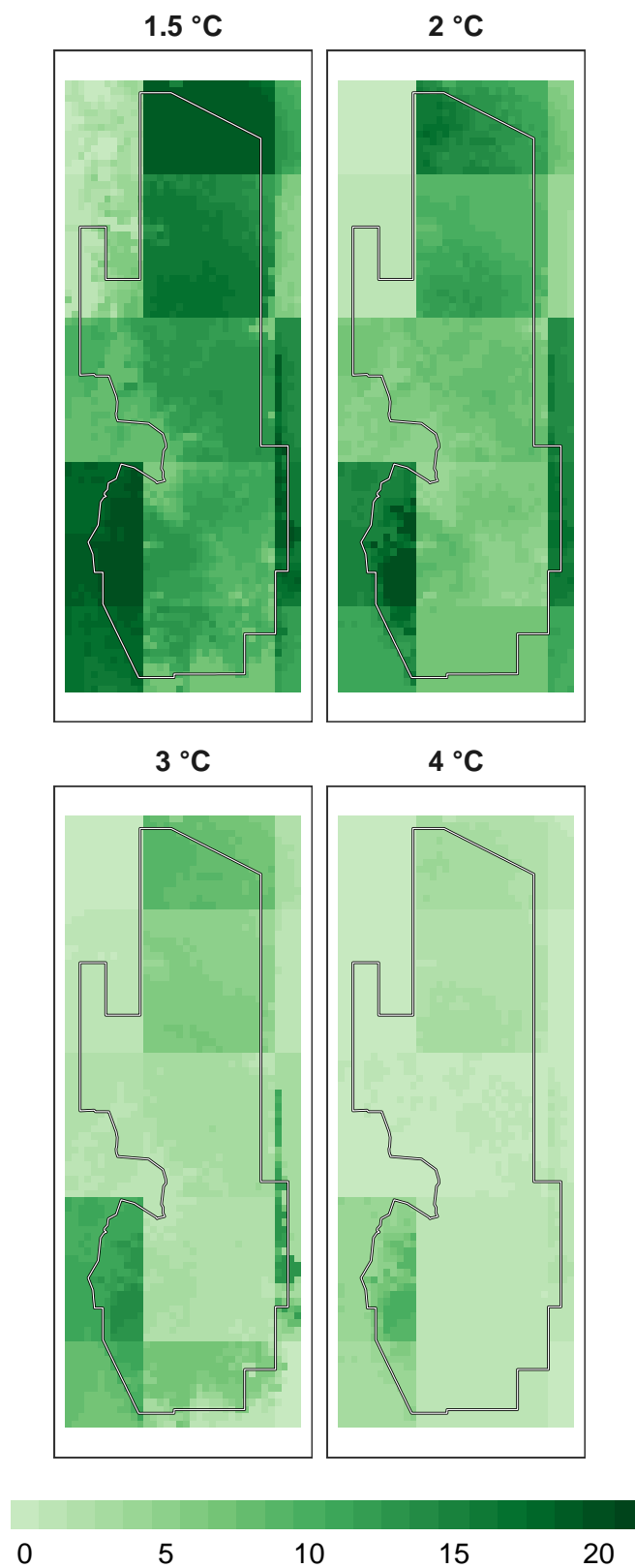
Figure 9: Number of models in agreement for reptile refugia at 1 km resolution.
