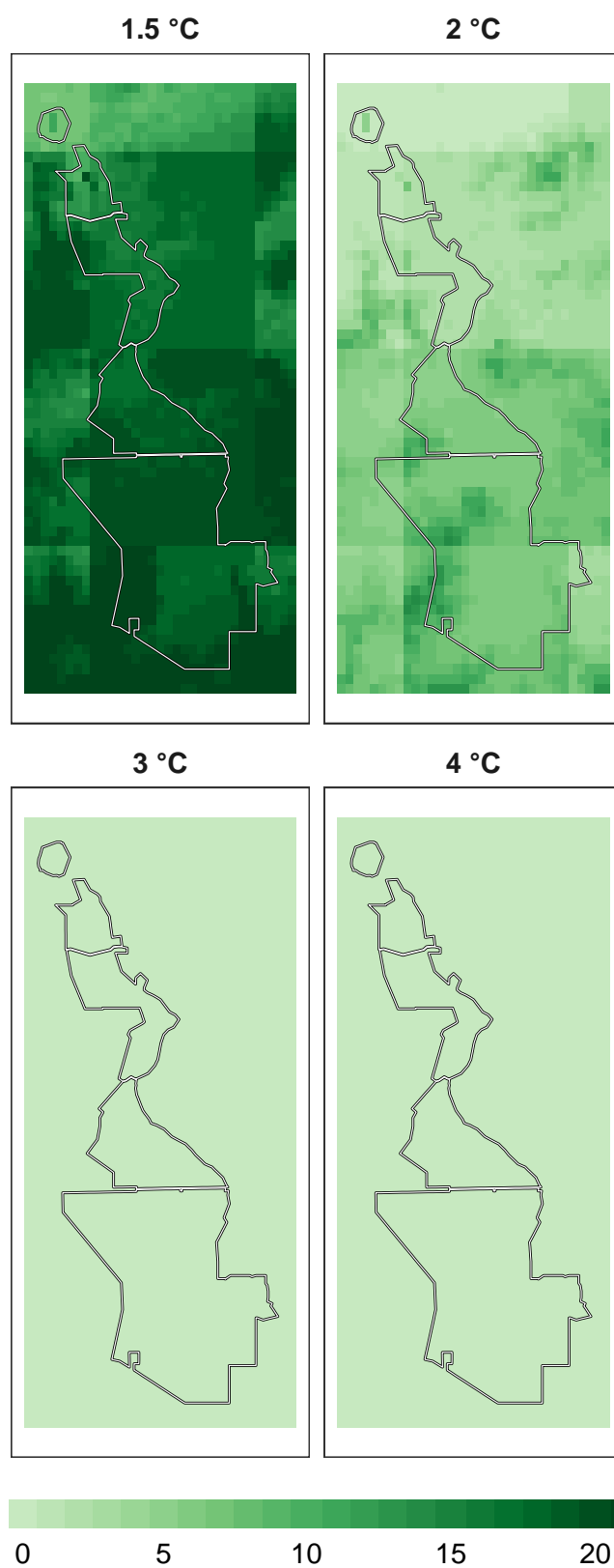
Figure 15: Number of models in agreement for insect refugia at 1 km resolution.
