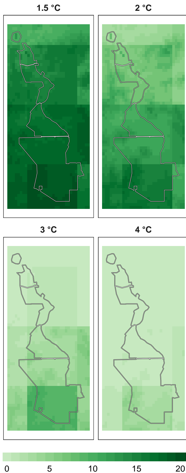
Figure 14: Number of models in agreement for reptile refugia at 1 km resolution.
