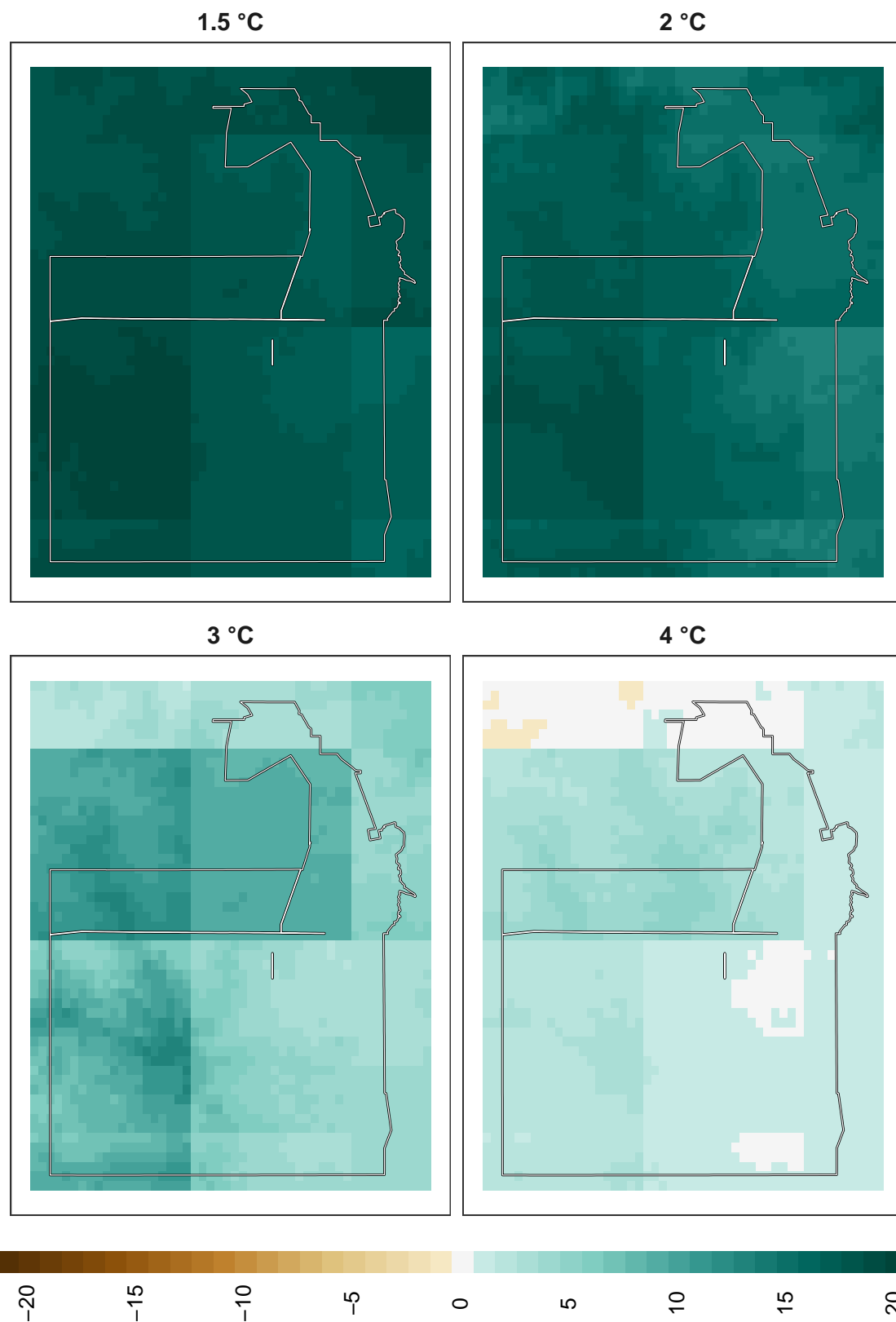
Figure 21: Adaptation effort for reptiles at 1 km resolution.
