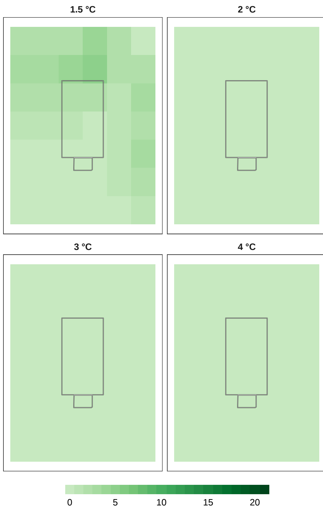
Figure 13: Number of models in agreement for mammal refugia at 1 km resolution.
