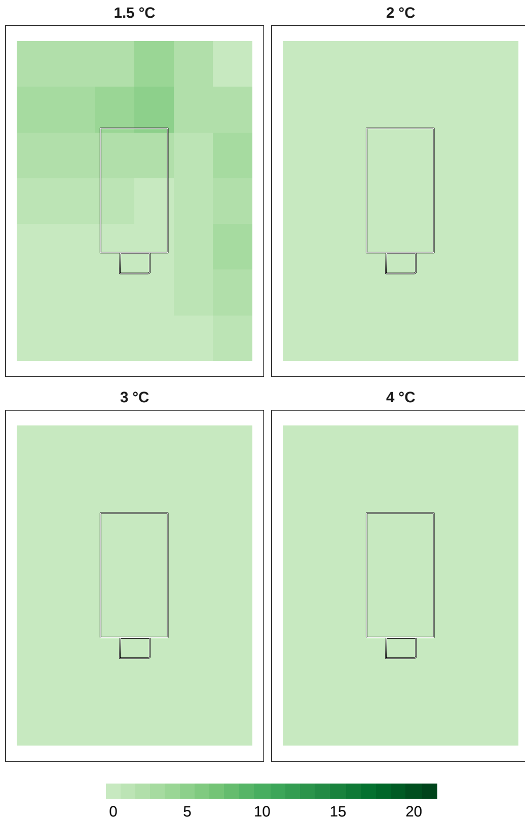
Figure 11: Number of models in agreement for amphibian refugia at 1 km resolution.
