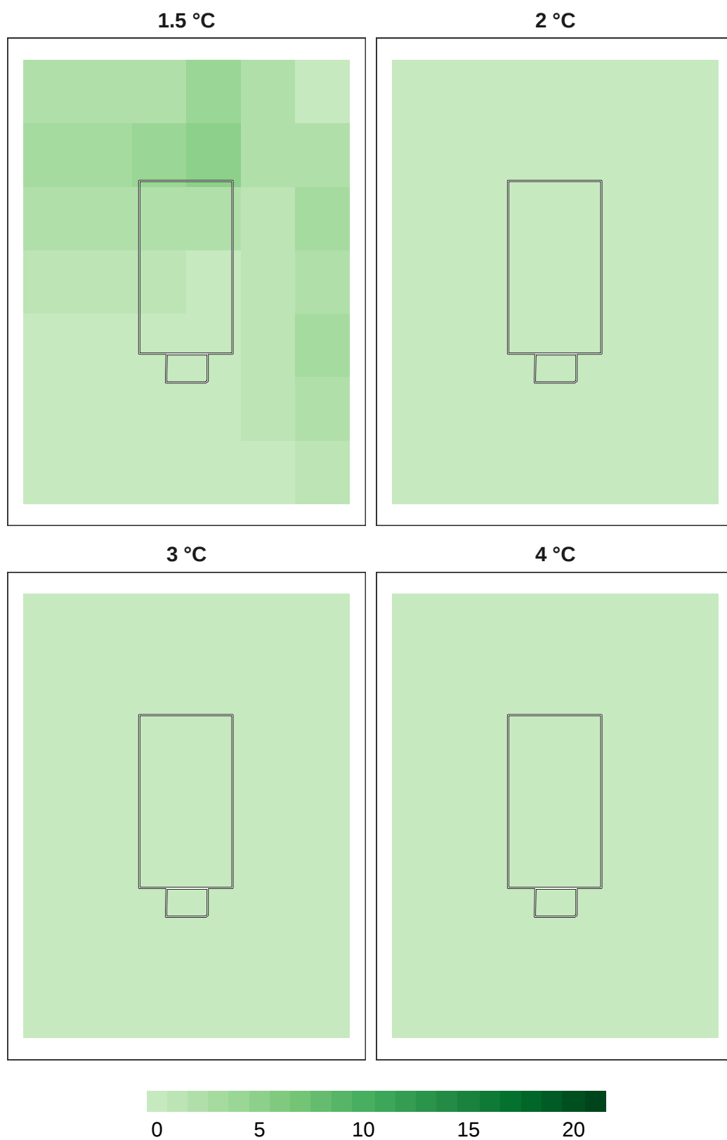
Figure 14: Number of models in agreement for reptile refugia at 1 km resolution.
