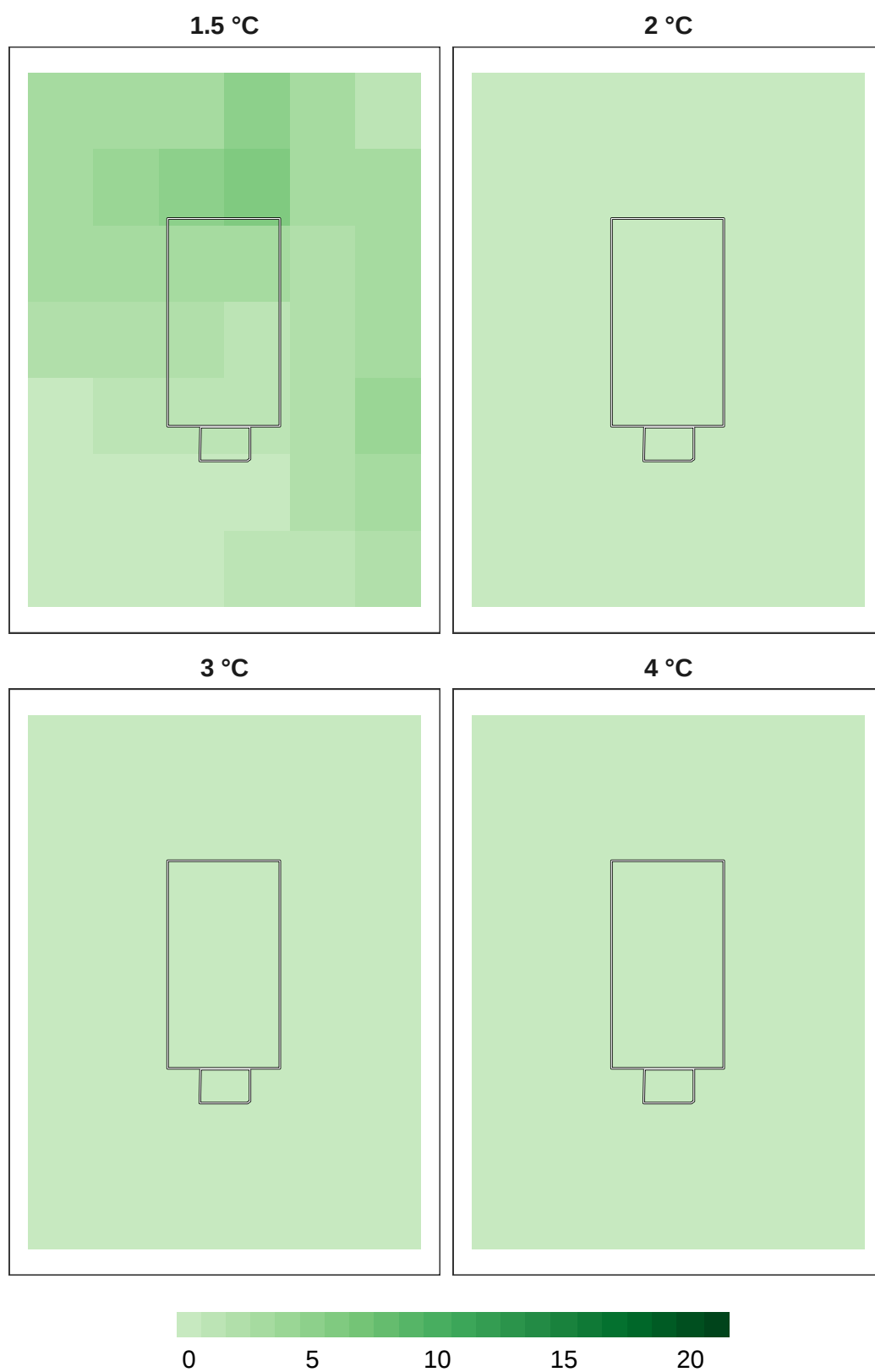
Figure 12: Number of models in agreement for bird refugia.
