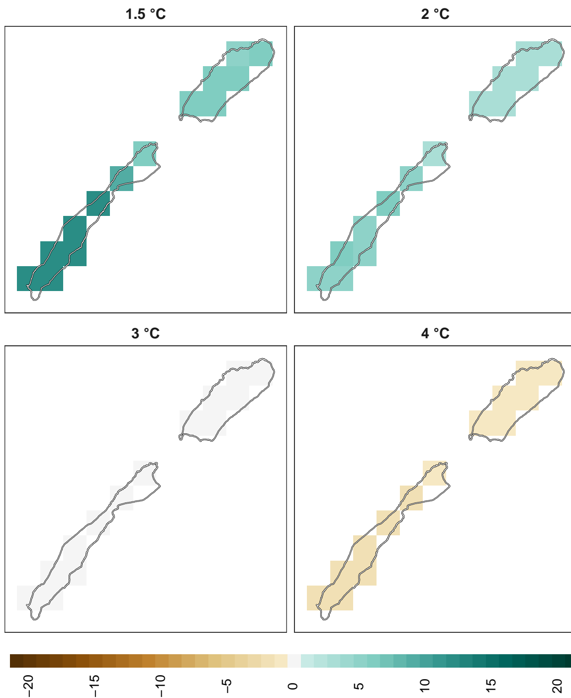
Figure 14: Adaptation effort for reptiles at 1 km resolution.
