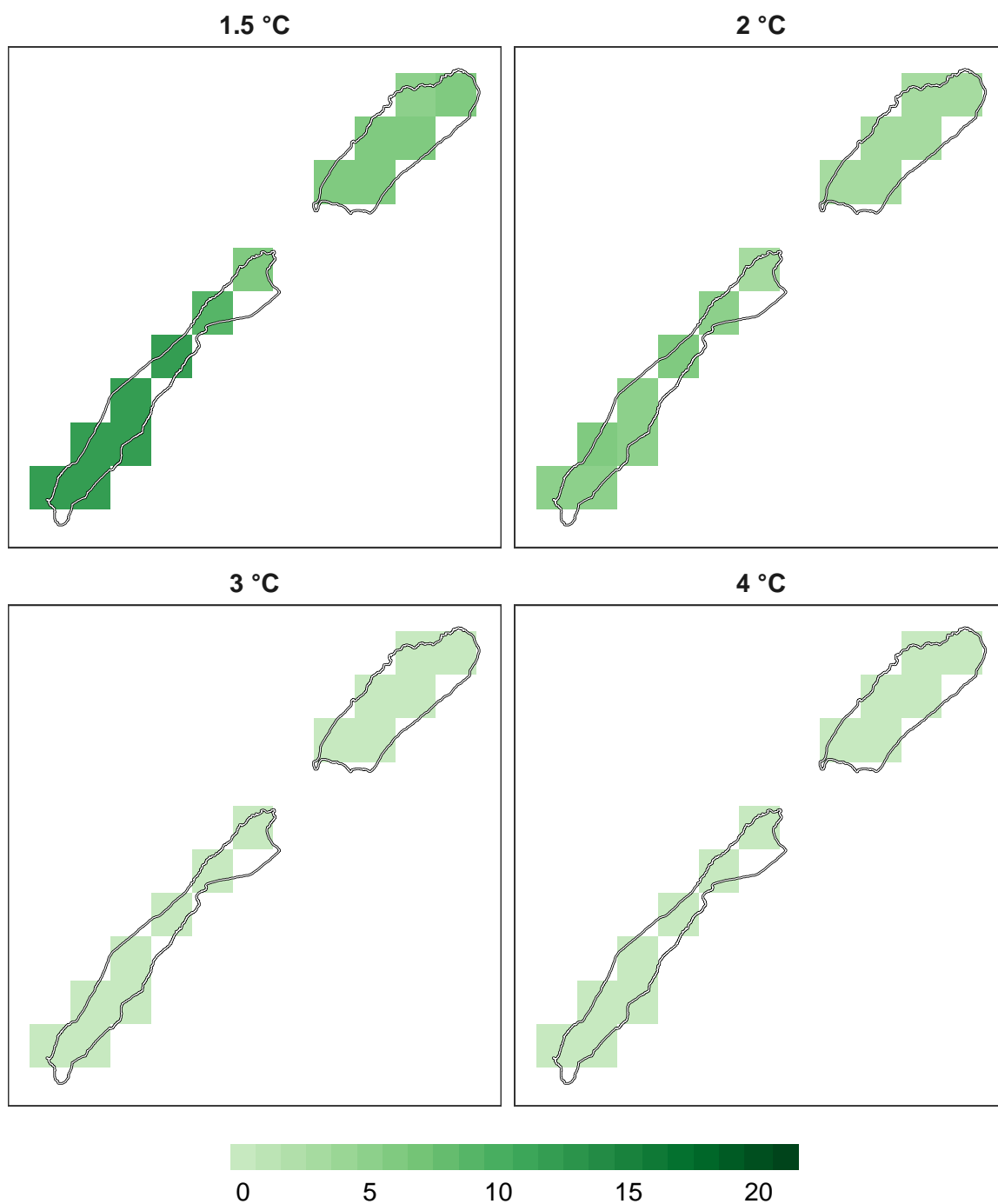
Figure 9: Number of models in agreement for reptile refugia at 1 km resolution.
