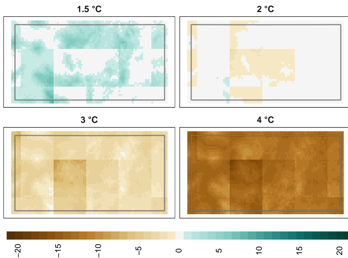
Figure 19: Adaptation effort for insects at 1 km resolution.
