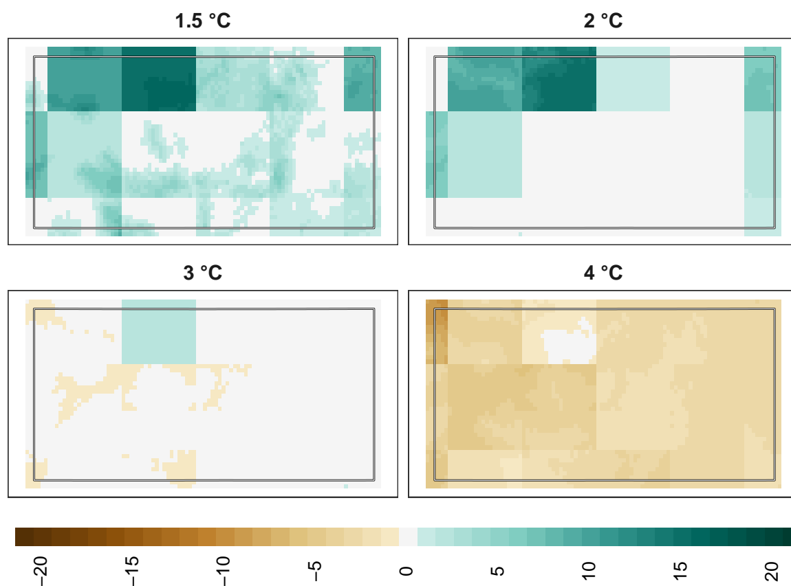
Figure 18: Adaptation effort for reptiles at 1 km resolution.
