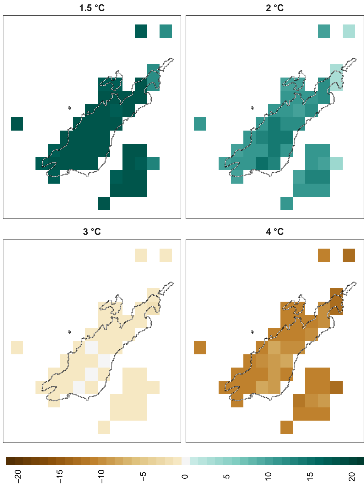
Figure 14: Adaptation effort for reptiles at 1 km resolution.
