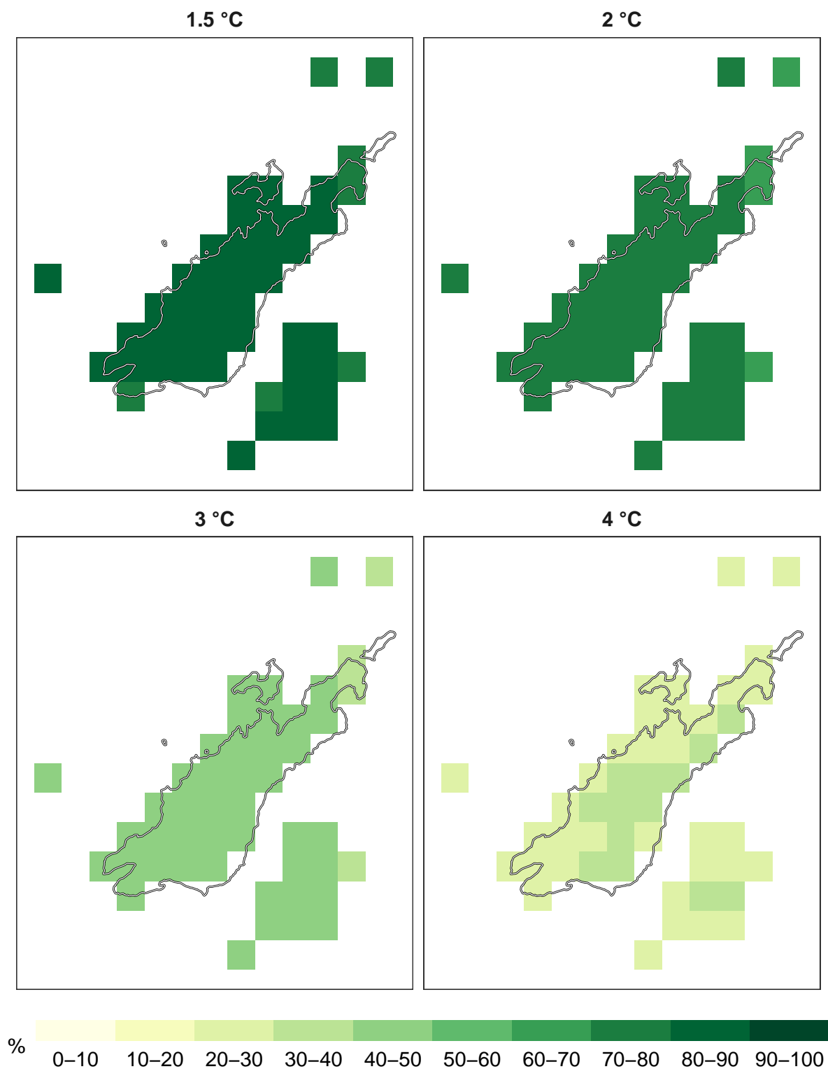
Figure 4: Percent reptiles remaining at 1 km resolution.
