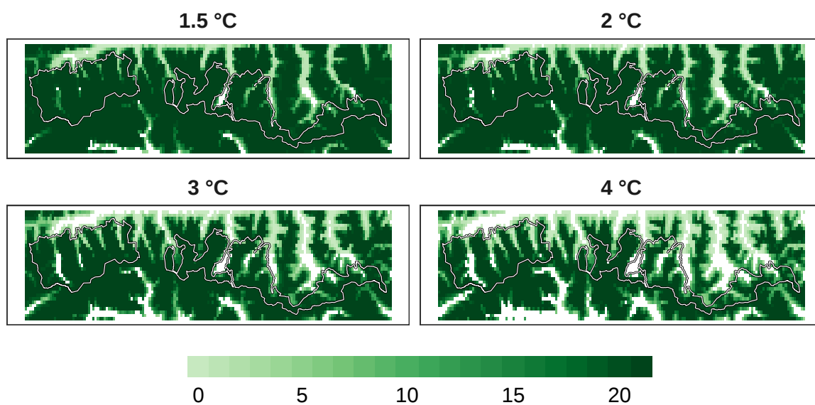
Figure 16: Number of models in agreement for insect refugia at 1 km resolution.
