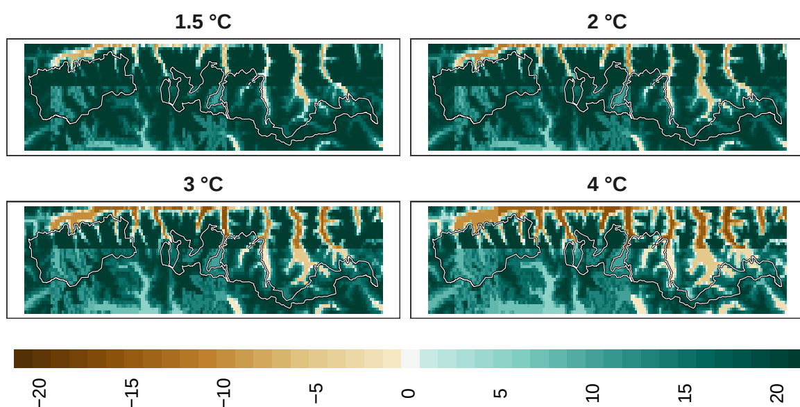
Figure 20: Adaptation effort for amphibians at 1 km resolution.
