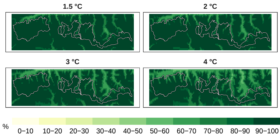
Figure 4: Percent birds remaining at 1 km resolution.
