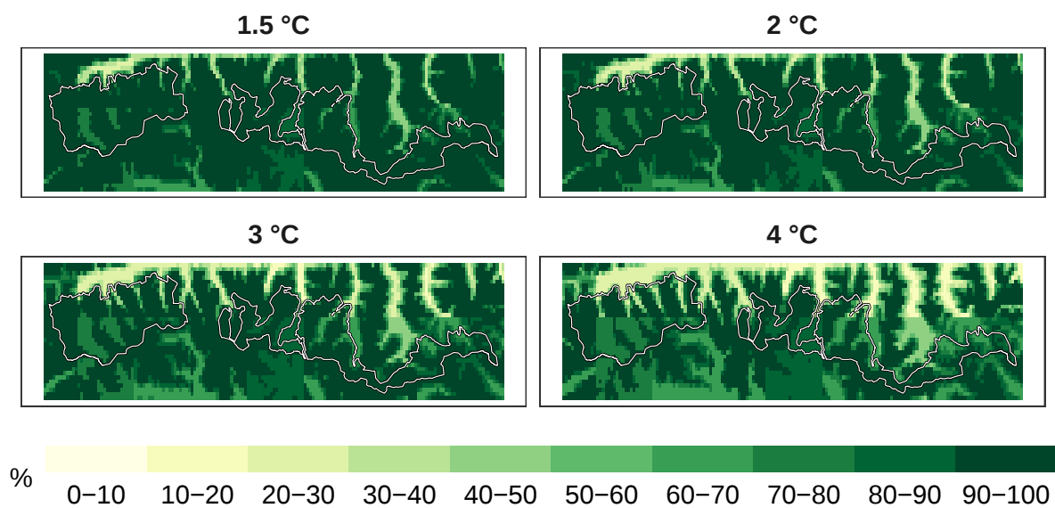
Figure 3: Percent amphibians remaining at 1 km resolution.
