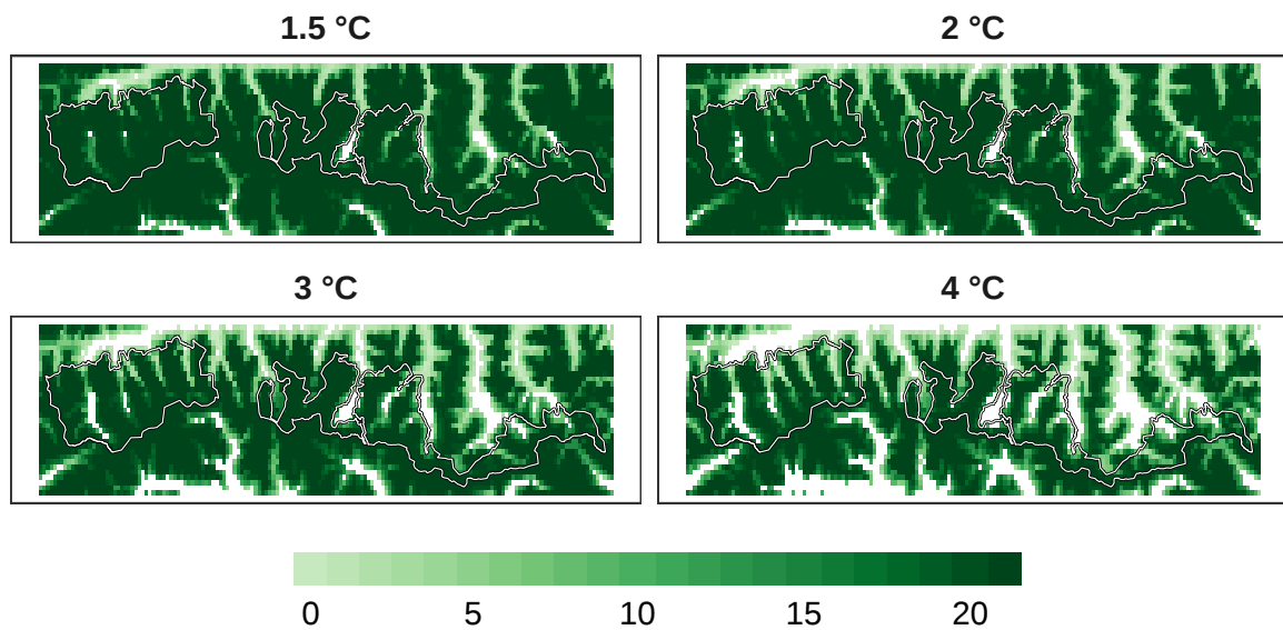
Figure 11: Number of models in agreement for plant refugia at 1 km resolution.
