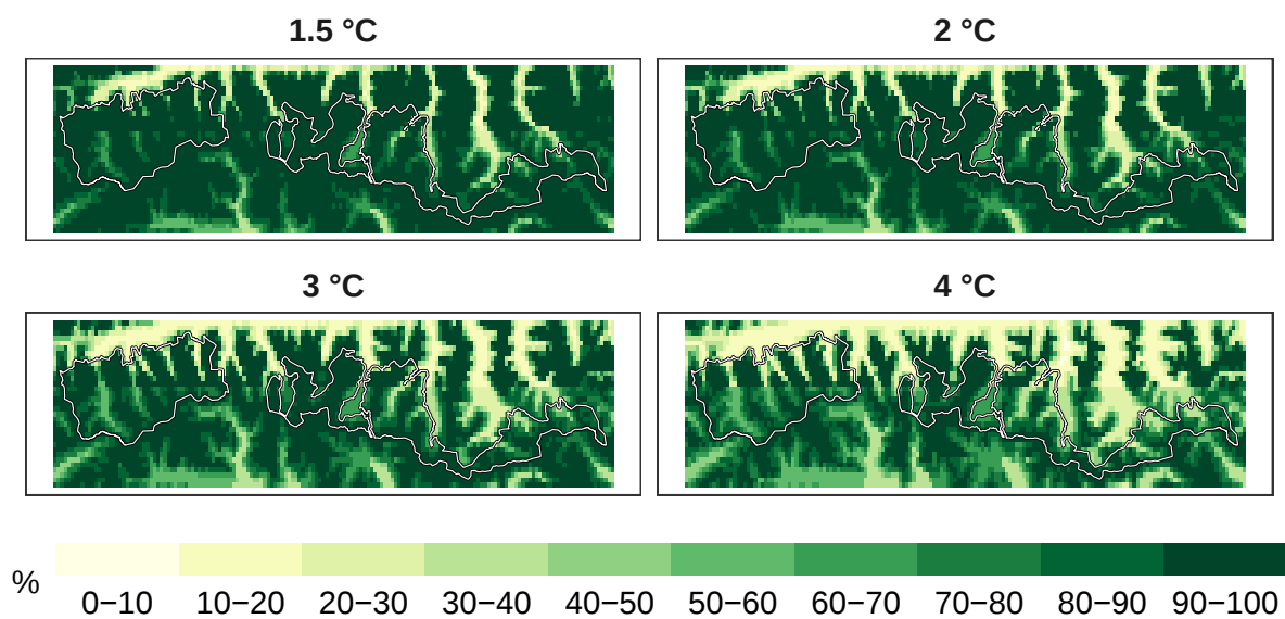
Figure 8: Percent pollinators remaining at 1 km resolution.
