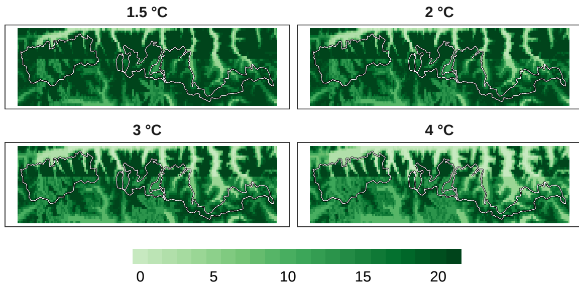
Figure 12: Number of models in agreement for amphibian refugia at 1 km resolution.
