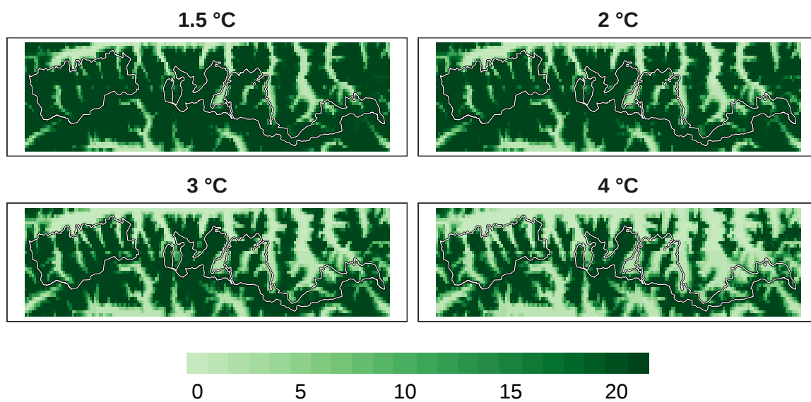
Figure 17: Number of models in agreement for pollinator refugia at 1 km resolution.
