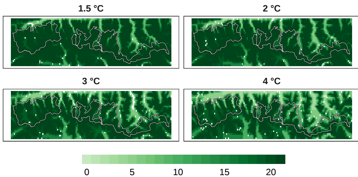
Figure 13: Number of models in agreement for bird refugia.
