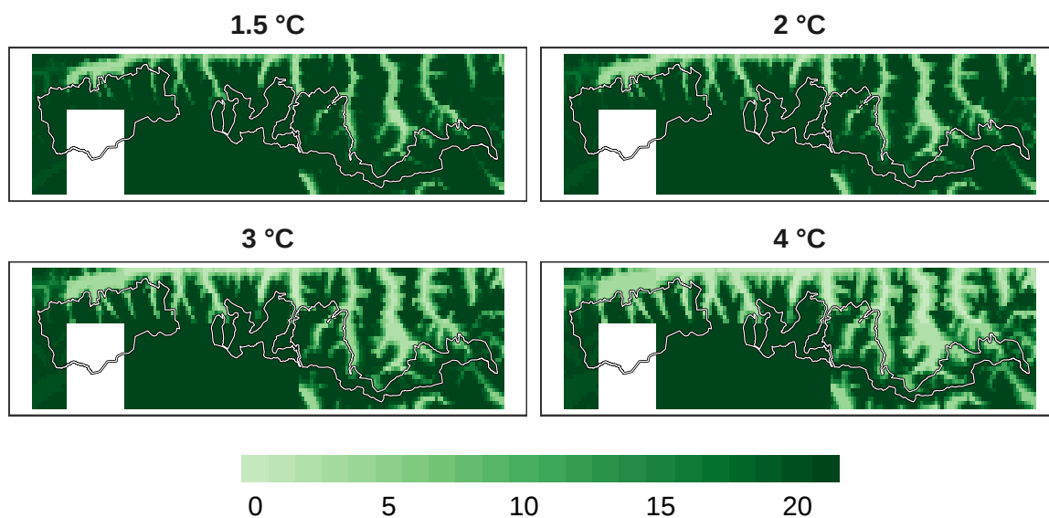
Figure 15: Number of models in agreement for reptile refugia at 1 km resolution.
