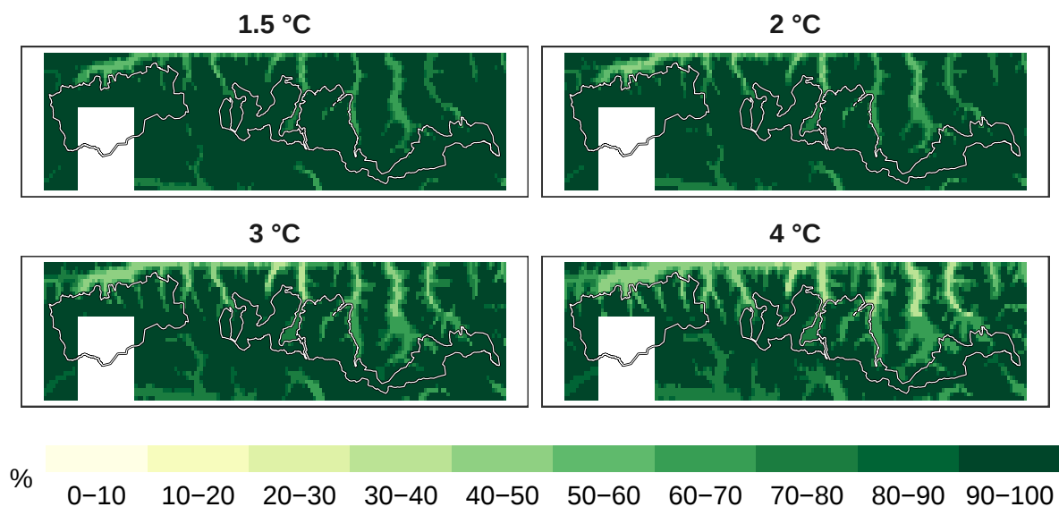
Figure 6: Percent reptiles remaining at 1 km resolution.
