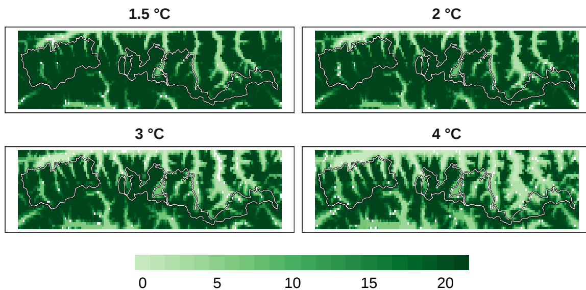
Figure 14: Number of models in agreement for mammal refugia at 1 km resolution.
