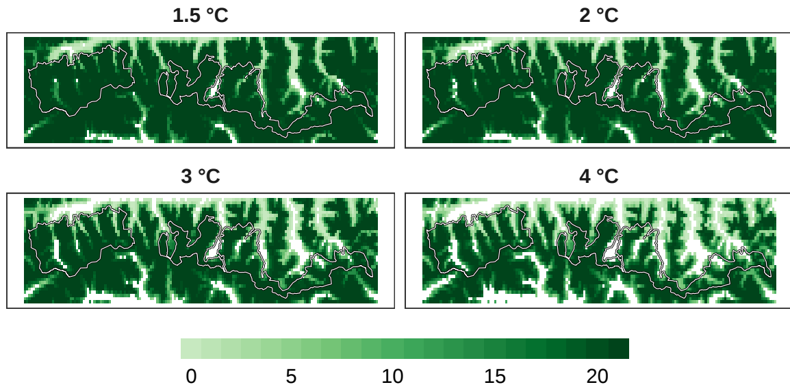
Figure 10: Number of models in agreement for overall biodiversity refugia at 1 km resolution.
