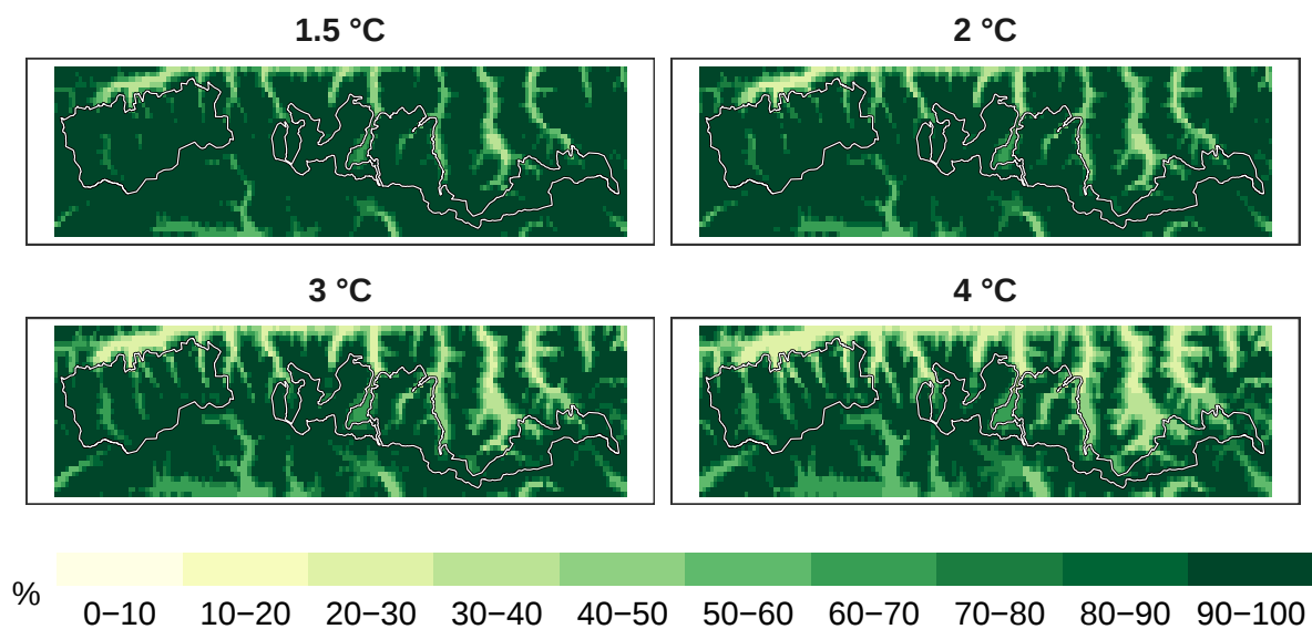
Figure 5: Percent mammals remaining at 1 km resolution.
