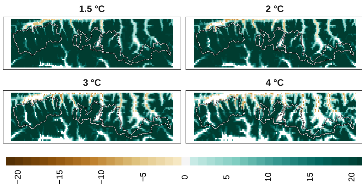
Figure 19: Adaptation effort for plants at 1 km resolution.
