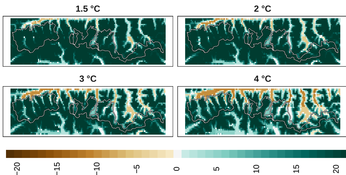
Figure 22: Adaptation effort for mammals at 1 km resolution.
