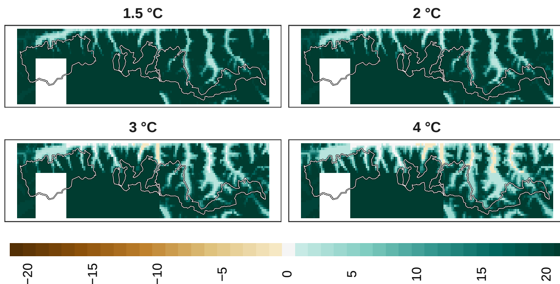
Figure 23: Adaptation effort for reptiles at 1 km resolution.
