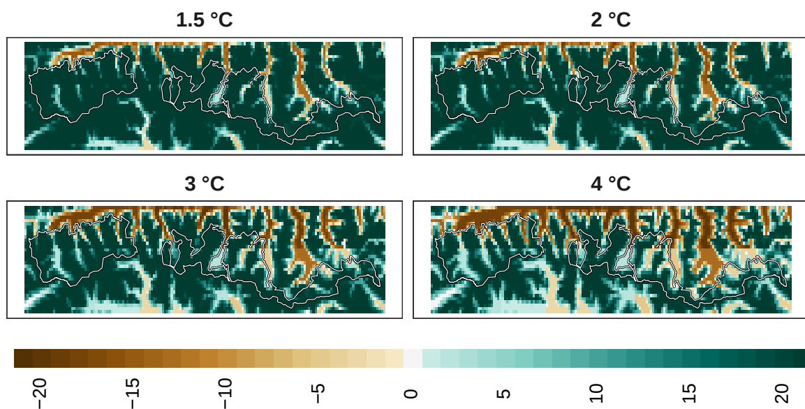
Figure 25: Adaptation effort for pollinators at 1 km resolution.
