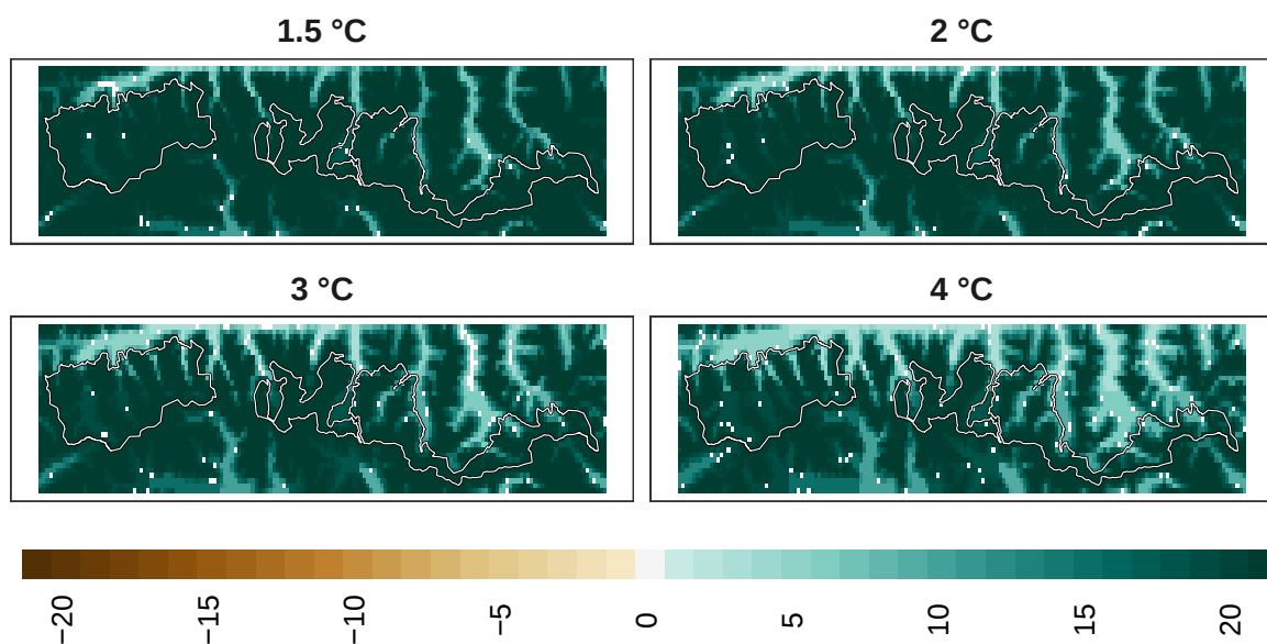
Figure 21: Adaptation effort for birds at 1 km resolution.
