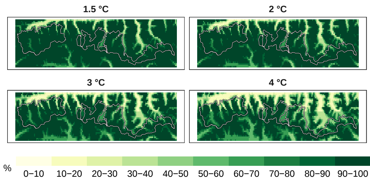
Figure 7: Percent insects remaining at 1 km resolution.
