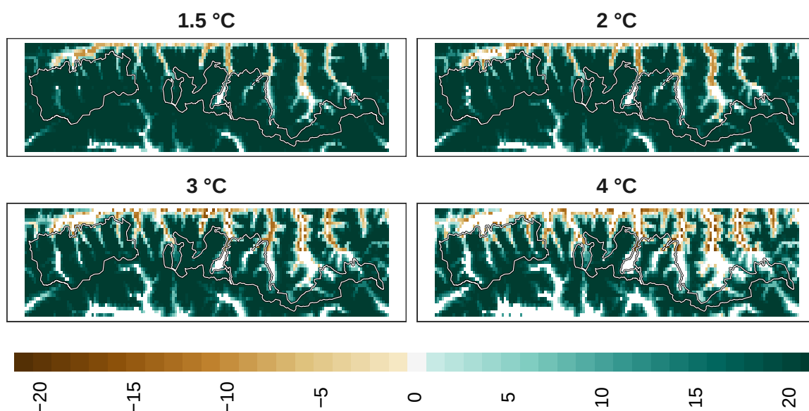
Figure 18: Adaptation effort for overall biodiversity at 1 km resolution.
