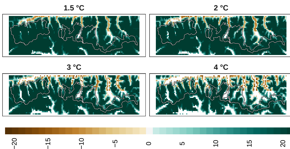
Figure 24: Adaptation effort for insects at 1 km resolution.
