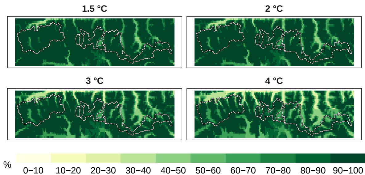
Figure 9: Percent timber species remaining at 1 km resolution.
