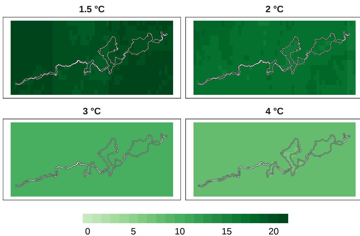
Figure 11: Number of models in agreement for bird refugia.
