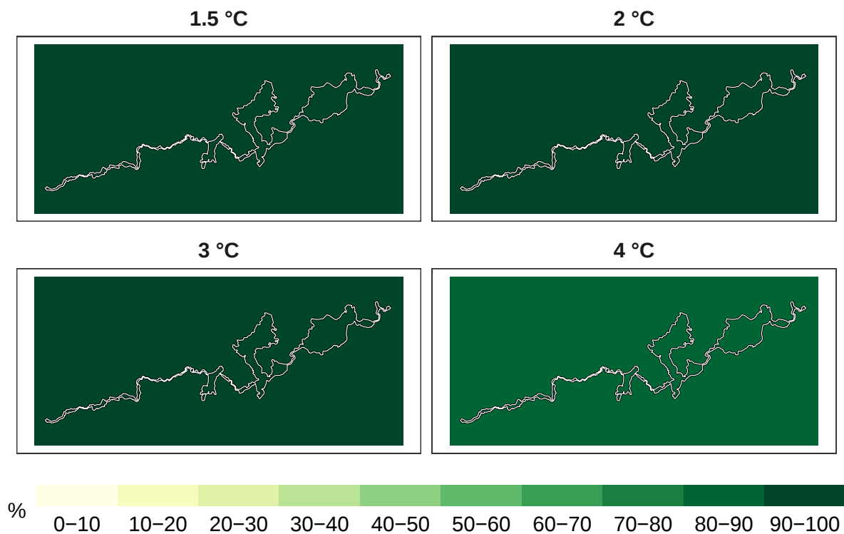
Figure 5: Percent reptiles remaining at 1 km resolution.
