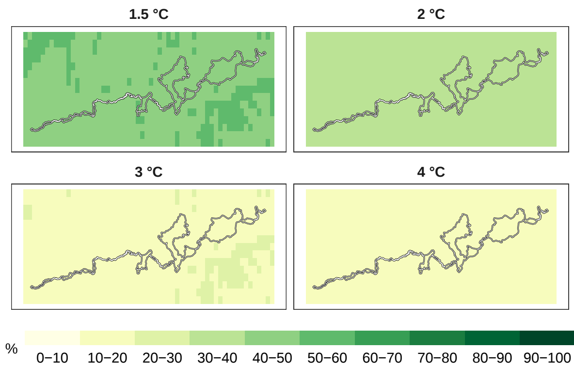
Figure 6: Percent insects remaining at 1 km resolution.
