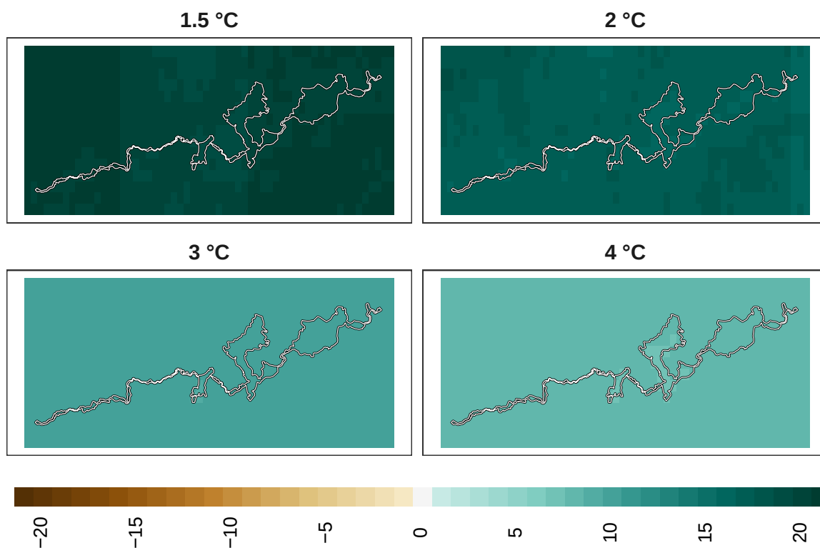
Figure 18: Adaptation effort for birds at 1 km resolution.
