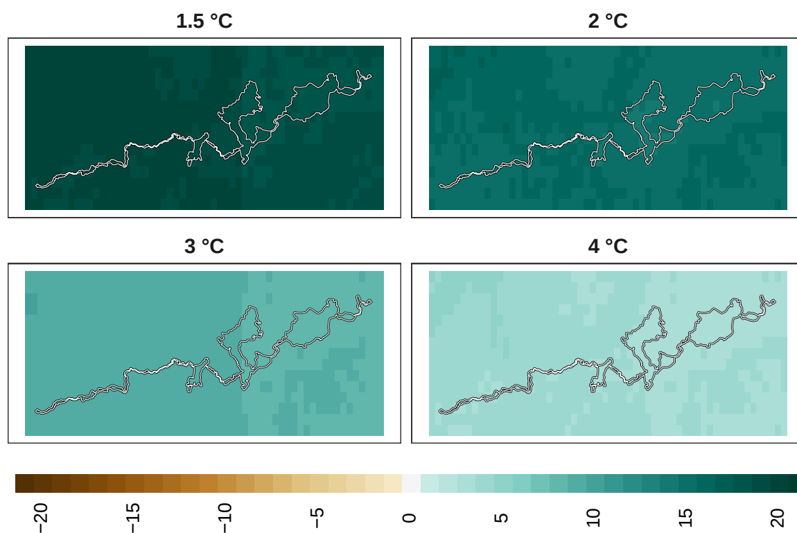
Figure 19: Adaptation effort for mammals at 1 km resolution.
