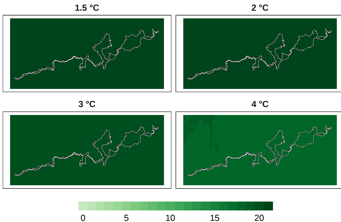
Figure 13: Number of models in agreement for reptile refugia at 1 km resolution.
