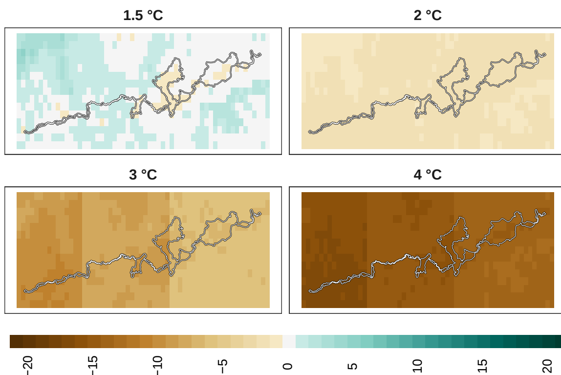
Figure 16: Adaptation effort for overall biodiversity at 1 km resolution.
