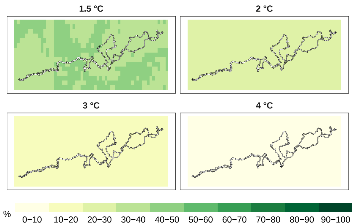
Figure 7: Percent pollinators remaining at 1 km resolution.
