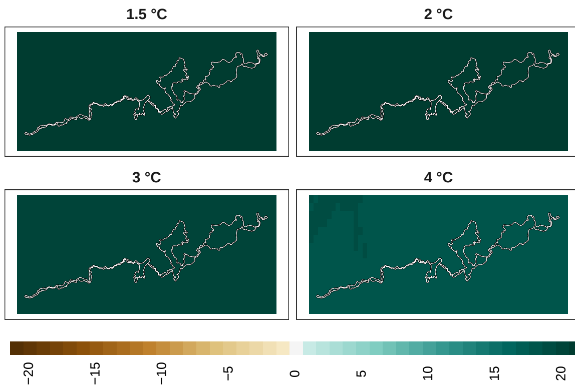
Figure 20: Adaptation effort for reptiles at 1 km resolution.
