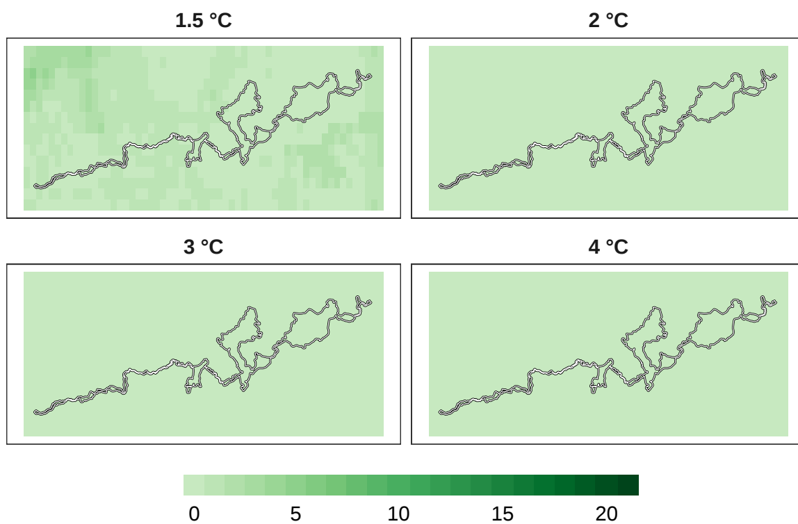
Figure 15: Number of models in agreement for pollinator refugia at 1 km resolution.
