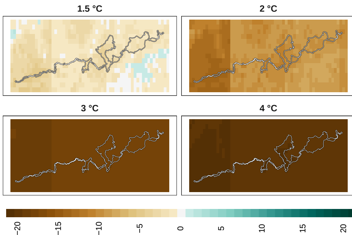
Figure 22: Adaptation effort for pollinators at 1 km resolution.
