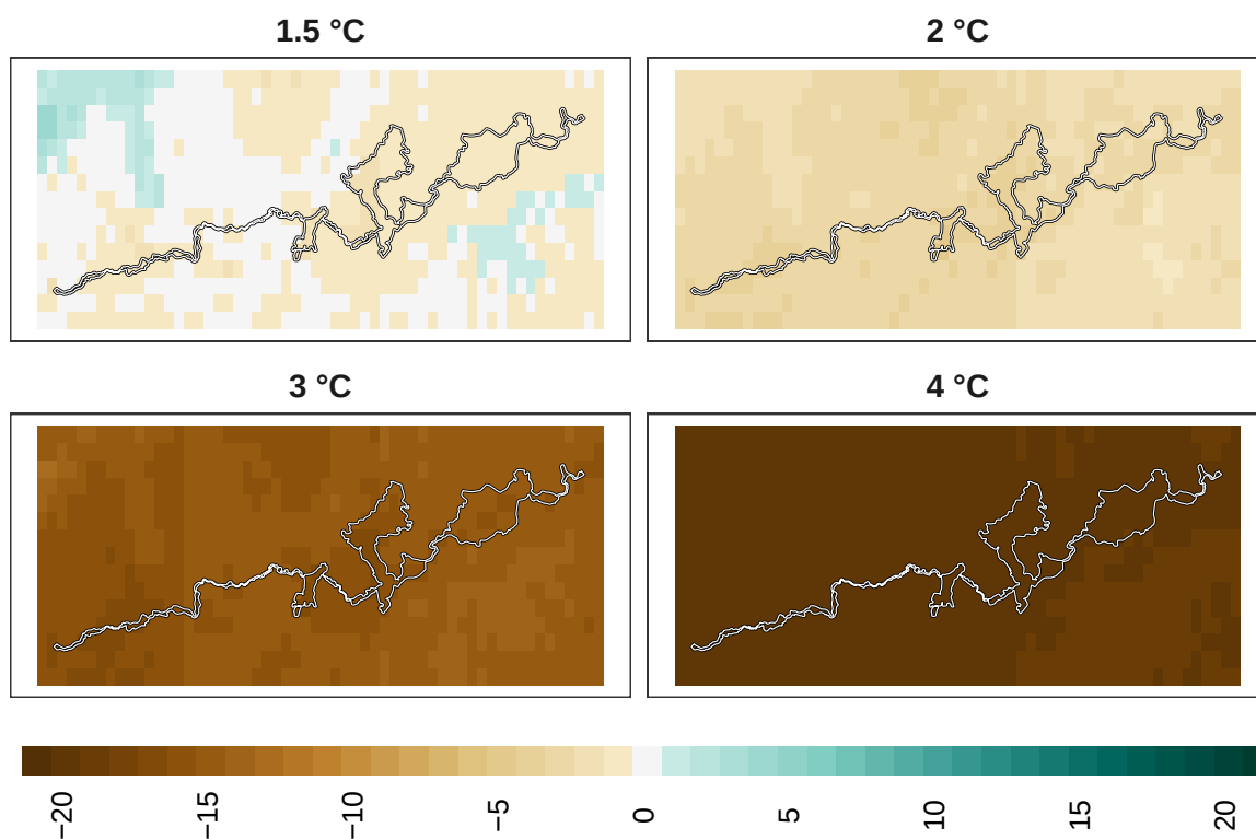
Figure 21: Adaptation effort for insects at 1 km resolution.
