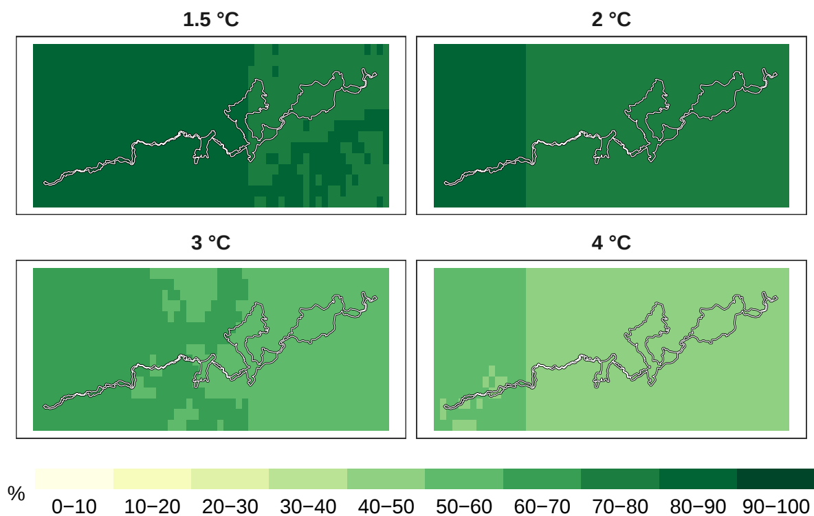
Figure 8: Percent timber species remaining at 1 km resolution.
