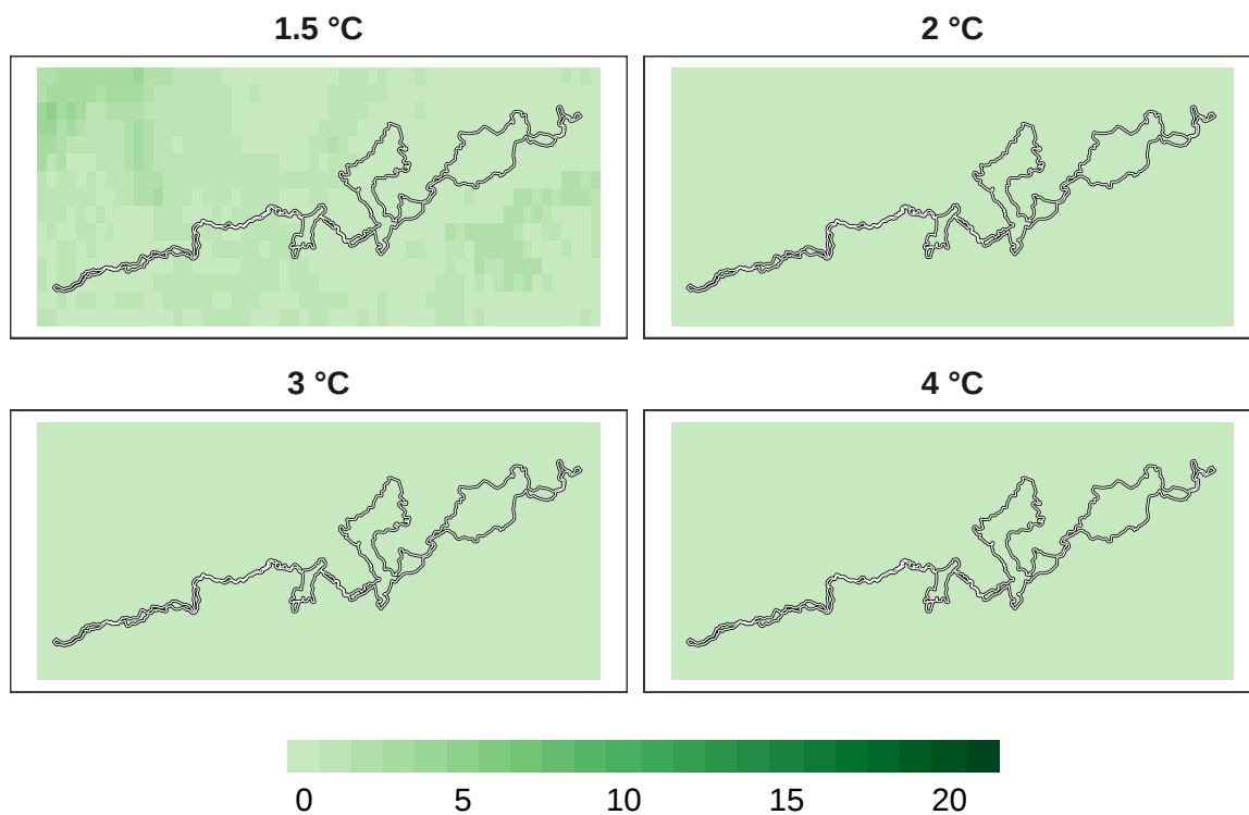
Figure 9: Number of models in agreement for overall biodiversity refugia at 1 km resolution.
