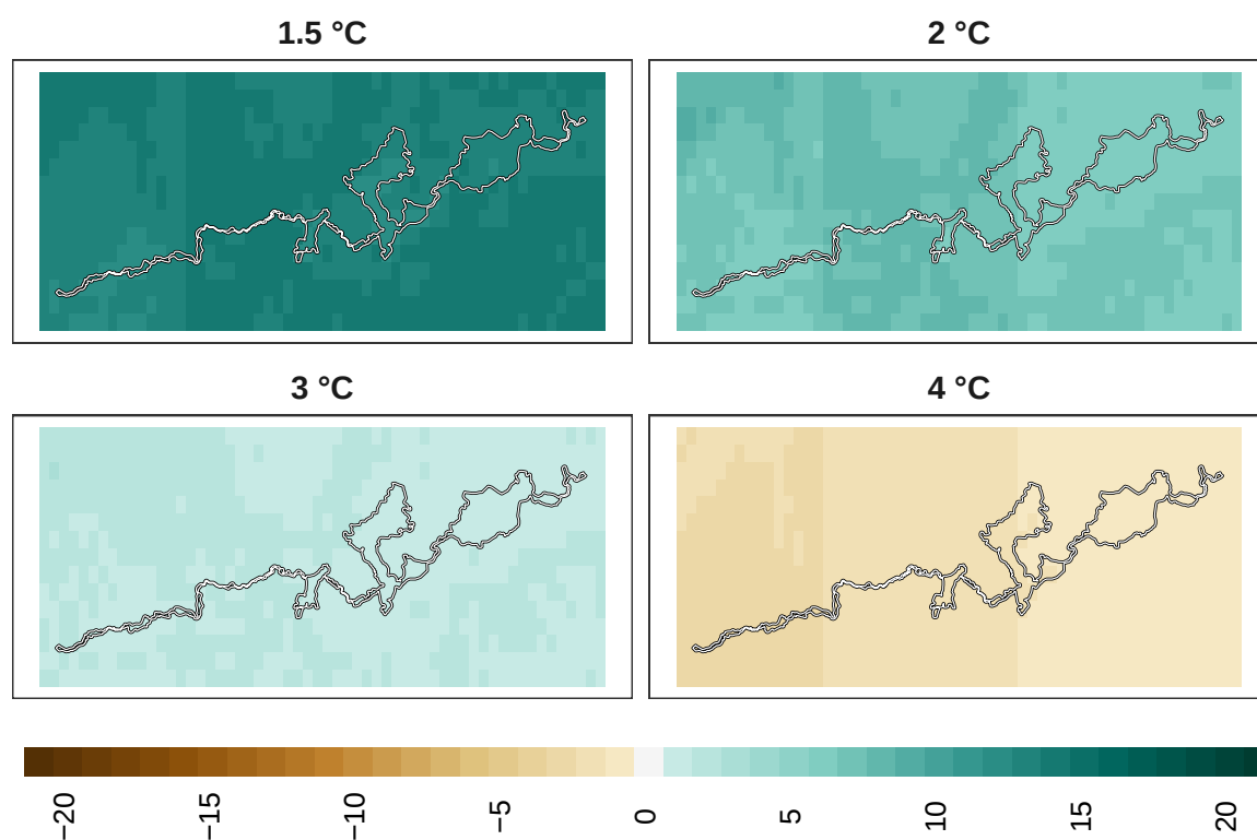
Figure 17: Adaptation effort for plants at 1 km resolution.
