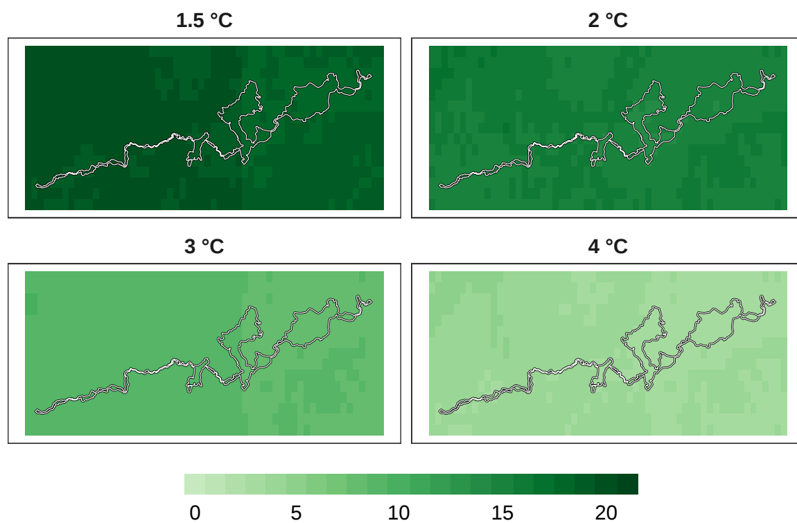
Figure 12: Number of models in agreement for mammal refugia at 1 km resolution.
