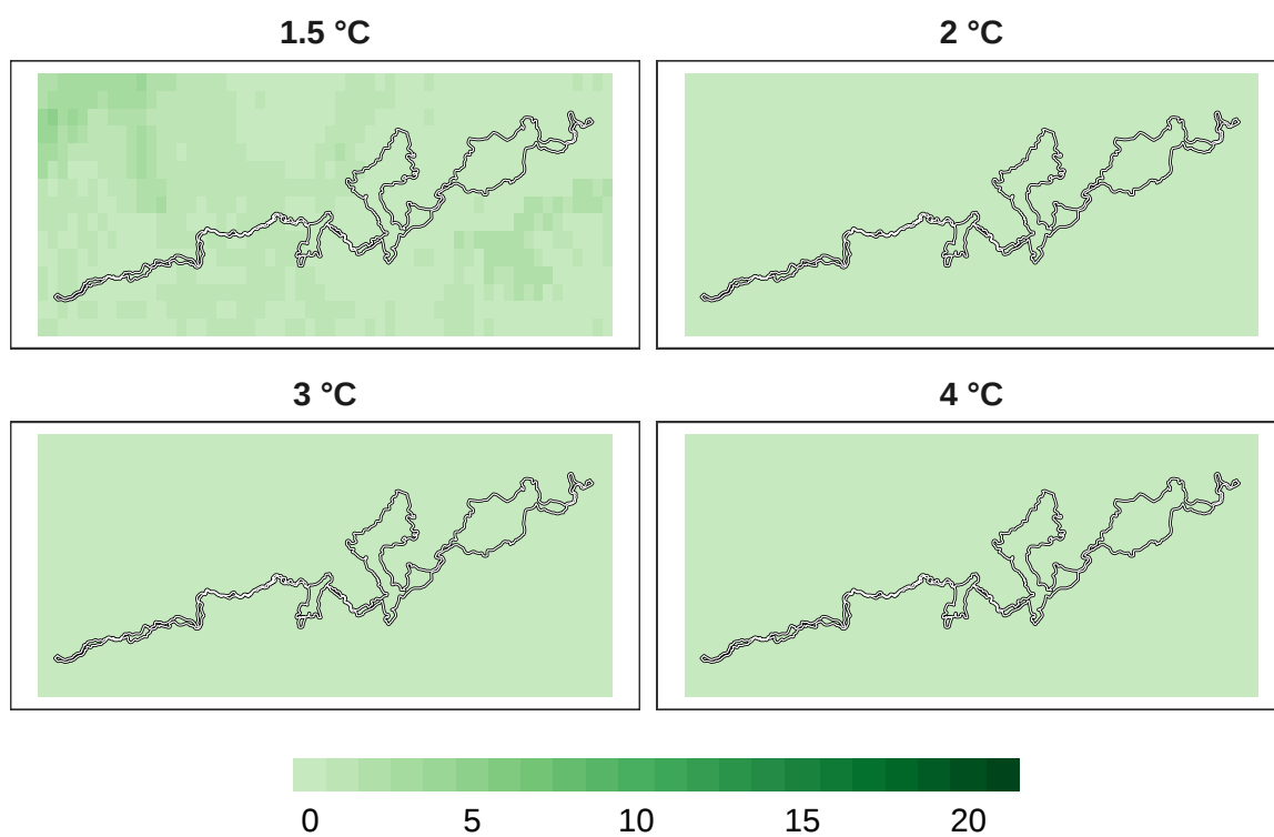
Figure 14: Number of models in agreement for insect refugia at 1 km resolution.
