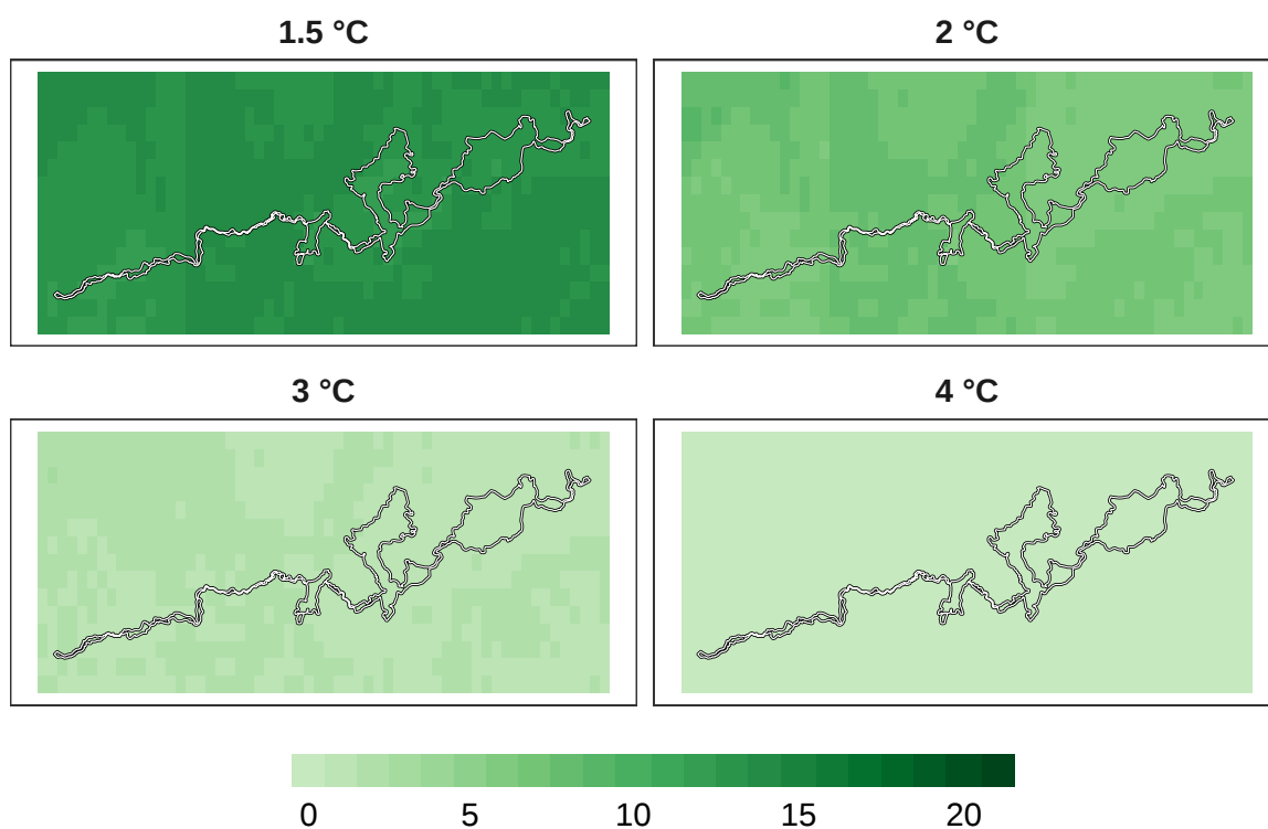
Figure 10: Number of models in agreement for plant refugia at 1 km resolution.
