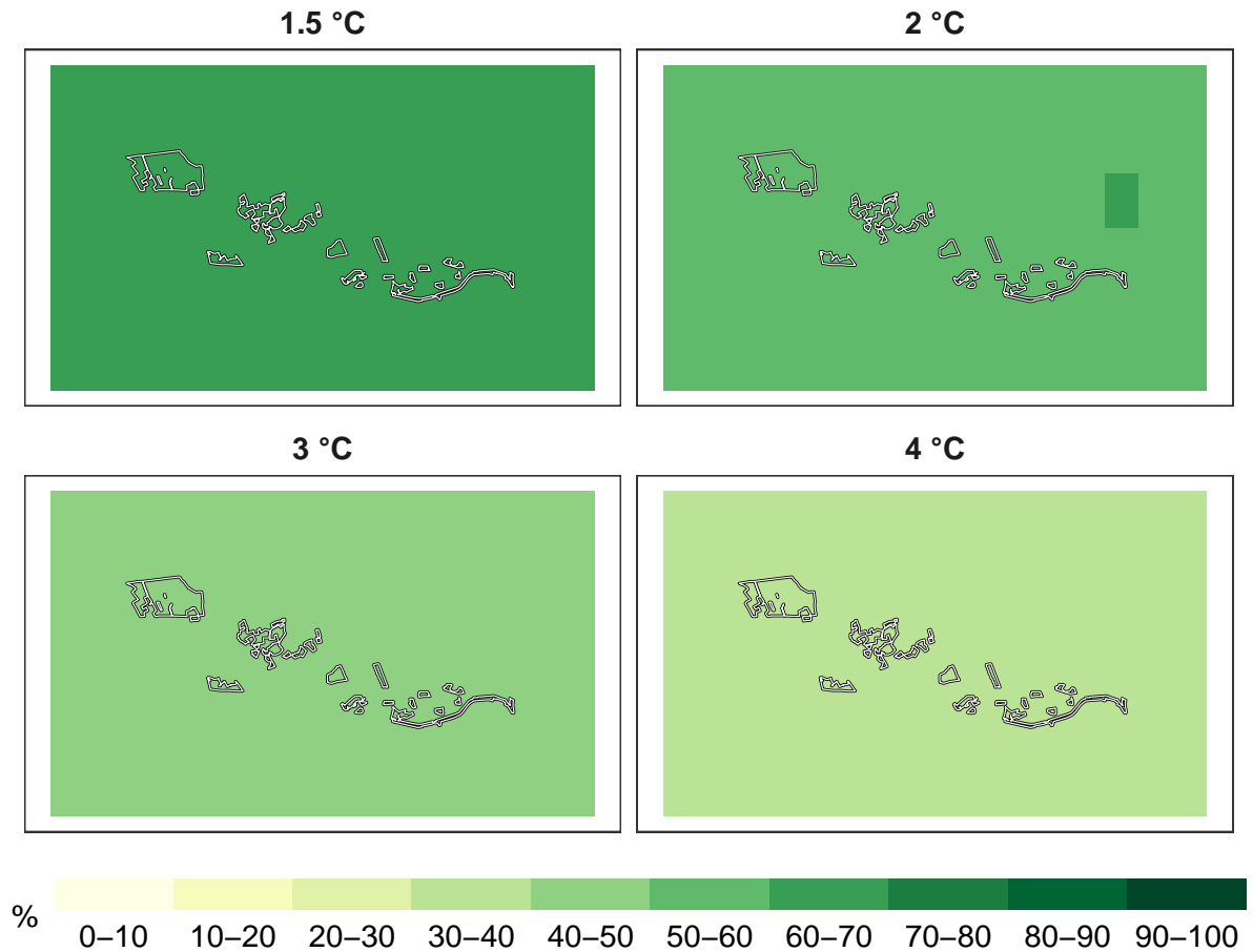
Figure 1: Percent overall biodiversity remaining at 1 km resolution.
