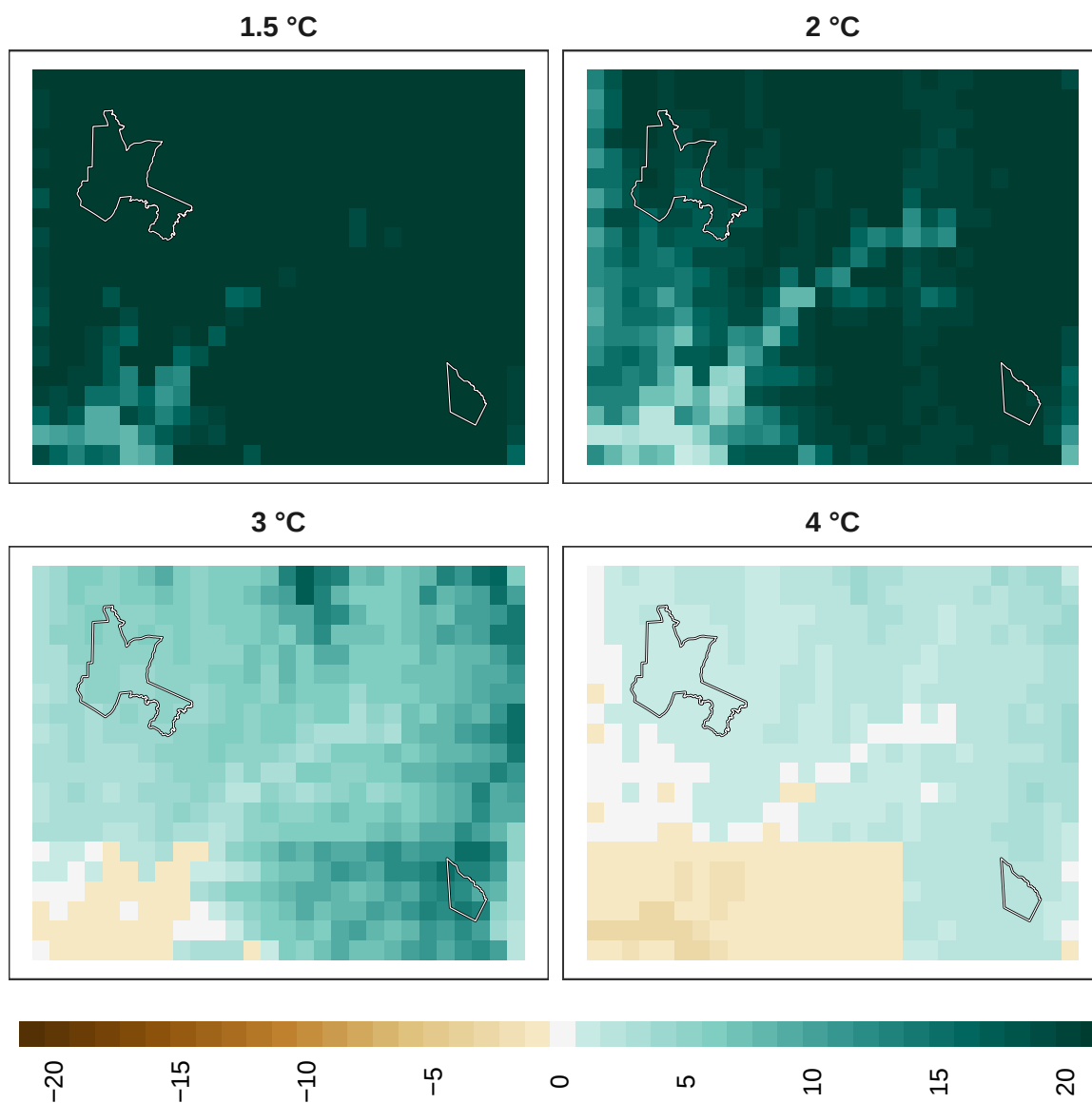
Figure 25: Adaptation effort for pollinators at 1 km resolution.
