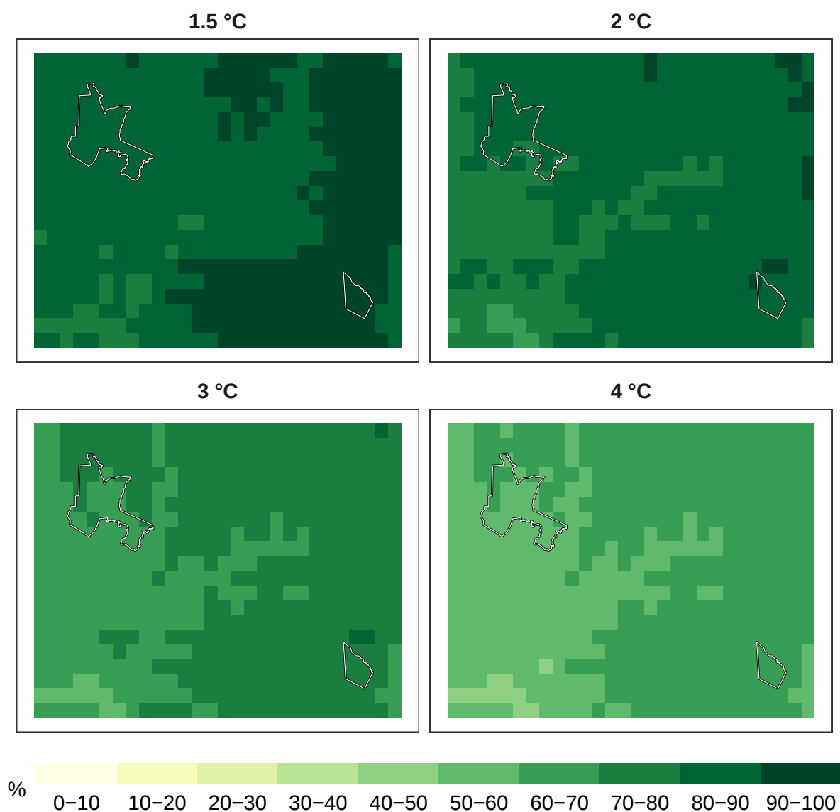
Figure 7: Percent insects remaining at 1 km resolution.
