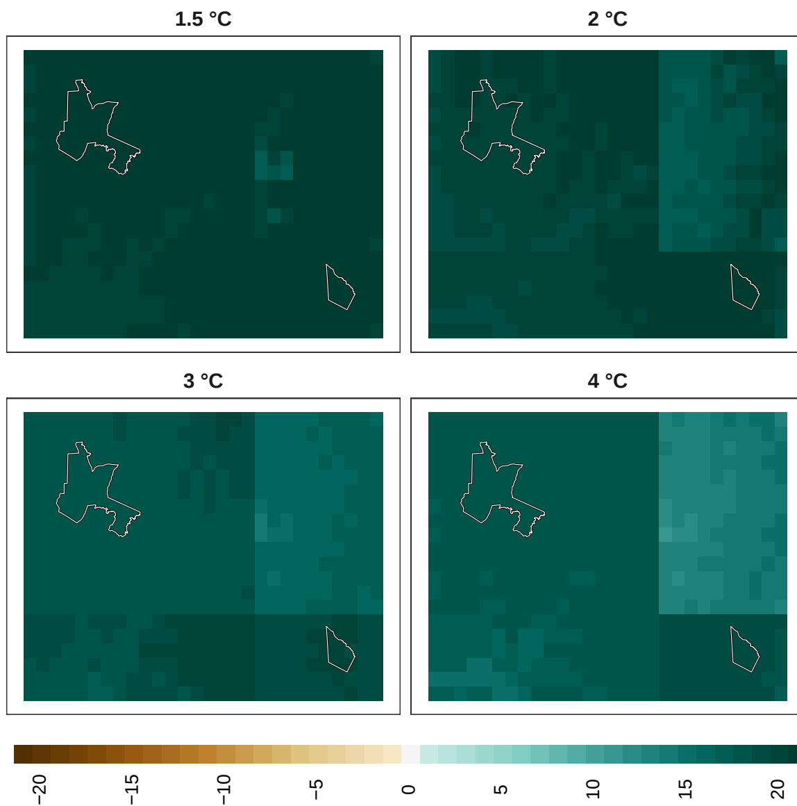
Figure 23: Adaptation effort for reptiles at 1 km resolution.
