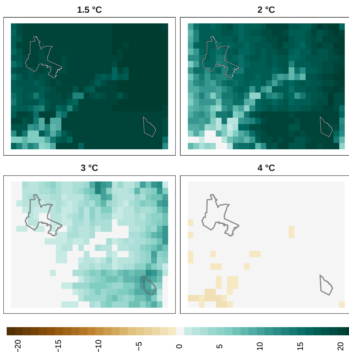
Figure 18: Adaptation effort for overall biodiversity at 1 km resolution.
