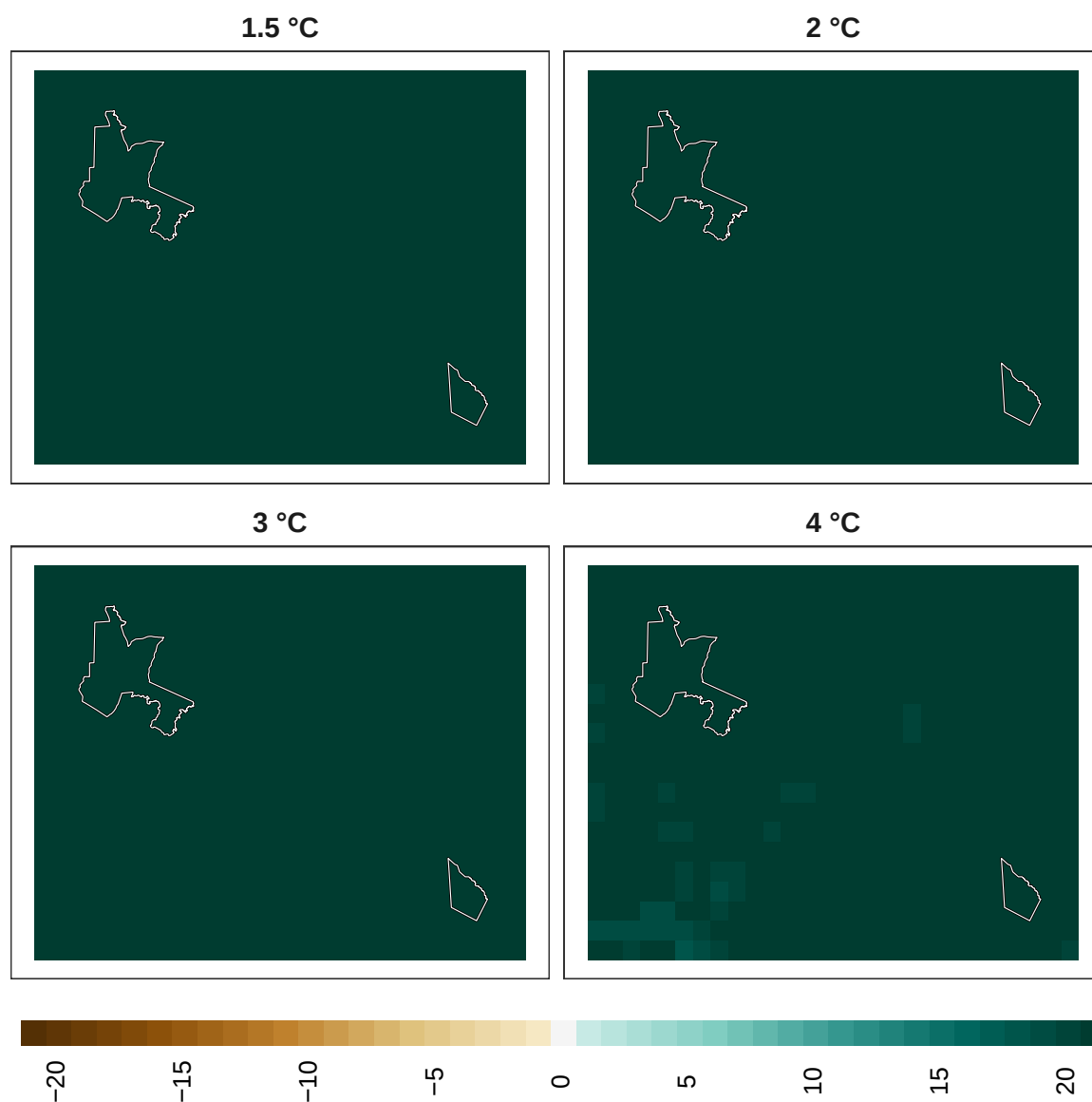
Figure 20: Adaptation effort for amphibians at 1 km resolution.
