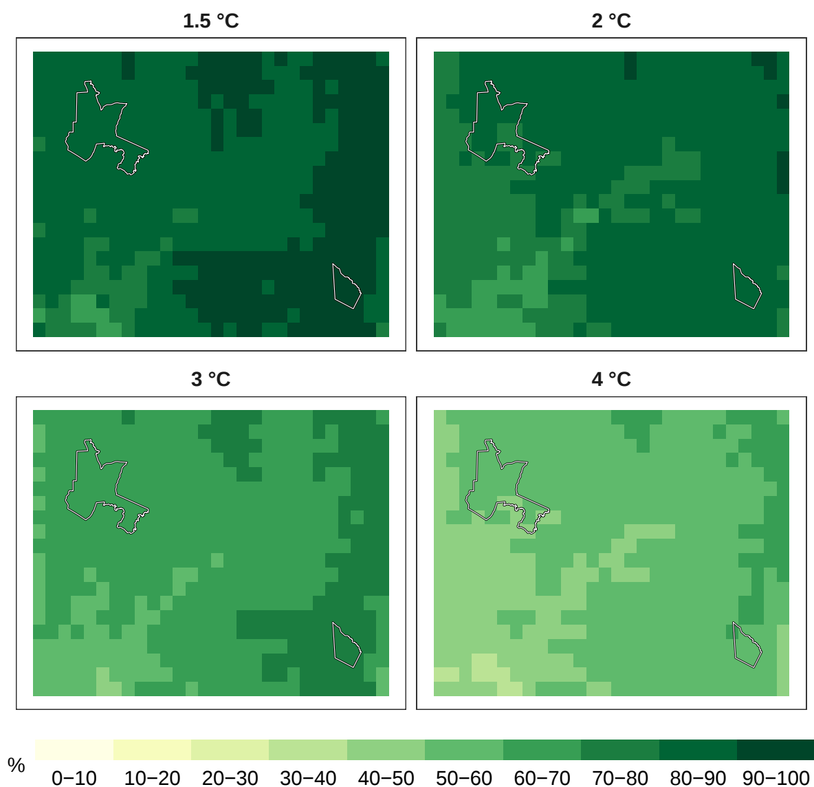
Figure 8: Percent pollinators remaining at 1 km resolution.
