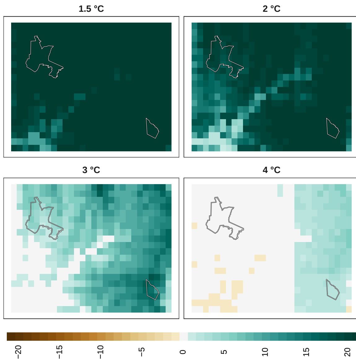
Figure 24: Adaptation effort for insects at 1 km resolution.
