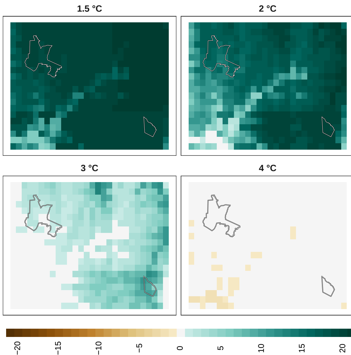
Figure 19: Adaptation effort for plants at 1 km resolution.
