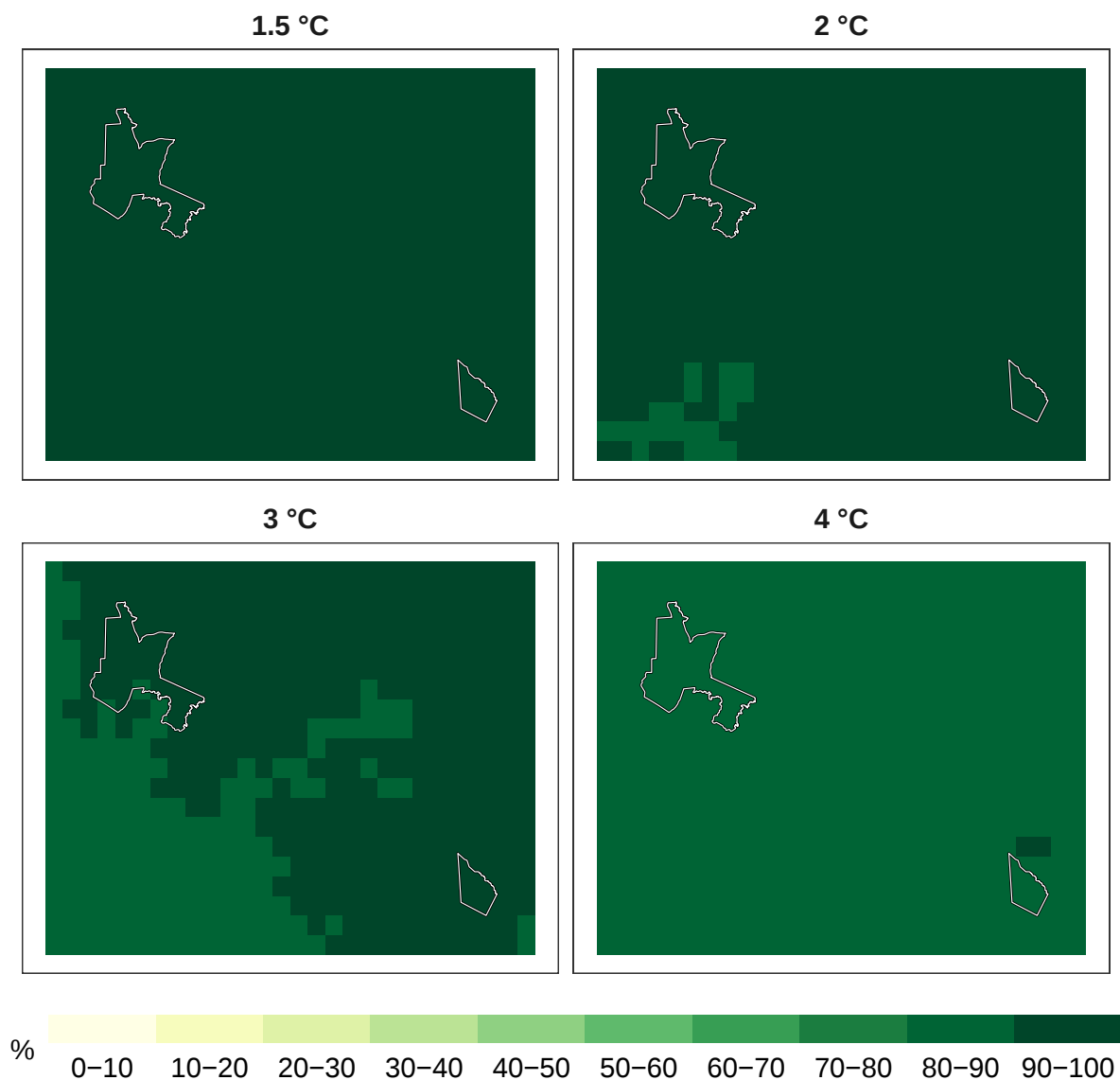
Figure 5: Percent mammals remaining at 1 km resolution.
