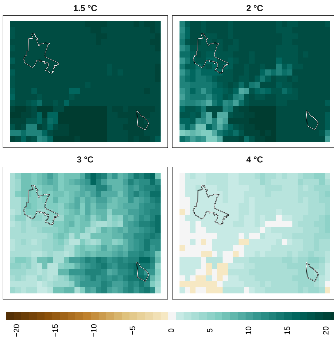
Figure 21: Adaptation effort for birds at 1 km resolution.
