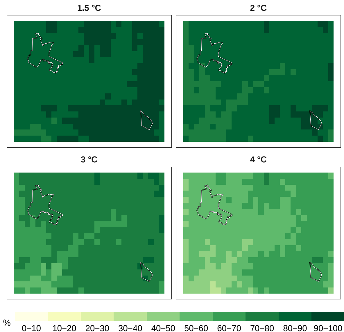
Figure 4: Percent birds remaining at 1 km resolution.
