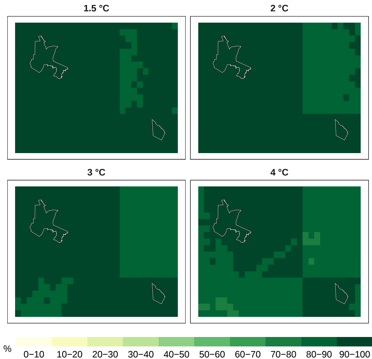
Figure 6: Percent reptiles remaining at 1 km resolution.
