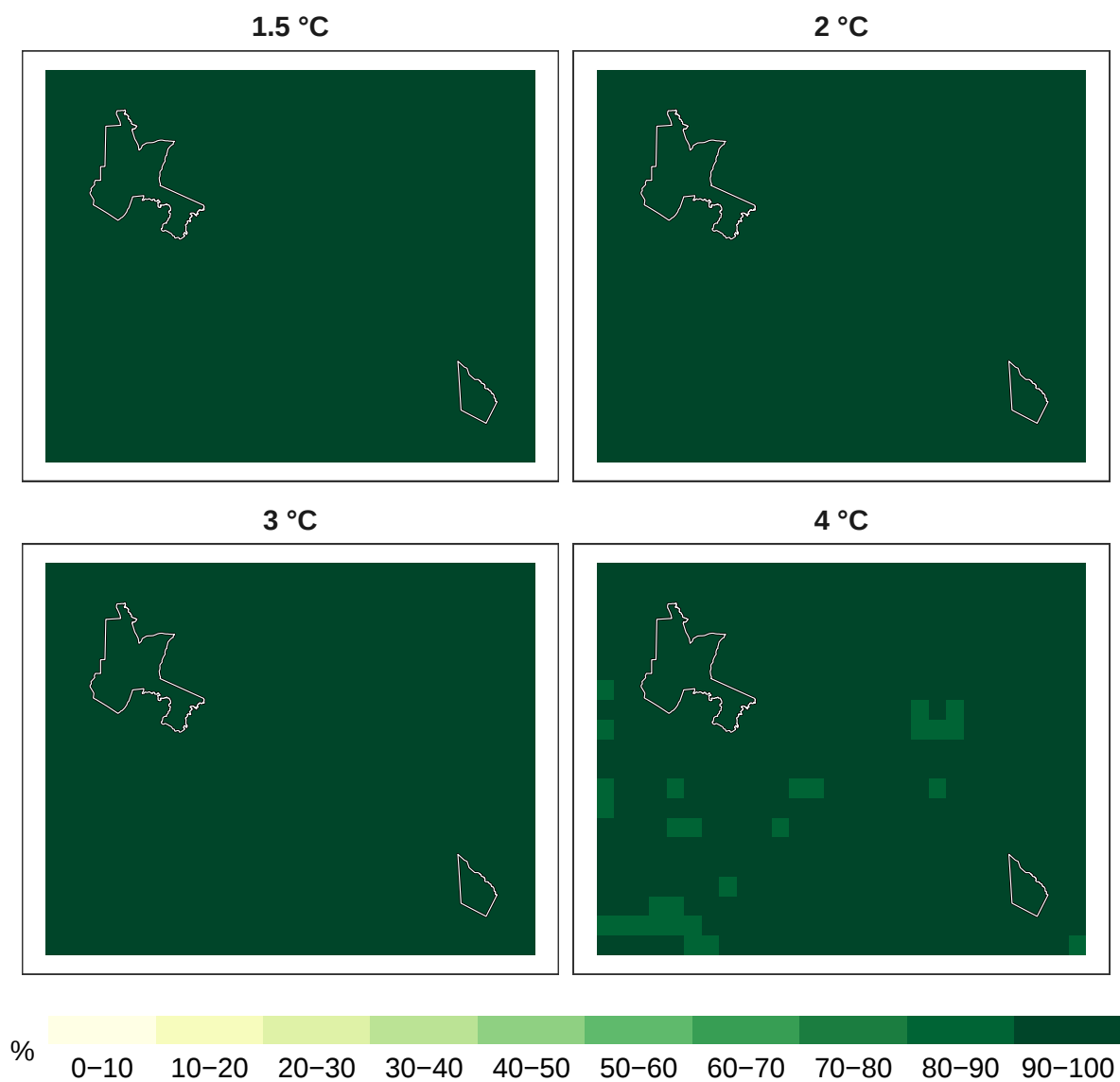
Figure 3: Percent amphibians remaining at 1 km resolution.
