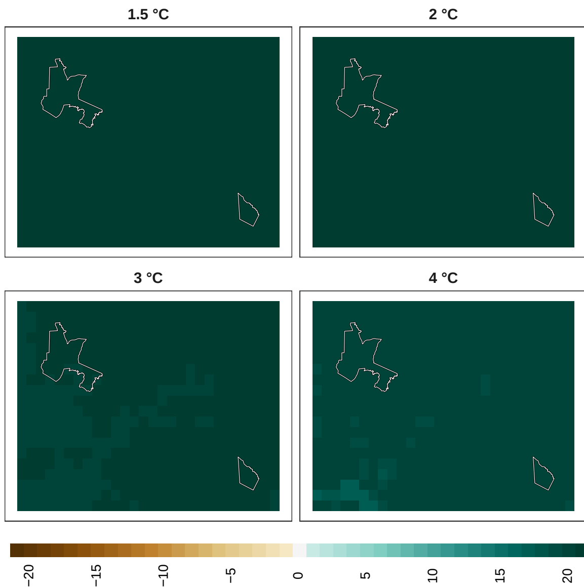
Figure 22: Adaptation effort for mammals at 1 km resolution.
