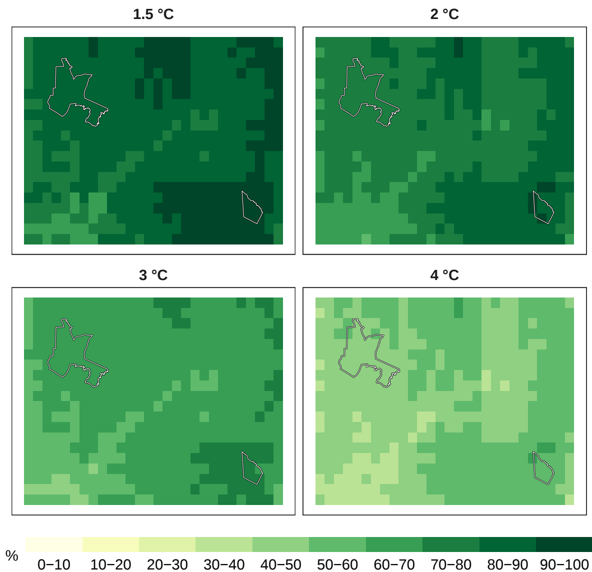
Figure 9: Percent timber species remaining at 1 km resolution.
