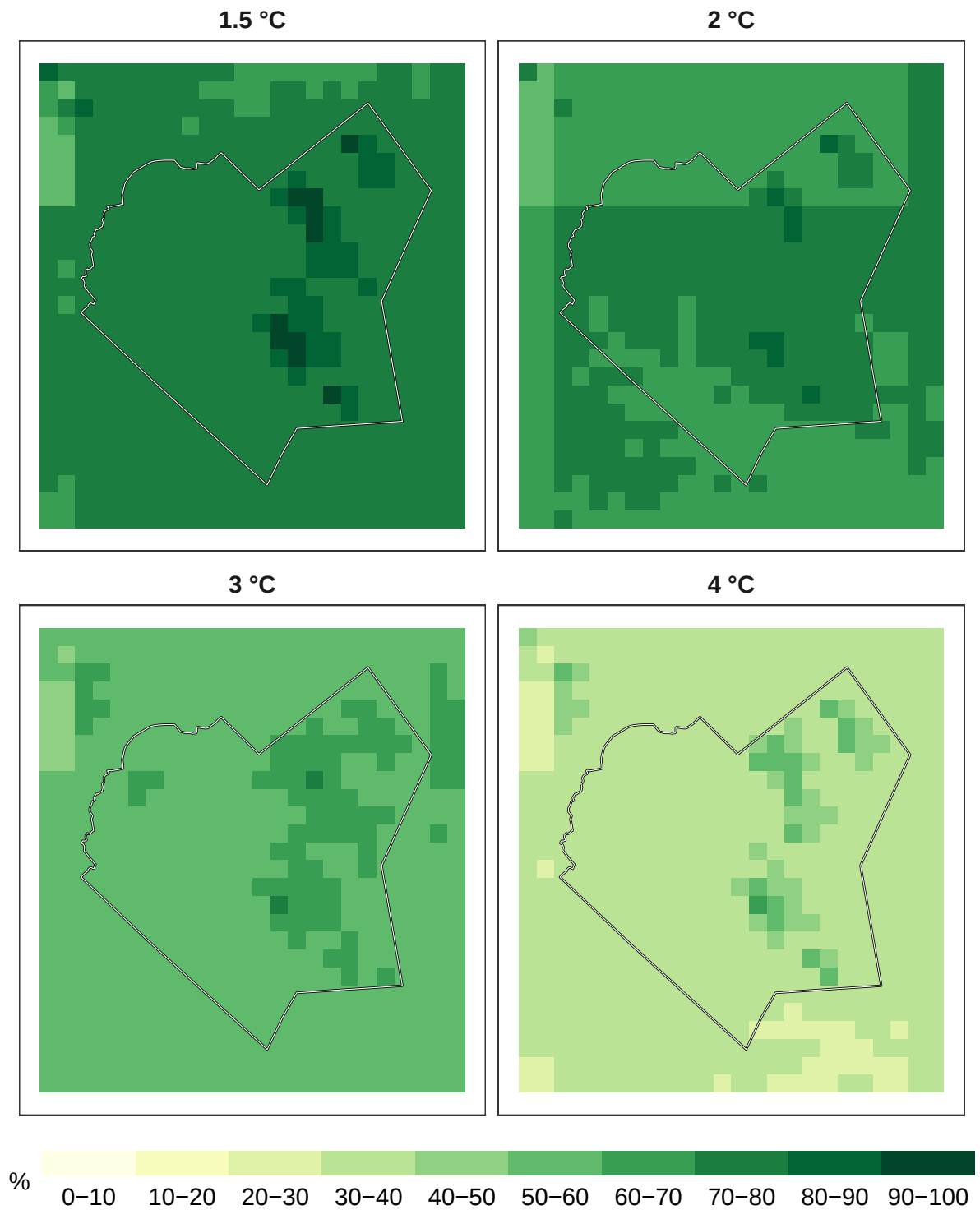
Figure 5: Percent mammals remaining at 1 km resolution.
