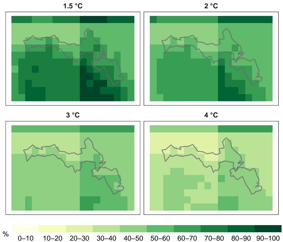
Figure 7: Percent pollinators remaining at 1 km resolution.
