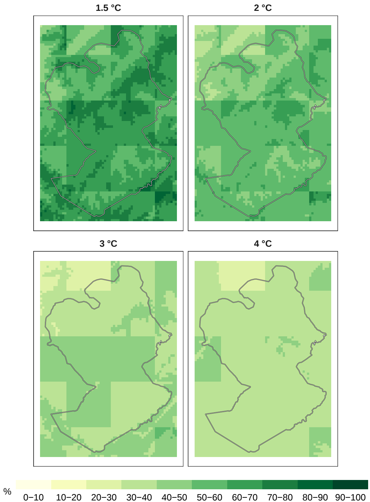
Figure 3: Percent birds remaining at 1 km resolution.
