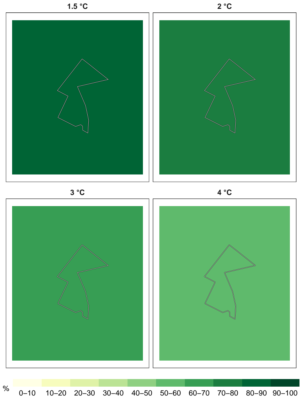
Figure 6: Percent insects remaining at 1 km resolution.
