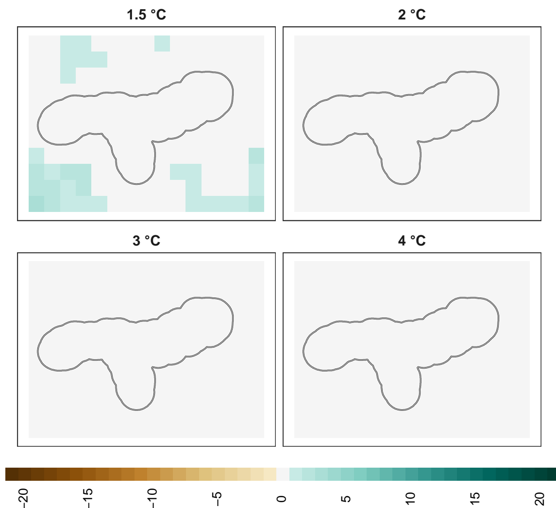
Figure 16: Adaptation effort for amphibians at 1 km resolution.
