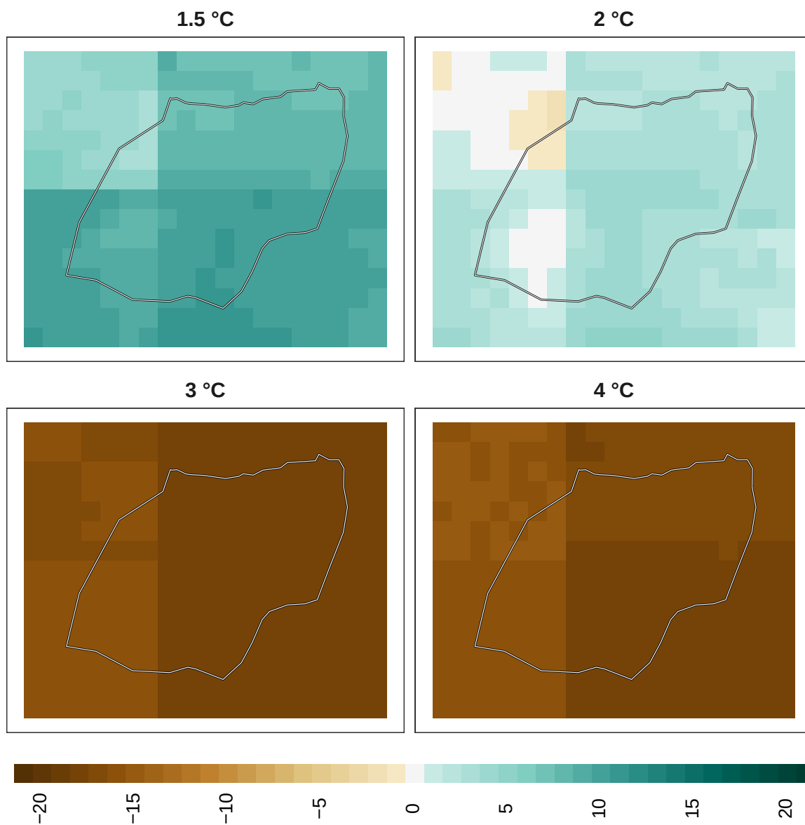
Figure 18: Adaptation effort for reptiles at 1 km resolution.
