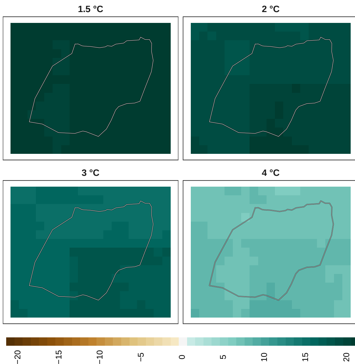
Figure 19: Adaptation effort for insects at 1 km resolution.
