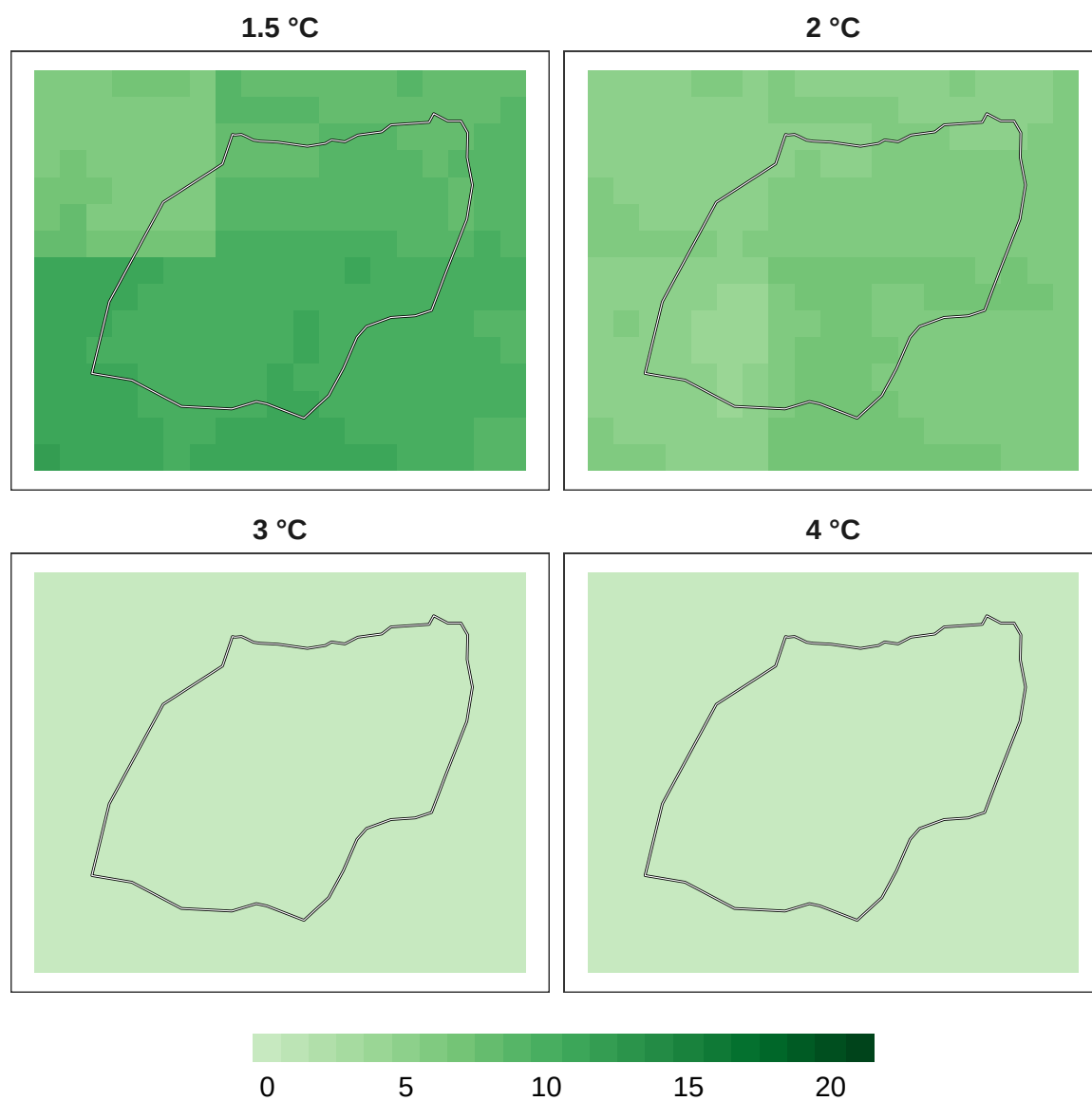
Figure 12: Number of models in agreement for reptile refugia at 1 km resolution.
