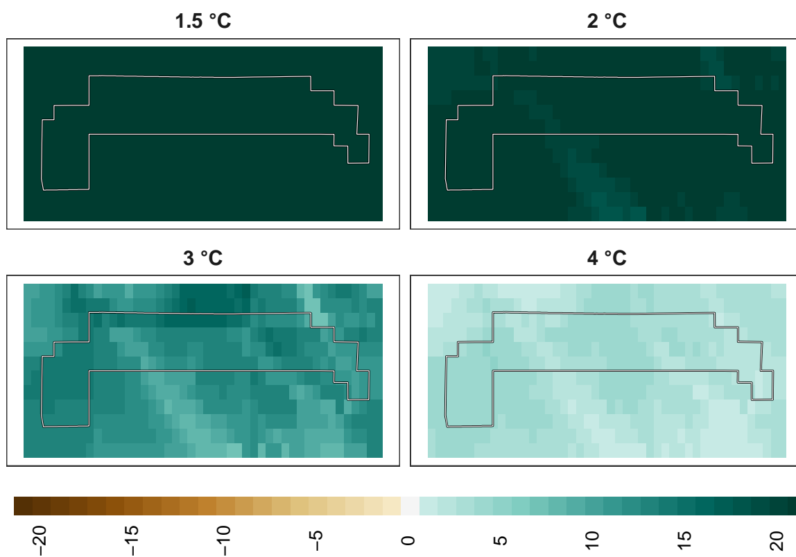
Figure 17: Adaptation effort for insects at 1 km resolution.
