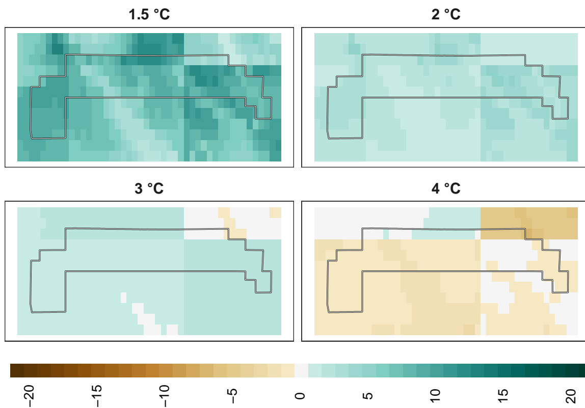
Figure 18: Adaptation effort for pollinators at 1 km resolution.
