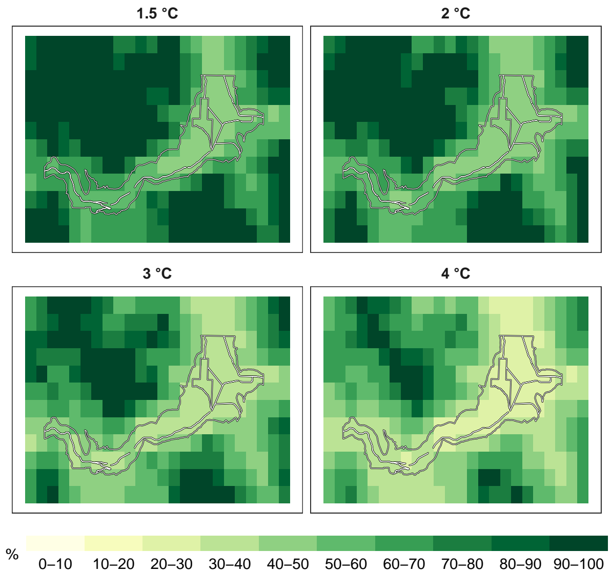
Figure 7: Percent pollinators remaining at 1 km resolution.
