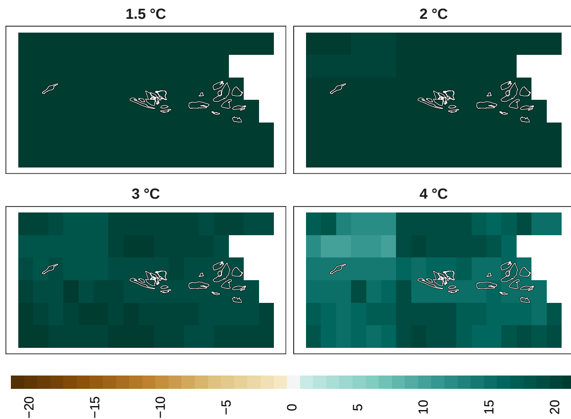
Figure 18: Adaptation effort for amphibians at 1 km resolution.
