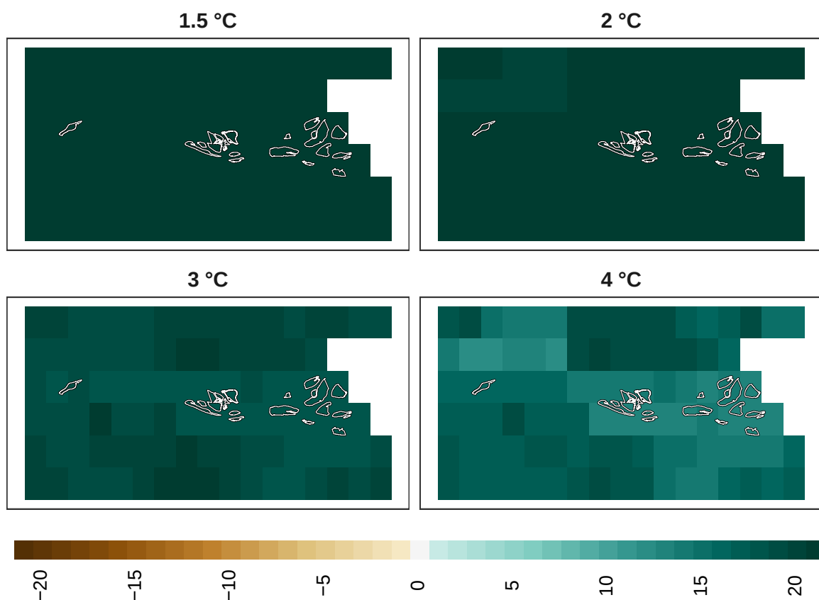
Figure 22: Adaptation effort for pollinators at 1 km resolution.
