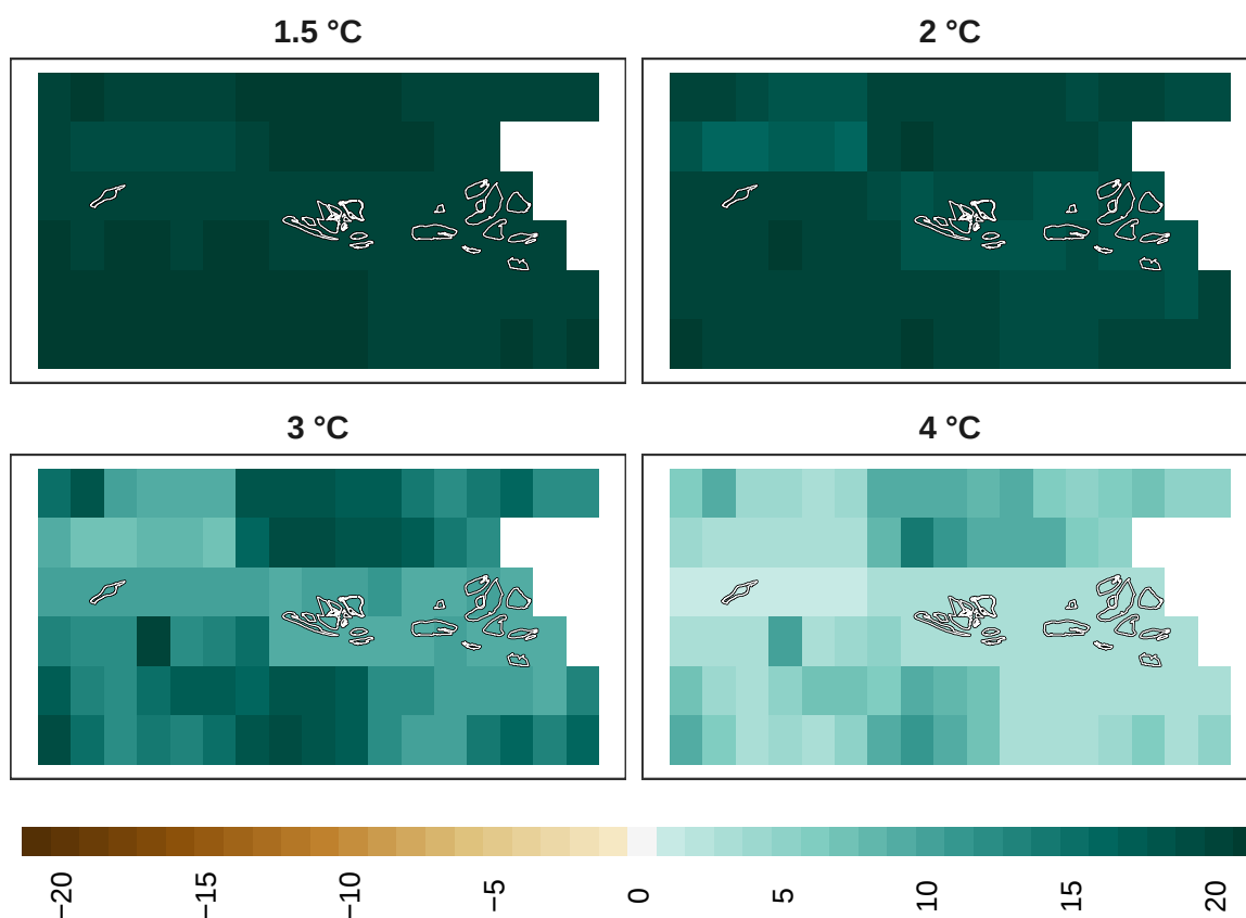
Figure 21: Adaptation effort for insects at 1 km resolution.
