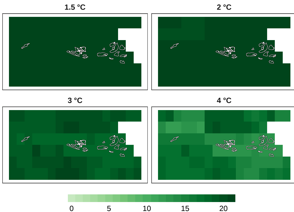
Figure 15: Number of models in agreement for pollinator refugia at 1 km resolution.
