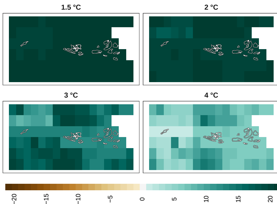
Figure 16: Adaptation effort for overall biodiversity at 1 km resolution.
