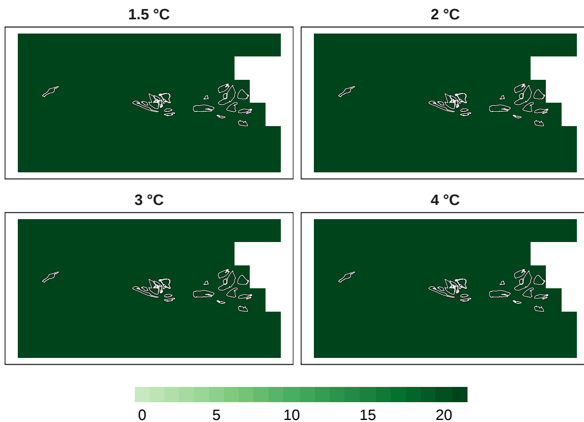
Figure 12: Number of models in agreement for bird refugia.
