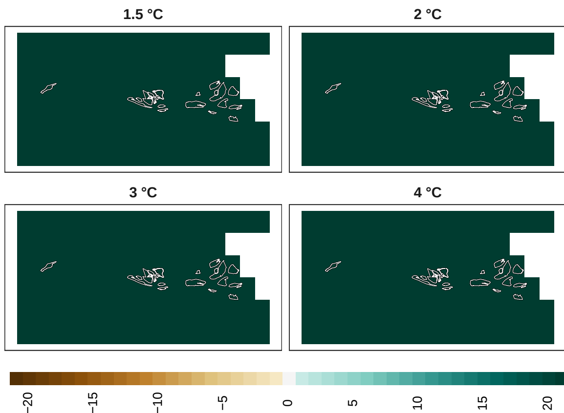
Figure 19: Adaptation effort for birds at 1 km resolution.
