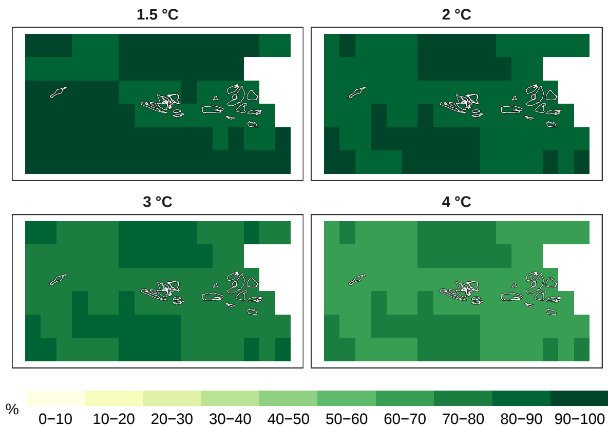
Figure 6: Percent insects remaining at 1 km resolution.
