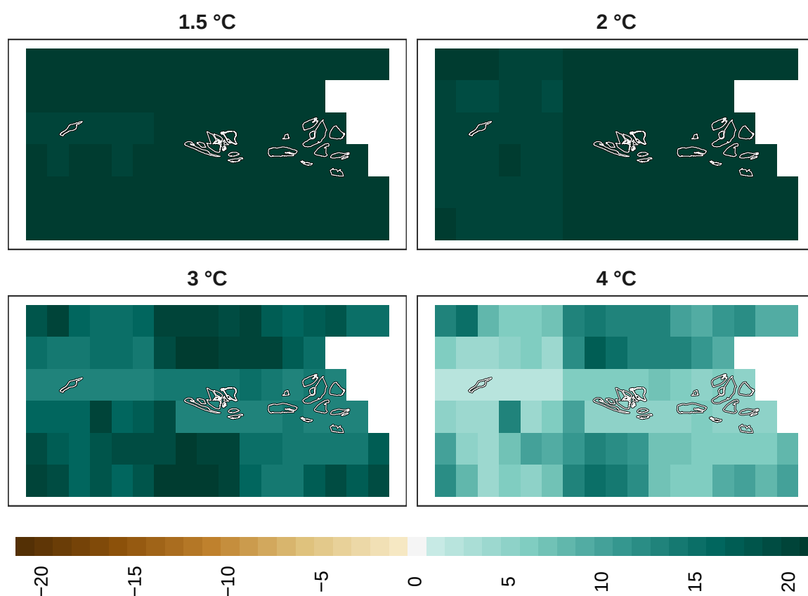
Figure 20: Adaptation effort for mammals at 1 km resolution.
