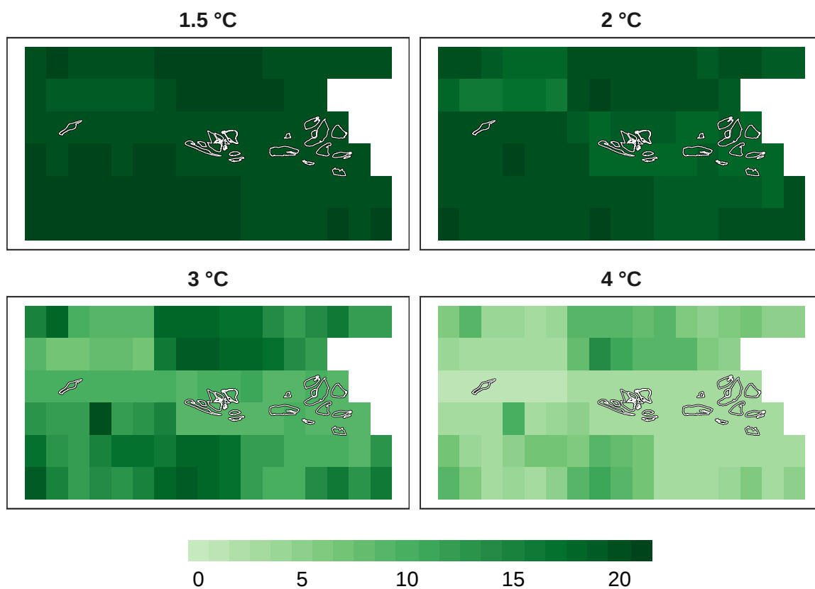
Figure 14: Number of models in agreement for insect refugia at 1 km resolution.
