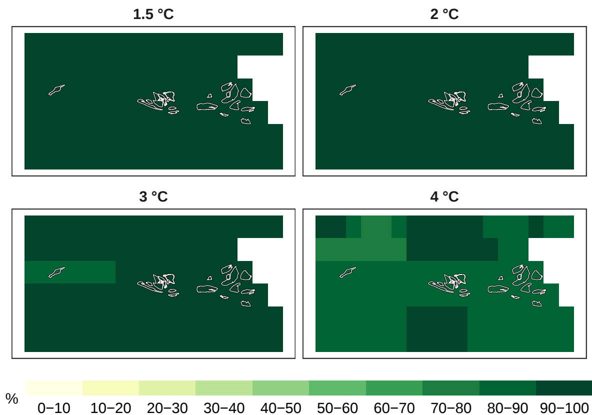
Figure 7: Percent pollinators remaining at 1 km resolution.
