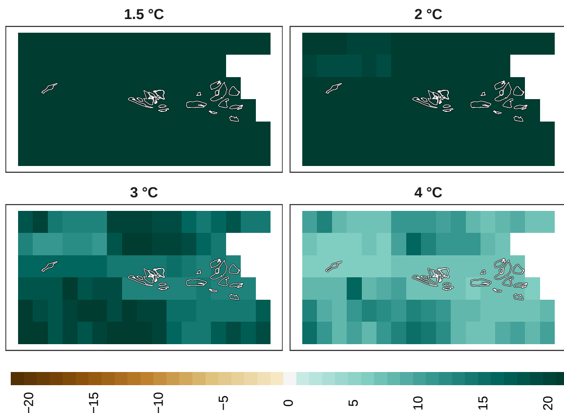
Figure 17: Adaptation effort for plants at 1 km resolution.
