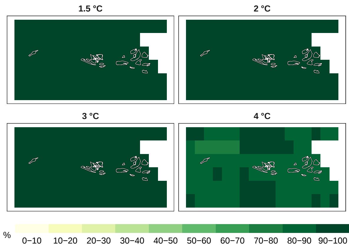
Figure 8: Percent timber species remaining at 1 km resolution.
