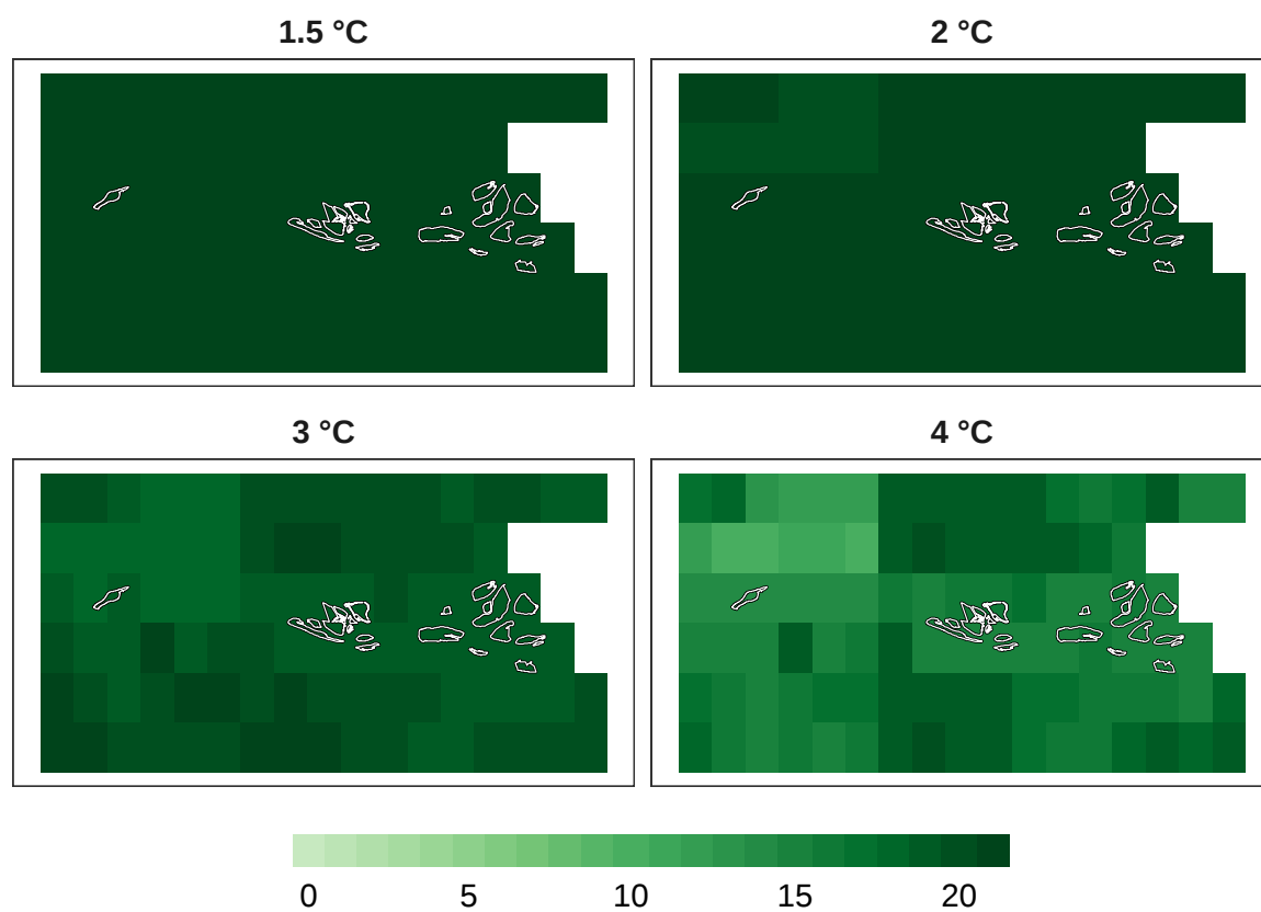
Figure 11: Number of models in agreement for amphibian refugia at 1 km resolution.
