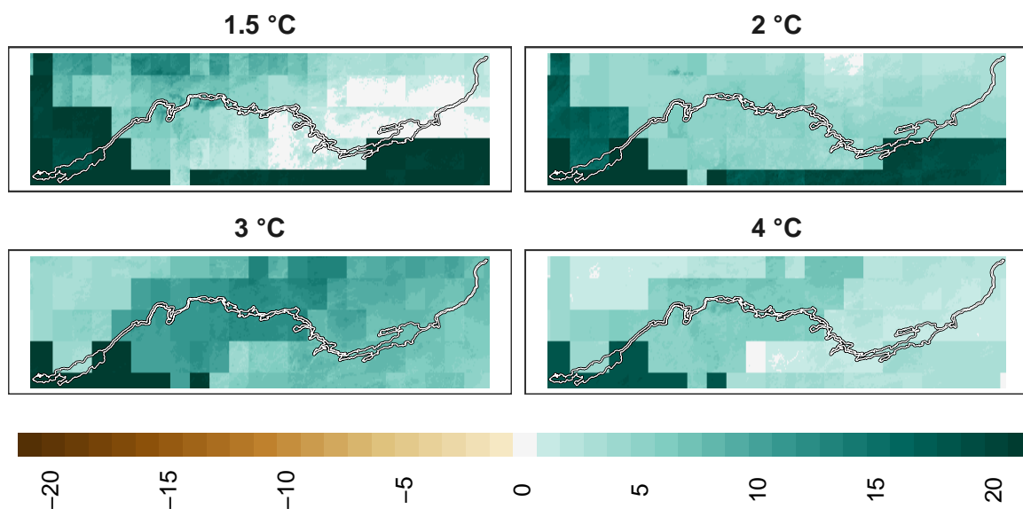
Figure 20: Adaptation effort for mammals at 1 km resolution.
