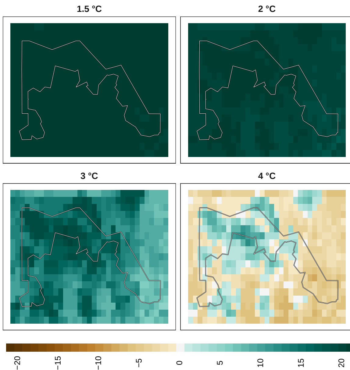
Figure 20: Adaptation effort for mammals at 1 km resolution.
