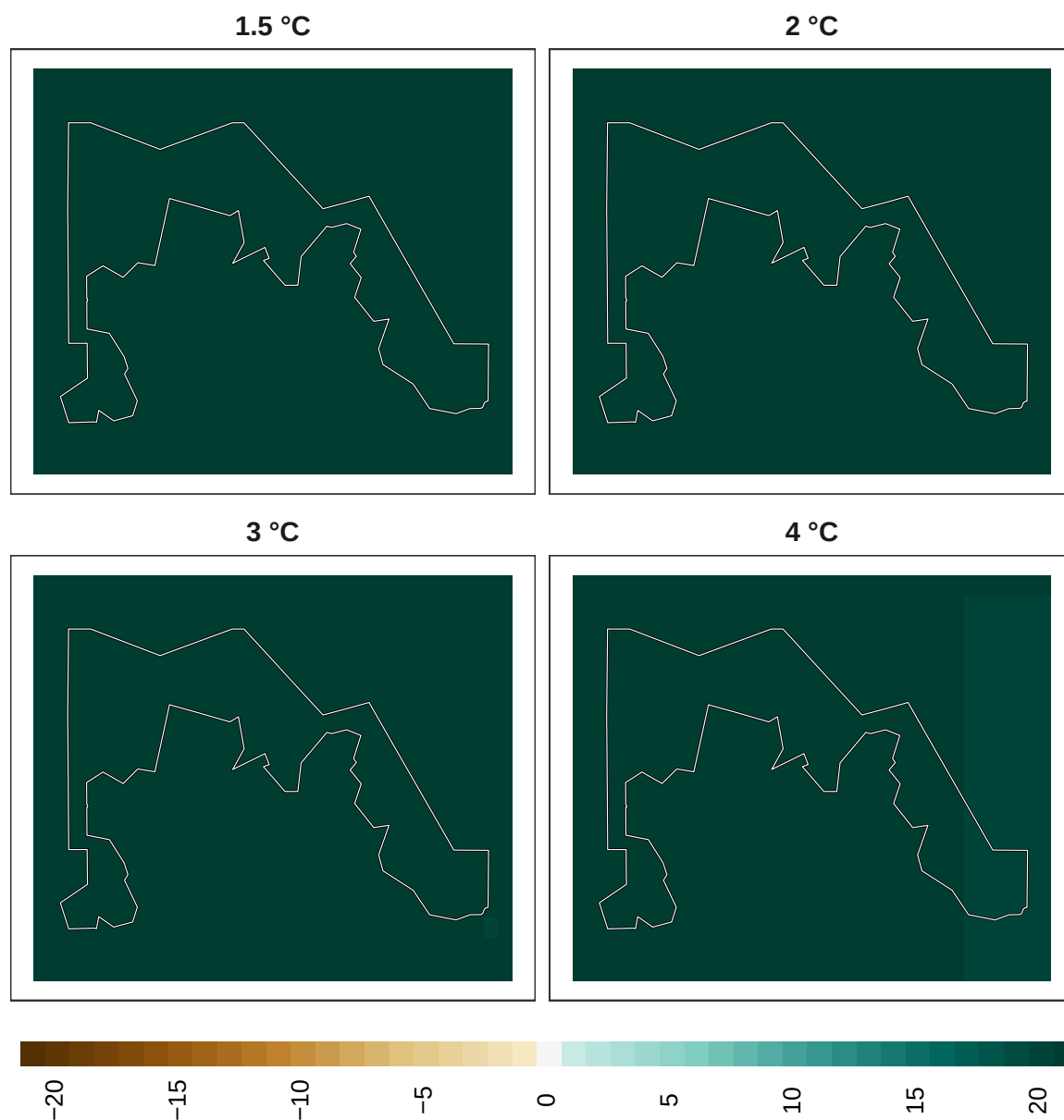
Figure 18: Adaptation effort for amphibians at 1 km resolution.
