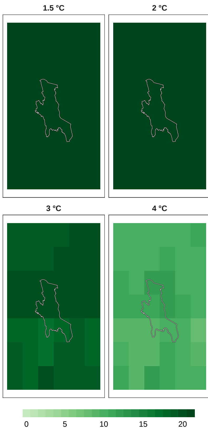
Figure 13: Number of models in agreement for mammal refugia at 1 km resolution.
