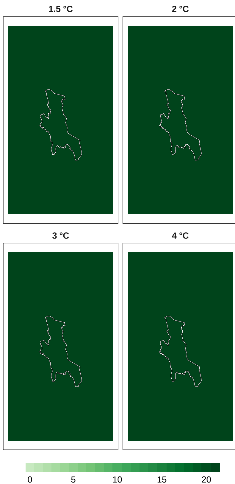
Figure 12: Number of models in agreement for bird refugia.
