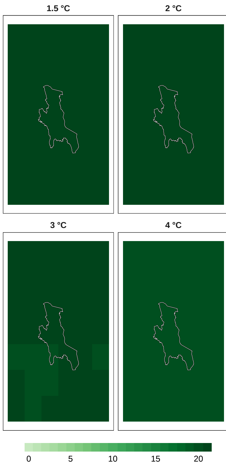
Figure 11: Number of models in agreement for amphibian refugia at 1 km resolution.
