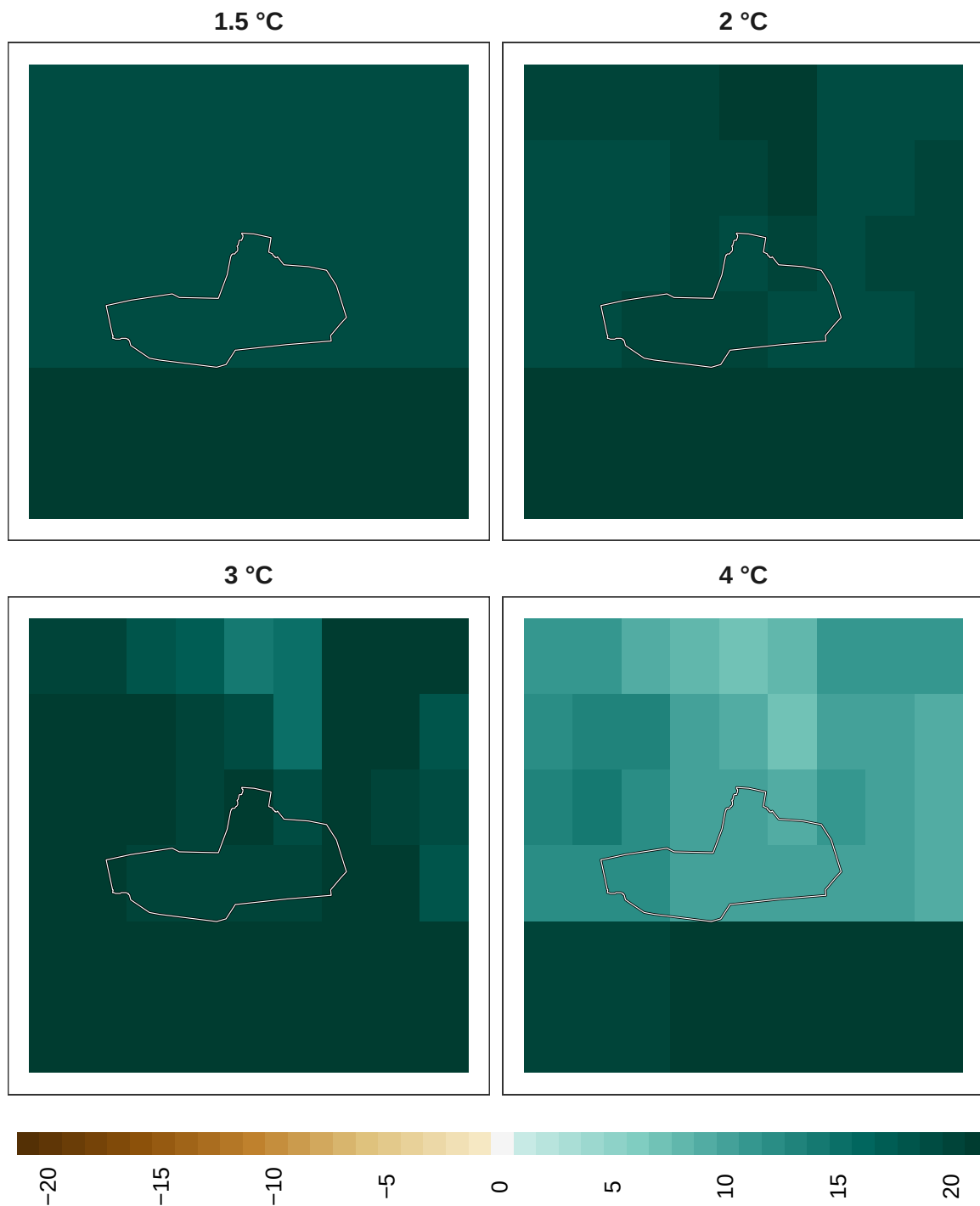
Figure 20: Adaptation effort for mammals at 1 km resolution.
