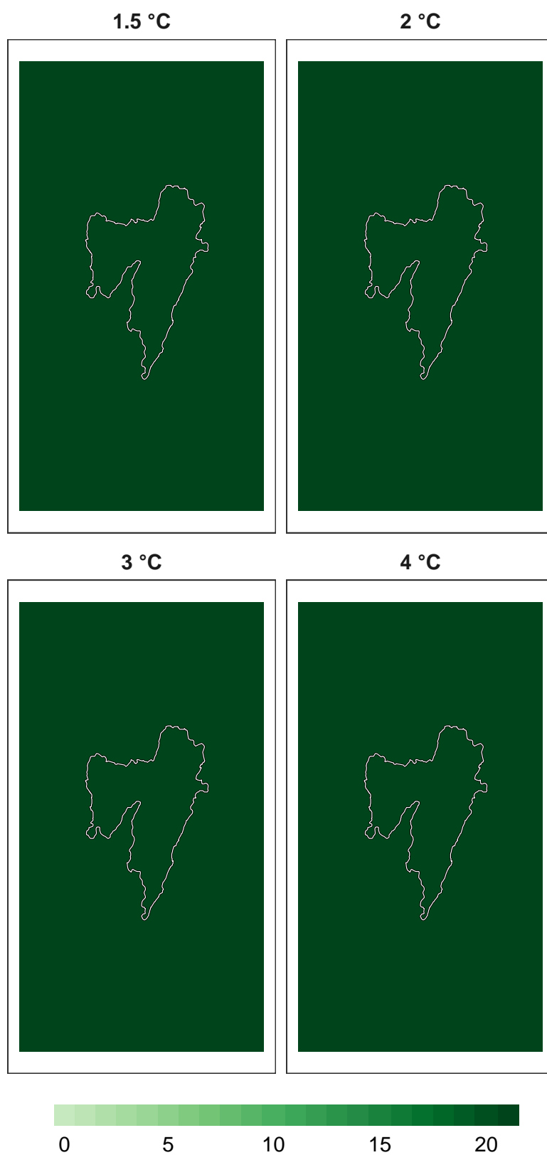
Figure 11: Number of models in agreement for pollinator refugia at 1 km resolution.
