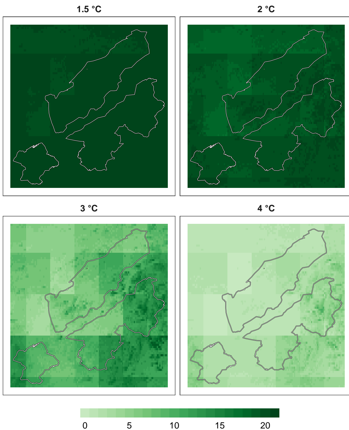
Figure 8: Number of models in agreement for insect refugia at 1 km resolution.
