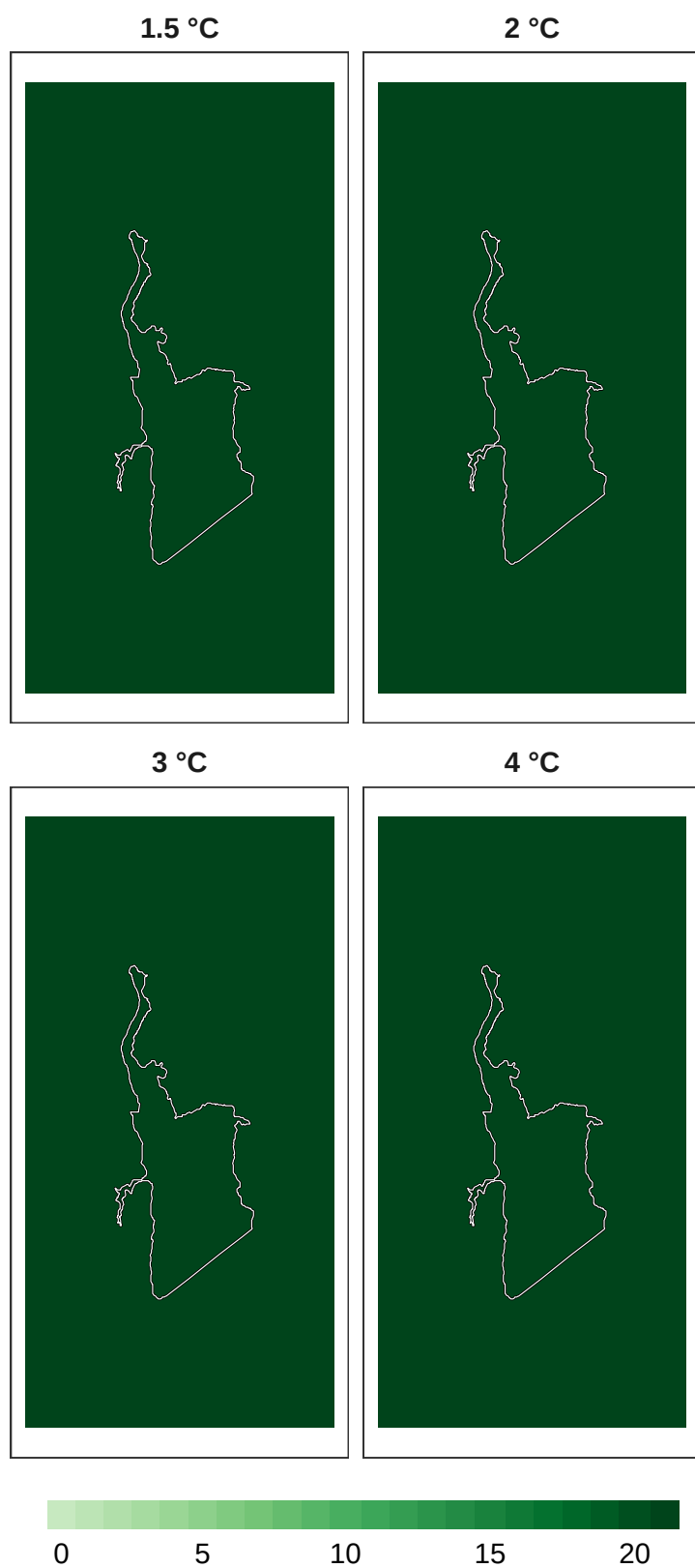
Figure 11: Number of models in agreement for amphibian refugia at 1 km resolution.
