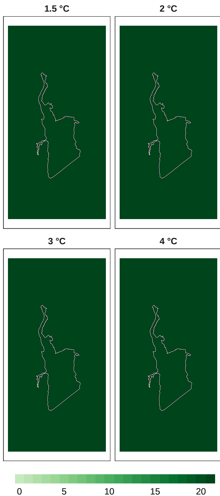
Figure 12: Number of models in agreement for bird refugia.
