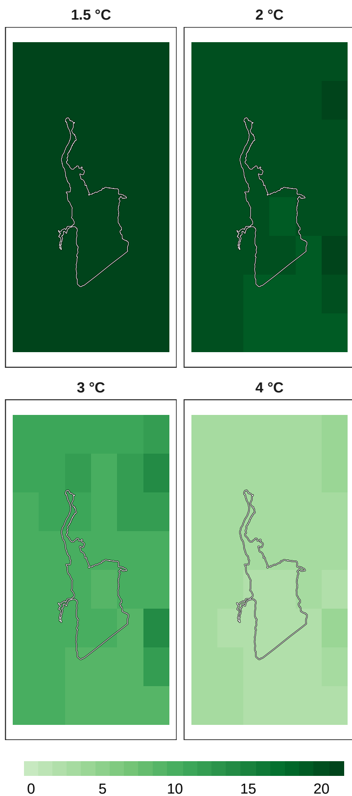
Figure 13: Number of models in agreement for mammal refugia at 1 km resolution.
