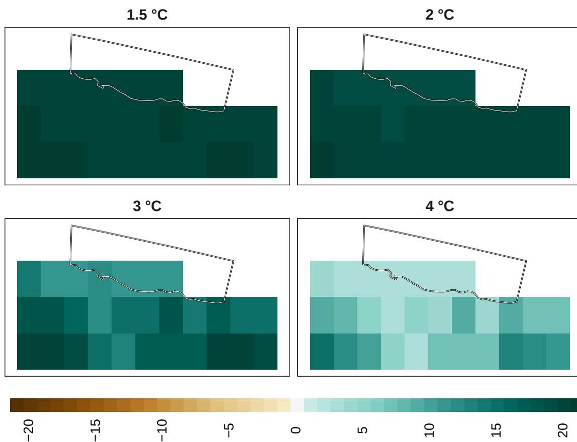
Figure 22: Adaptation effort for pollinators at 1 km resolution.
