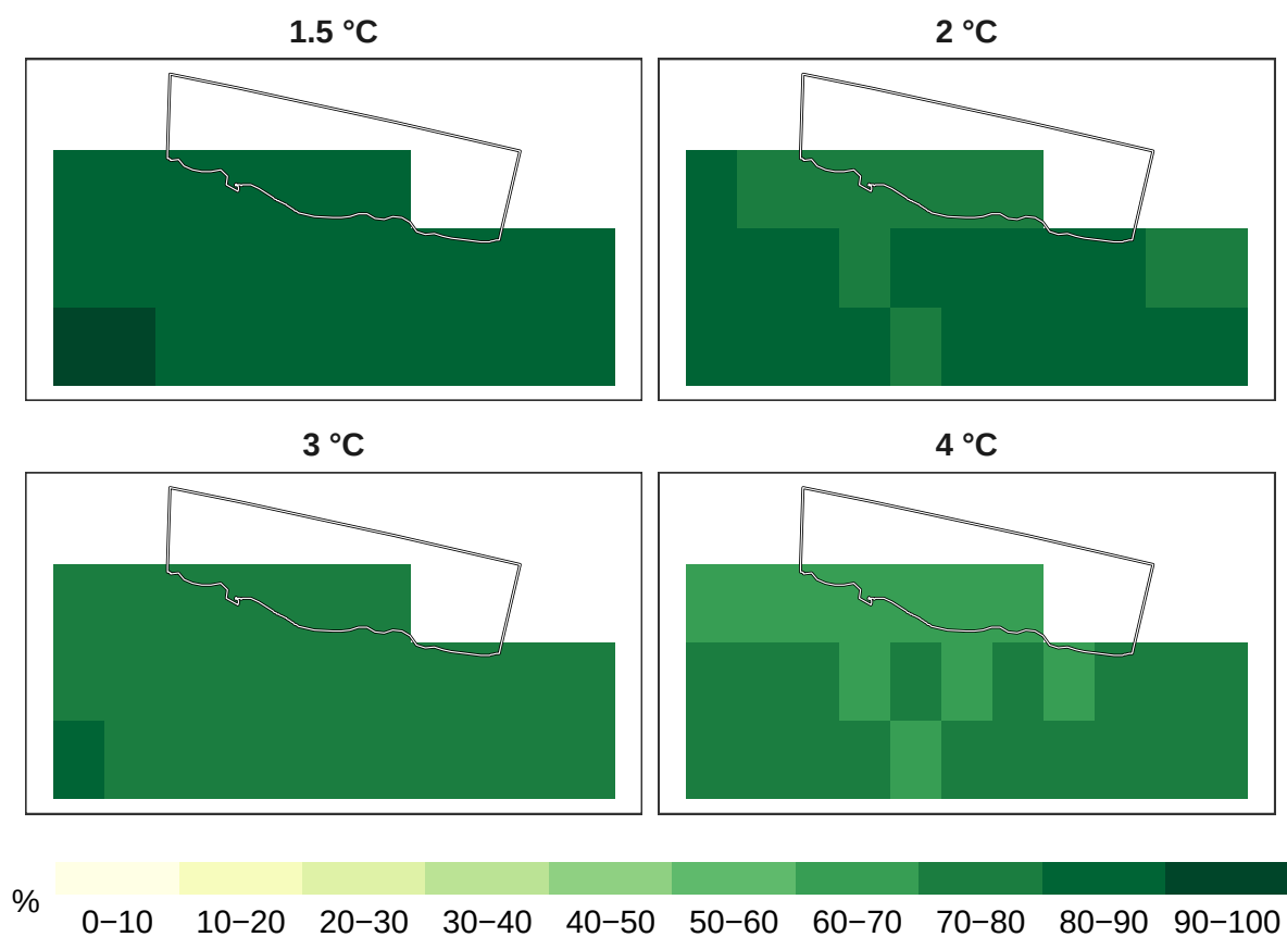
Figure 7: Percent pollinators remaining at 1 km resolution.
