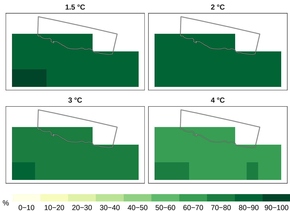
Figure 6: Percent insects remaining at 1 km resolution.
