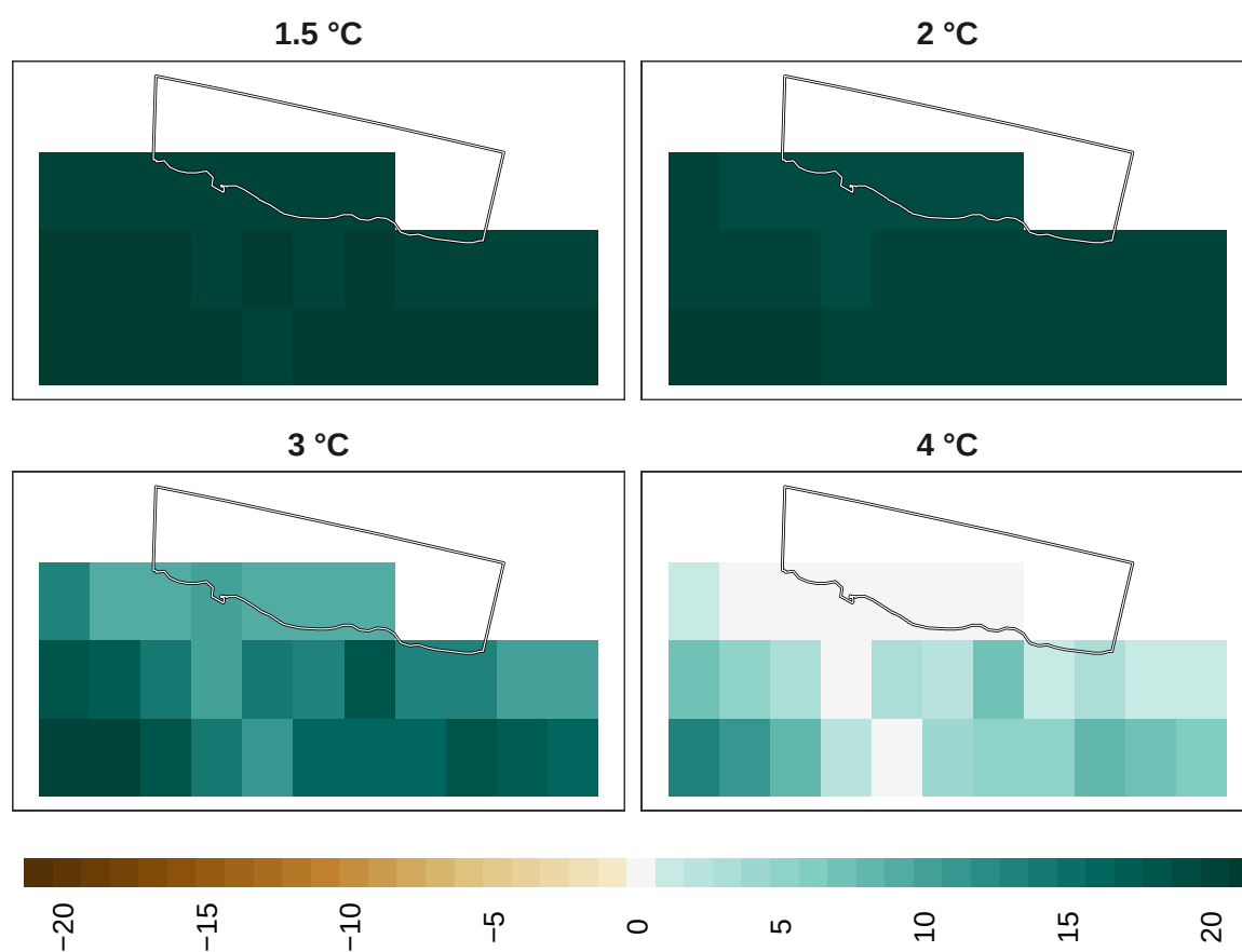
Figure 21: Adaptation effort for insects at 1 km resolution.
