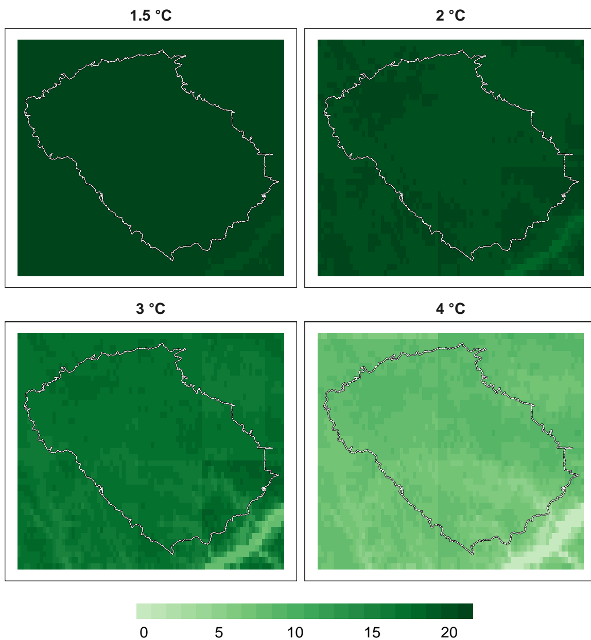
Figure 9: Number of models in agreement for insect refugia at 1 km resolution.
