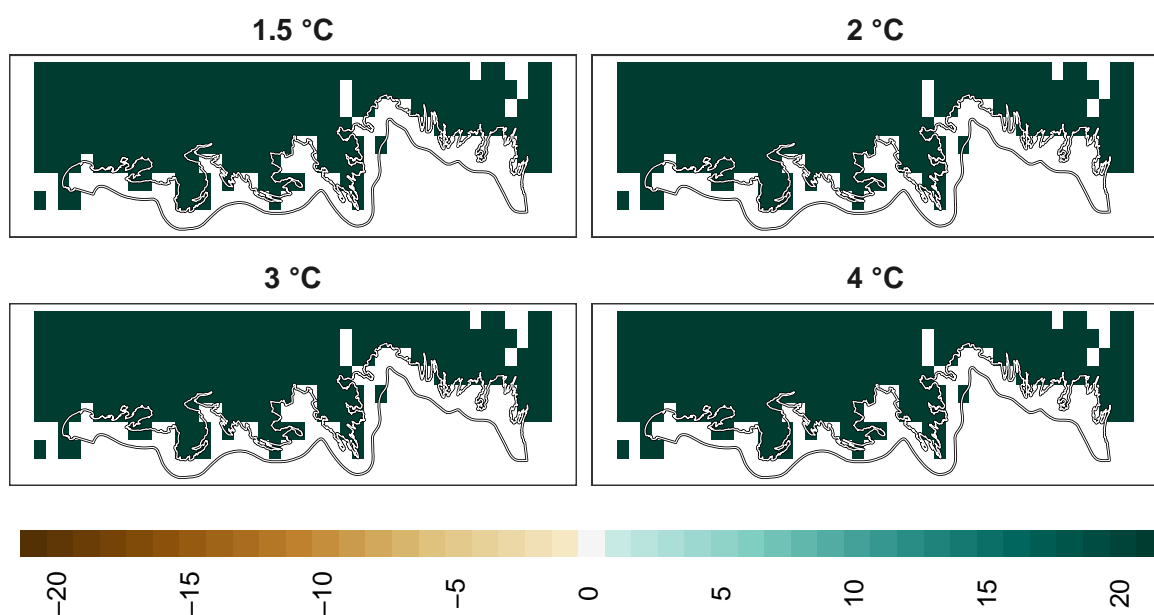
Figure 19: Adaptation effort for birds at 1 km resolution.
